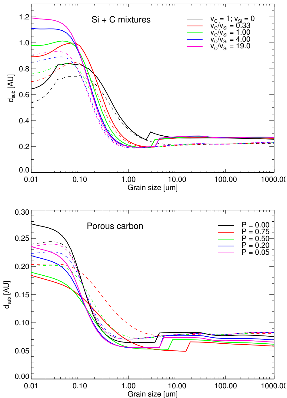
Figure 5.4: Sublimation distances of silicate ( top panel ) and carbonaceous material ( bottom panel ) in composite grains (C+Si or C+vacuum respectively) as a function of grain size in the Fomalhaut environment, with either a constant (dashed line) or a size-dependent (solid line) sublimation temperature. Relevant disk properties obtained from preliminary modeling are used (Sec. 5.4). Size-dependent sublimation temperatures are a function of the size-dependent survival timescales shown in Fig. 5.3 causing jumps at the material-dependent blowout limit.
