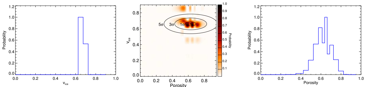
Figure 3.11: Bayesian probabilities for the grain composition in the case of 4-material dust mixtures.
