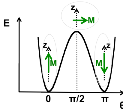
Fig. 2. 1 Schematic of the energy barrier in the case of a uni-axial system with no external applied magnetic field.
