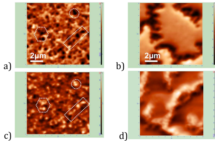
Fig. 5. 17 Comparison of magnetic states after applying +8\text{T} and -8\text{T} for high coercivity NdFeB film (a and c) and lower coercivity NdFeB film (b and d).
