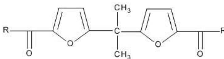
Figure 1.28: 2,2'-bis(5-chloroformyl-2-furyl)propane if R=Cl.
