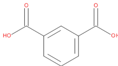
Figure 2.2: Isophthalic acid (benzene-1,3-dicarboxylic acid)
