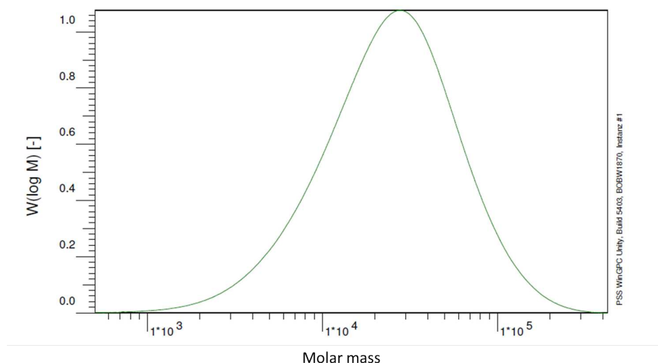
Figure 3.22: SEC spectrum of PA 6-I 90 /6-F 10 in HFIP, PMMA standards
