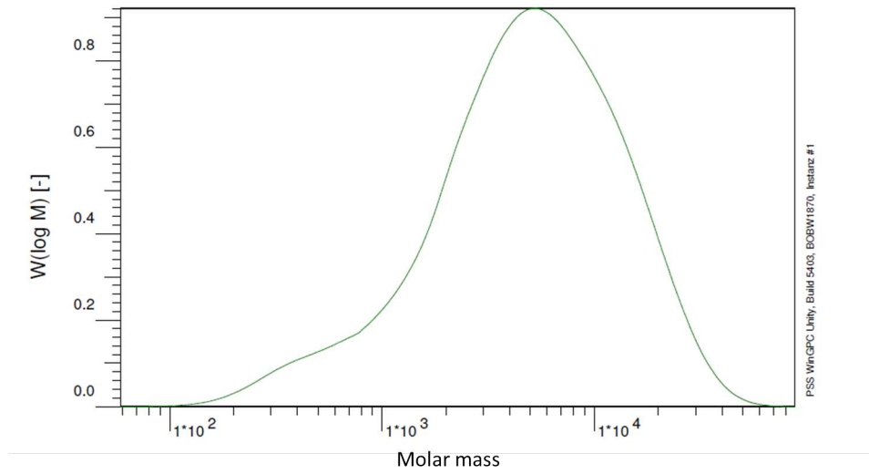
Figure 3.23: SEC spectrum of PA 6-F in HFIP, PMMA standards
