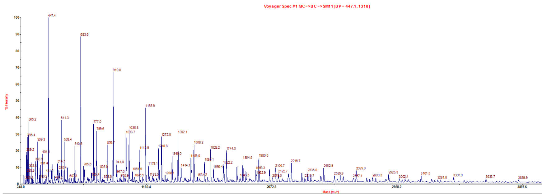
Figure 3.19: MALDI-TOF mass spectrum of PA 6-F (linear mode, dithranol matrix)
