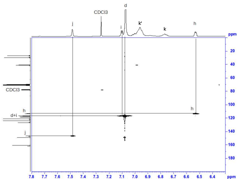
Figure 3.13: 2D Heteronuclear Single-Quantum Correlation Spectroscopy (HSQC) NMR spectra of PA 6-F in HFIP/ \text{CDCl}_3 (50/50).
