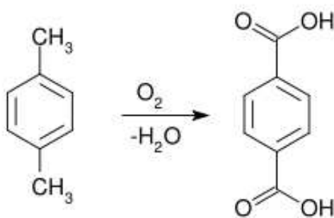
Figure 2.3: Oxidation of p-xylene by O_2 in the air
