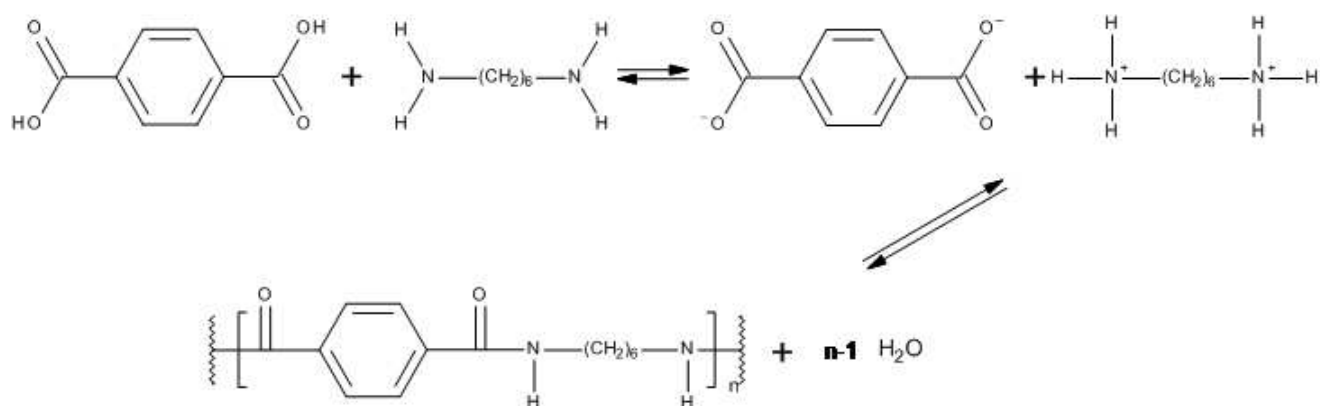
Figure 2.6: Polycondensation reaction scheme PA 6-T
