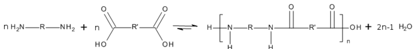
Figure 1.2: Synthesis of a polyamide starting from a diamine and a diacid (AABB).
