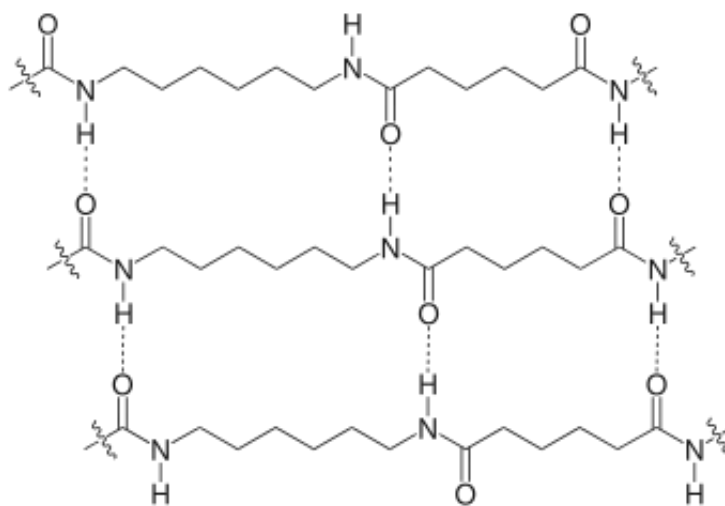
Figure 1.12: Polyamide 6-6 structure
