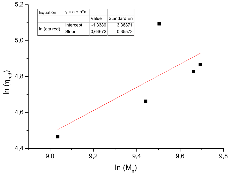
Figure 2.18: Reduced viscosity as a function of \bar{M}_n (by SEC)
