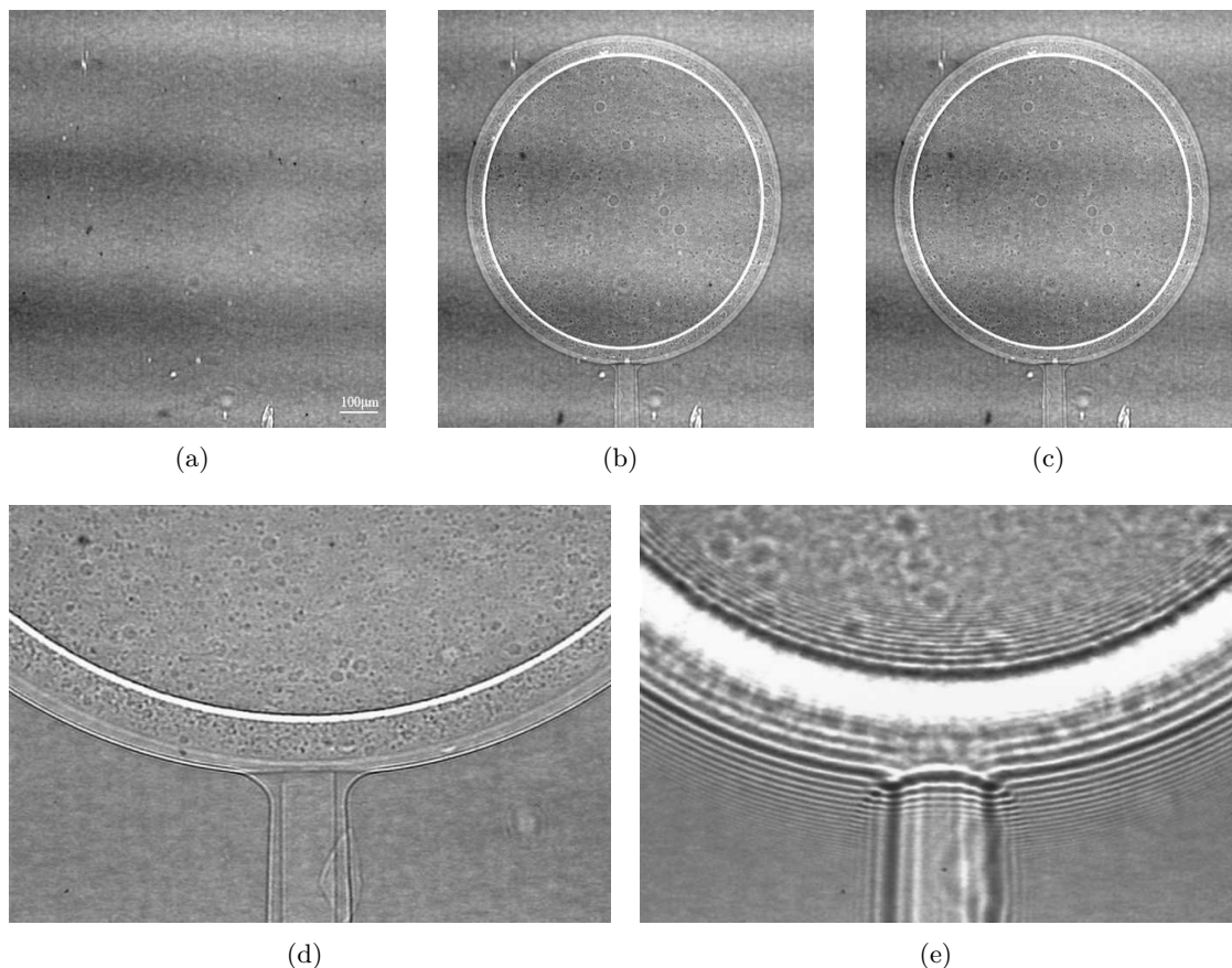
Figure 1.1: X-ray phase contrast images for a two-layered sphere sample. A 30\ \mu\text{m} layer of polystyrene covered by a 15\ \mu\text{m} layer parylene for (a) D = 0.3\ \text{cm} , (b) D = 19\ \text{cm} and (c) D = 83\ \text{cm} . Data acquisition have been performed at ESRF for E=18\text{keV} . Image details for (d) D = 15\ \text{cm} and (e) D = 310\ \text{cm} . Reproduced from [Cloetens et al. (1999)].
