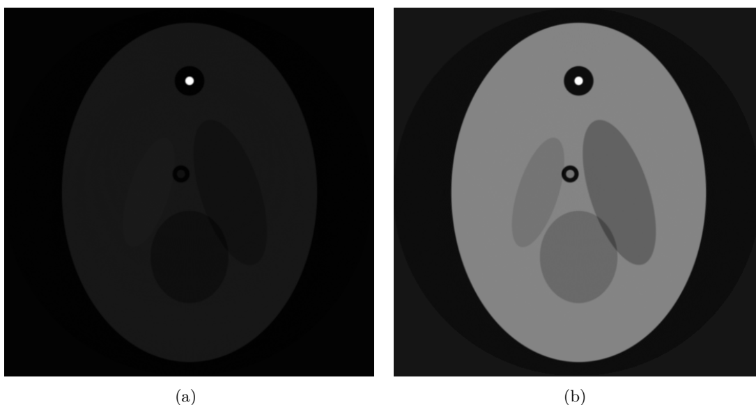
Figure 9.6: Central slice of the 3D Shepp-Logan phantom used in the simulations. (a) Absorption index \beta ( D = 0 m) and (b) refractive index decrement \delta_r .
