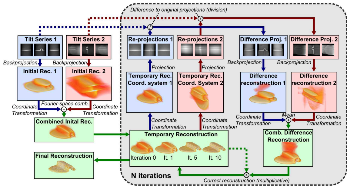
Figure 9.6: Principle of the proposed combined dual-axis SIRT reconstruction algorithm.
