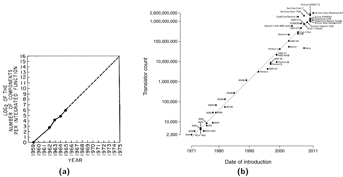
Figure 2.1: Moore's law: (a) Graph originally published by Gordon Moore in 1965 (Moore, 1965) (b) Extrapolation until 2011 showing important microprocessors (Wikipedia, 2013).
