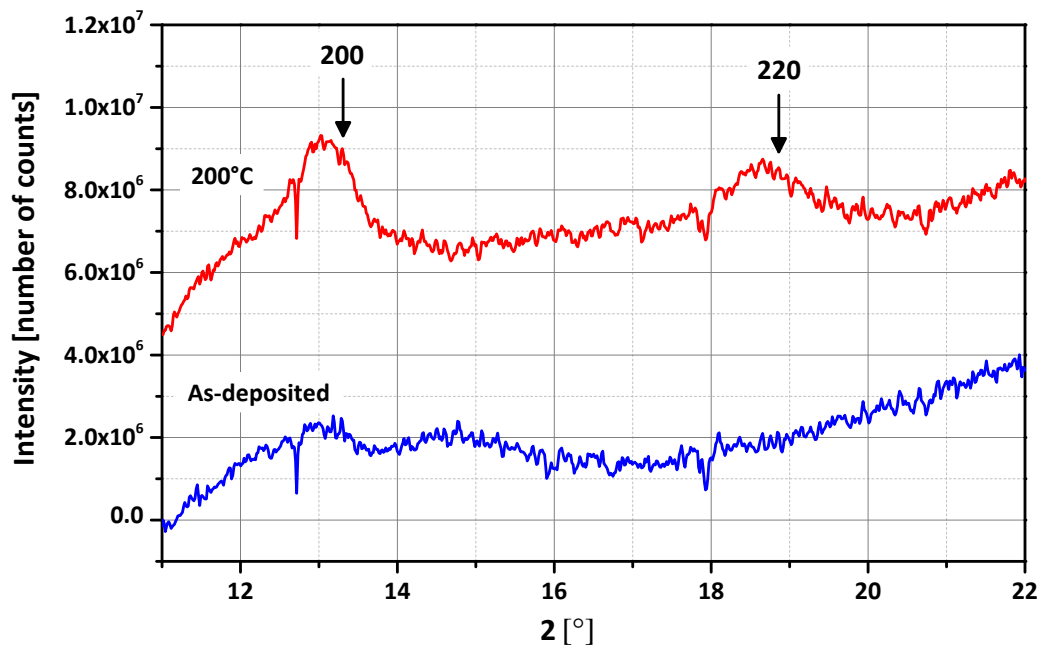
Figure 3.13: X-ray diffraction spectra at room temperature for as-deposited and 200°C ex situ annealed GST clusters after background subtraction. Curves are shifted for clarity. Arrows indicate bulk GST fcc peak positions calculated assuming the lattice parameter of GST a=6.0117 \text{ \AA} reported in Ref.[25].
