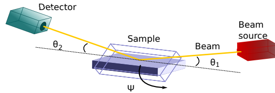
Figure 4.5: Schematic representation of the experimental geometry of the XRD experiment, where \theta is the incident beam angle and \Psi is the tilting angle of the sample. A detailed description of the experimental setup is provided in appendix A.2.1
