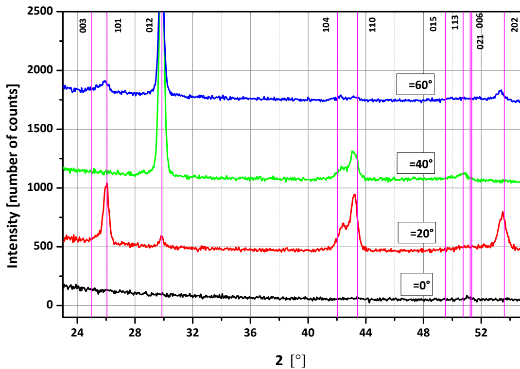
Figure 4.13: Diffracted intensity as a function of 2\theta for the GeTe 100 nm thin film interfaced with \text{SiO}_2 , measured at 100°C after annealing at 300°C (heating rate around 0.11°C/min) for various tilting angles \Psi . The intensity of the 012 Bragg peak is maximum at around \Psi = 40^\circ , as already reported in Fig.4.7, while the 101, 202, 104 and 110 peaks exhibit the highest intensity for \Psi = 20^\circ .
