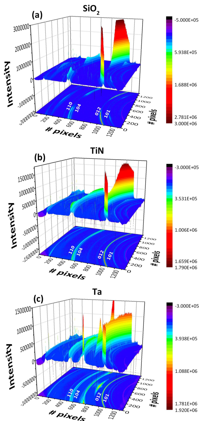
Figure 4.12: 3D images of the diffracted rings obtained for GeTe 100 nm thin films annealed at 400°C for 15 minutes and interfaced with (a) SiO 2 (b) TiN (c) Ta. The SiO 2 interfaced film is strongly textured while only a faint texture is visible for the TiN interfaced film and the GeTe rings are isotropic for the Ta interfaced film. The strongly textured rings that can be seen in (c) correspond to Ta.
