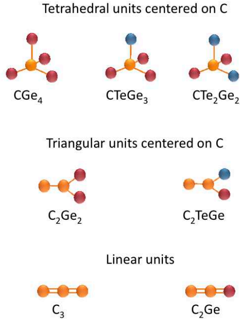
Figure 2.12: Summary of the carbon environments in the C-doped GeTe sample. C-TeGe_3 , C-Ge_4 and C-Ge_2Te_2 tetrahedra can be found, as well as C-C-Ge_2 and C-C-GeTe triangular environments.
