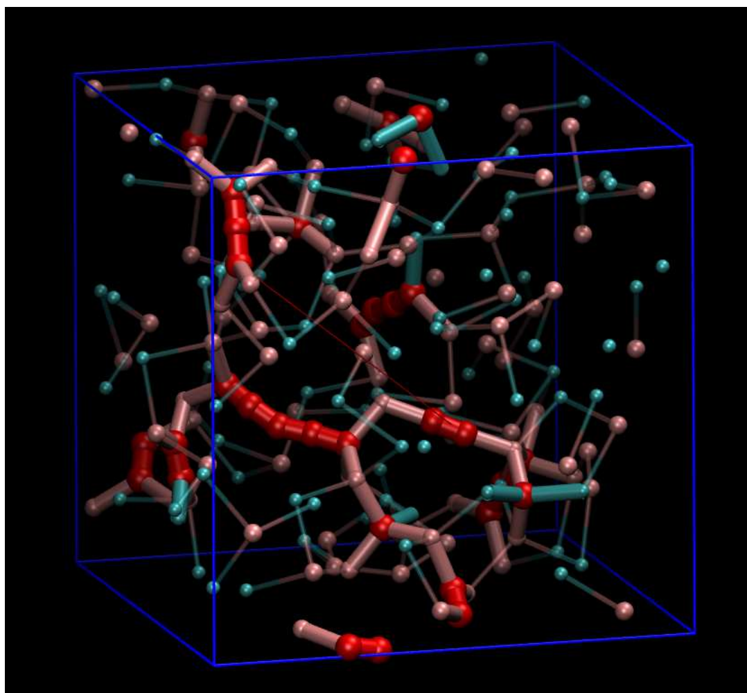
Figure 2.11: Snapshot of the final state of the simulation box for GeTeC. Ge atoms are represented in pink, Te atoms in light blue and C atoms in red. The inspection of this box combined with a bond angle analysis around C atoms, reveals the presence of a mixture of tetrahedral ( C-TeGe_3 , C-Ge_4 and C-Ge_2Te_2 ), triangular ( C-C-Ge_2 and C-C-GeTe ), and linear (C chains) bonds.
