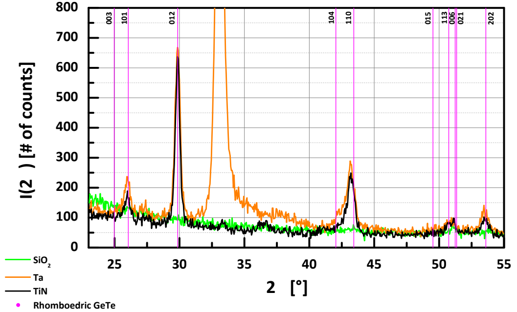
Figure 4.6: Diffracted intensity as a function of 2\theta for \Psi = 0^\circ of GeTe 100 nm thin films sandwiched between TiN, Ta or SiO 2 measured at 100°C after annealing at 300°C with a heating rate of about 0.11°C /min. The vertical lines correspond to the calculated position of Bragg peaks for rhombohedral GeTe (hexagonal indexation) [25]. No difference in the diffraction spectra can be observed between the Ta and TiN interfaced samples, while no peaks are visible for the sample sandwiched in SiO 2 . The intense peak around 33° is due to Ta.
