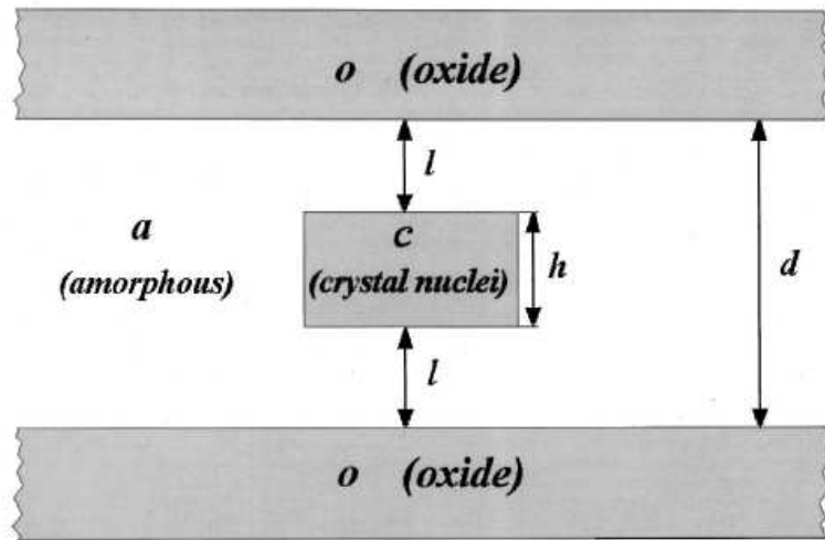
Figure 3.2: Model used Ref.[71] to interpret the thickness-dependent variation of T_x . A cylindrical crystalline nucleus is embedded in the amorphous phase, sandwiched between two oxide interfaces.
