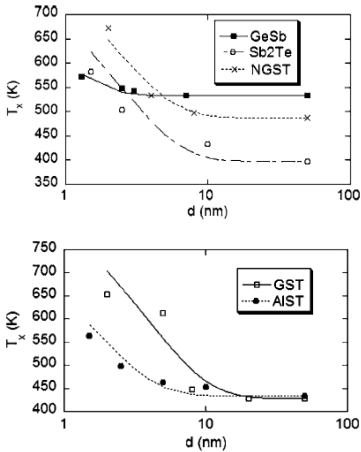
Figure 3.3: Crystallization temperature T_x as a function of film thickness for various PC materials: GST, N-doped GST (NGST), \text{Ge}_{15}\text{Sb}_{85} (GeSb), \text{Sb}_2\text{Te} and Ag- and In-doped \text{Sb}_2\text{Te} (AIST) deposited on Si and capped with \text{Al}_2\text{O}_3 , fitted using Eq.3.1, as presented in Ref.[70].
