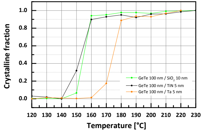
Figure 4.9: Evolution of the crystalline fraction as a function of temperature (heating rate of about 0.11^{\circ}\text{C}/\text{min} ) for the 100nm thick GeTe films interfaced with \text{SiO}_2 , TiN and Ta as obtained from the 012 GeTe Bragg peak area measured by XRD through in situ annealing for a tilting angle \Psi=40^{\circ} .
