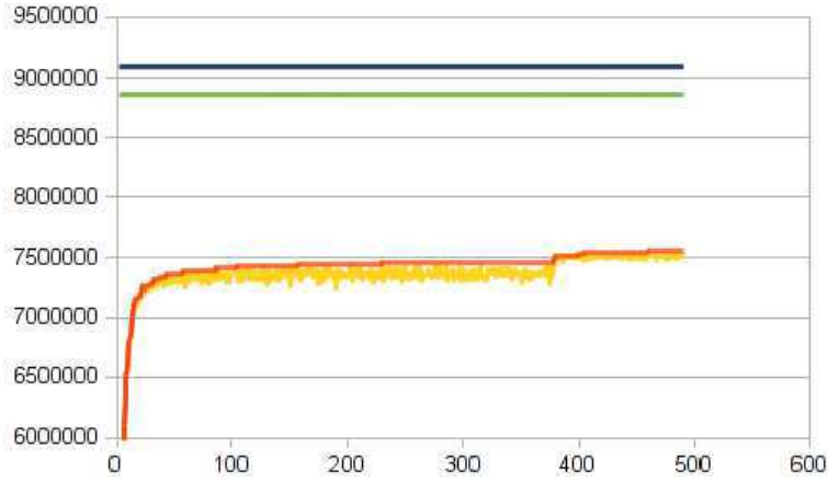
Figure 3.2: Convergence of the Lagrangian Relaxation (225 legs)
