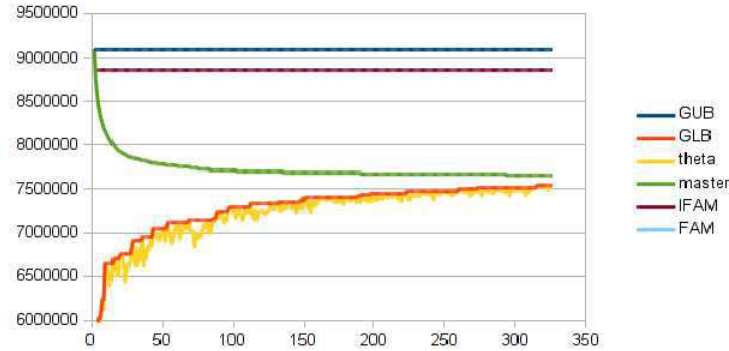
Figure 3.4: Dantzig-Wolfe Decomposition Relaxation Convergence (225 legs) (FAM and GUB are the same line: the solution is not improved)
