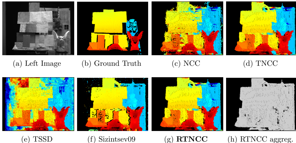
Figure 2.5: York University dataset of Sizintsev & Wildes (2009) , frame 8. Disparity maps are fairly similar since the scene moves really slowly and the disparity does not change much over time. Almost the entire scene is matched by the temporally aggregated statistic, see (h).
