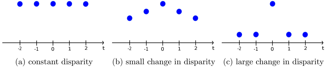
Figure 2.2: Distributions of per-frame correlations over time. The match is correct at time t = 0 . (a) If disparity is constant over time, all per-frame correlations are high. (b) When there is a small temporal change in disparity, all per-frame correlations around the central one ( t = 0 ) have a lower value. (c) When there is a large change in disparity, the correlations around the central frame tend close to zero.
