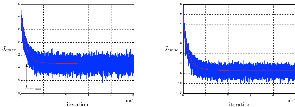
FIGURE 2.6 – Convergence of J_{MSE}(n) with step size \eta = 10^{-3} , in the case where input x(n) is i.i.d. on the left figure, and generated by a first-order AR process on the right figure. Compared to Figure 2.4 (left) and 2.5 (left), the variance of the noise z(n) has been increased from 10^{-2} to 1.
