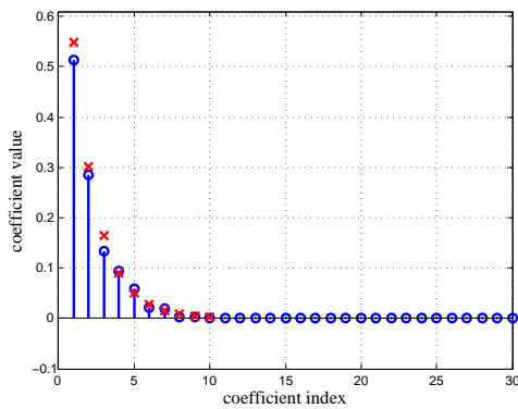
(c) Normalized NNLM algorithm.
