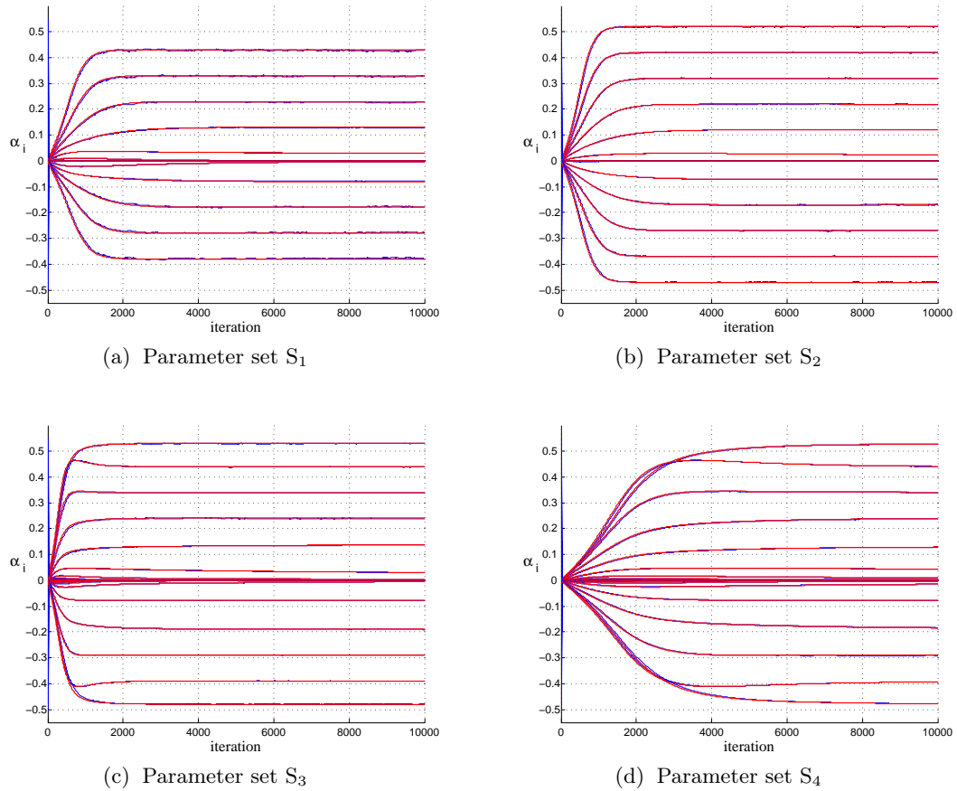
FIGURE 3.3 – Evolution of the coefficients \alpha_i(n) for the NNLMs-based \ell_1 -regularized algorithm with different parameter settings.
