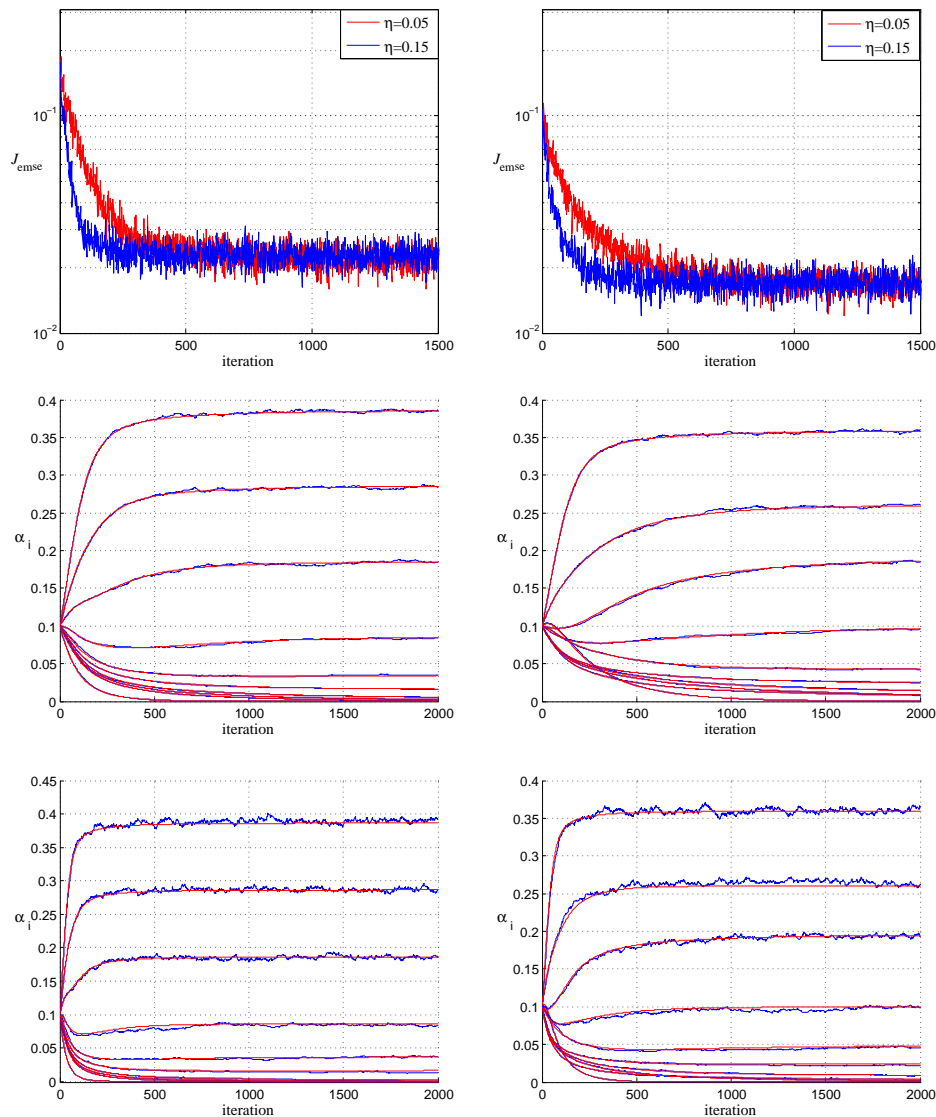
FIGURE 3.1 – First column : algorithm behavior with white input. Second column : algorithm behavior with correlated input. From top to bottom : EMSE convergence curves, weight behavior with \eta = 0.05 , weight behavior with \eta = 0.15 . The red curves for weight behavior are analytical results obtained with the model described in [Chen 2011]
