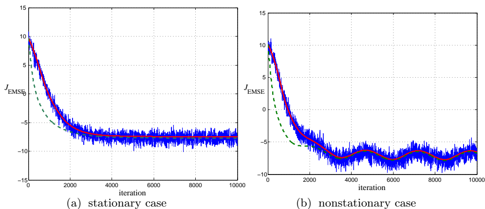
FIGURE 2.13 – Evolution of the EMSE for the Sign-Sign NNLMS algorithm in stationary and nonstationary environment. Theoretical evolution of original NNLMS is represented by the green dashed line.
