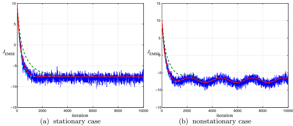
FIGURE 2.12 – Evolution of the EMSE for the Exponential NNLMS algorithm in stationary and nonstationary environment. Light blue dash-dot line and green dashed line show the theoretical results for (p, q) = (3, 5) and (p, q) = (1, 1) (original NNLMS), respectively.
