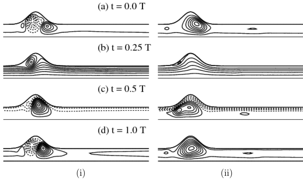
Figure 4.24: Streamlines at different time instants in a pulse cycle. Parameter settings: Q1 , Re = 264 , H = 0.5 , W = 0.5 (i) Wo = 10 (ii) Wo = 15 .
