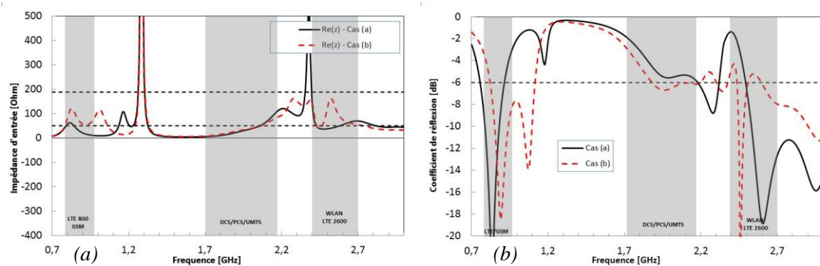
Figure IV-17 : Config 3 - (a) Re(z) , (b) S_{11} de l'antenne IFLA-AC
