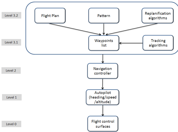
Figure 5. Level based decomposition of the controller
