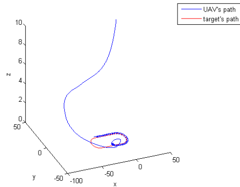
Figure 12. LaSalle's principle based tracking results in 3D
