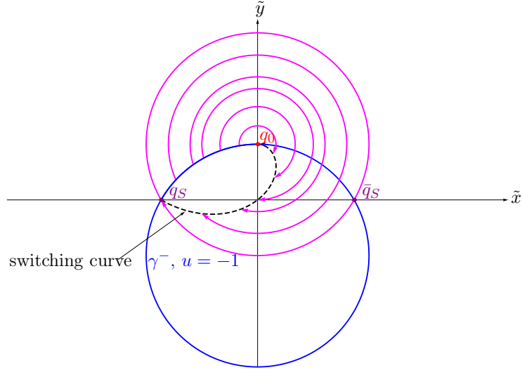
Figure 8: Switching curve family 1
