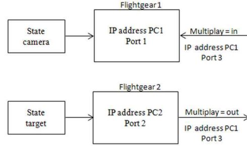
Figure 2. Flightgear configuration
