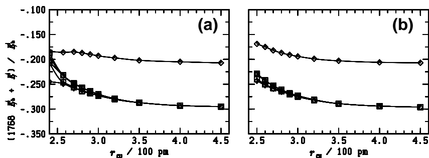
FIGURE 4.4: (22, 13) CAS - potential energy functions V(r_{\text{Cu}}) for the lowest linear singlet states of A' symmetry ( = A_1 \oplus B_1 ) at r_{\text{NO}} = 115 pm, \theta_{\text{Cu}} = 180^\circ (panel (a), Cu-N-O configuration) and \theta_{\text{Cu}} = 0^\circ (panel (b), N-O-Cu configuration). Lines are cubic spline interpolations and give MCSCF electronic energies E as numerical function 1768 + E/E_h of the copper distance r_{\text{Cu}} .
