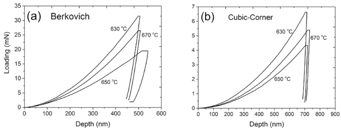
Figure 7-6 The obtained typical depth-penetrating curves of the steel studied by using (a) Berkovich indenter, and (b) Cubic-Corner indenter.
