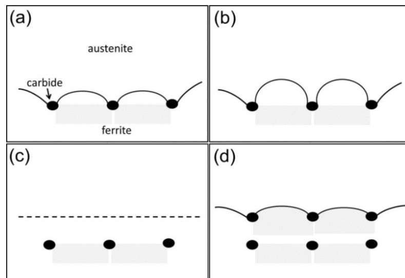
Figure 2-5 The bowing mechanism for the curved interphase-precipitated carbides with irregular spacing [34]
