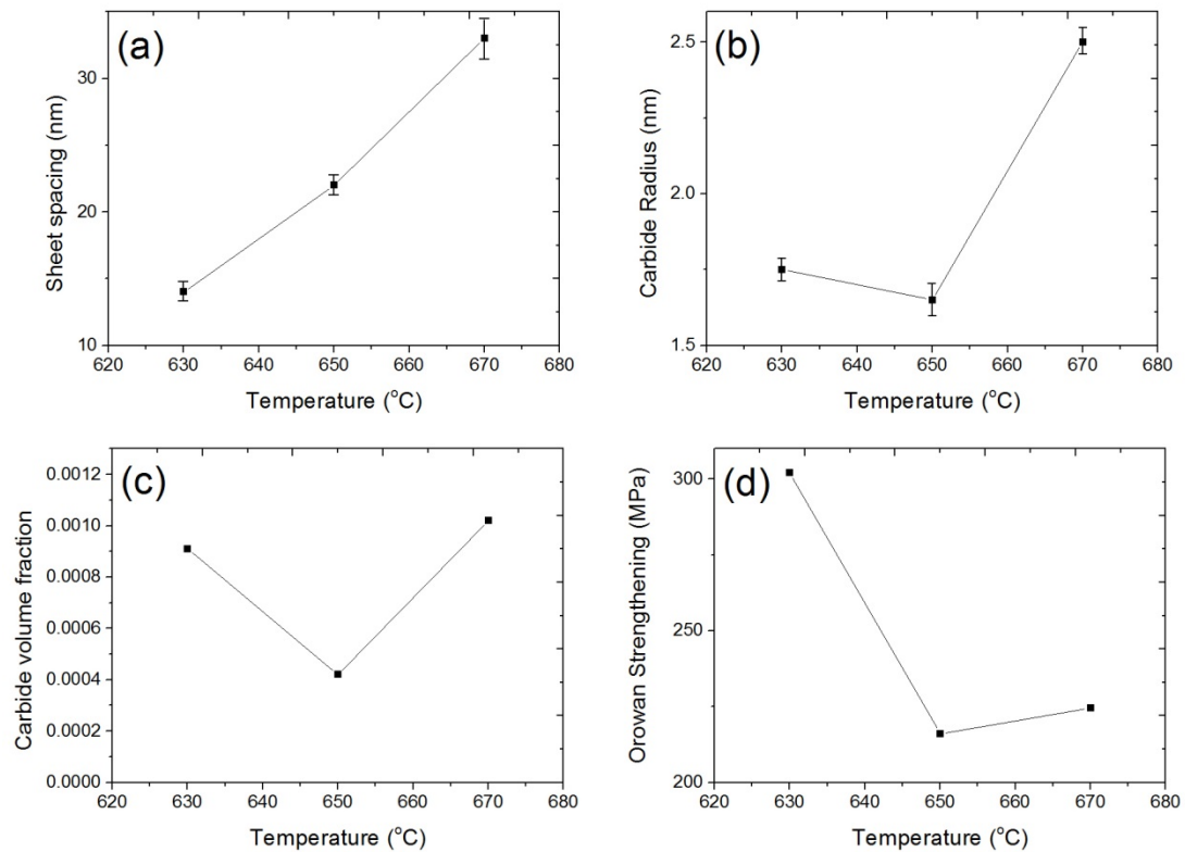
Figure 7-9 The temperature-dependence of (a) sheet spacing, (b) carbide radius, (c) carbide volume fraction, and (d) theoretical Orowan strengthening with transformation temperatures.
