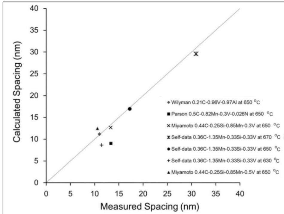
Figure 5-3 Coupling with experimental data to the calculated sheet spacing showing that good agreements with the sheet spacing measured at lower transformation temperatures ( < 700^{\circ}\text{C} ). The experimental data is cited from Wilyman [92], Parson [52], and Miyamoto [74]
