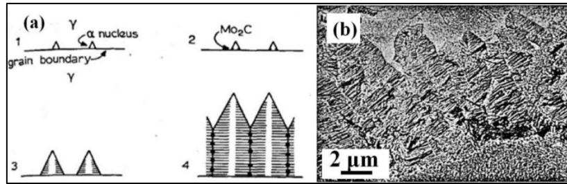
Figure 2-19 Model illustrating the \text{Mo}_2\text{C} carbides formed in spiky noduls. Fe-4.10Mo-0.23C (wt%) isothermal transformation at 650 oC for 2 hours [46]
