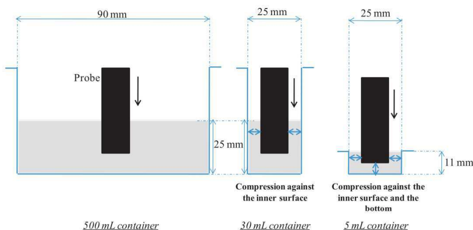
Fig. 1. Diagrams of the different containers used for penetration tests, showing side effects of product's compression against inner surface and bottom of the containers.
