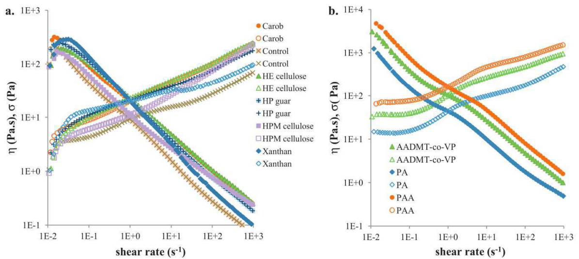
Fig. 3. Flow characterization of the 9 O/W emulsions. Each curve presents the mean values over three tests. The standard deviations remain lower than 5%, and are not shown for a better readability. Solid symbols: viscosity, \eta ; hollow symbols: shear stress, \sigma . Part (a) corresponds to the emulsions containing a polysaccharide and the control one; part (b) corresponds to the emulsions containing a synthetic polymer.
