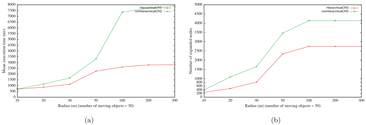
Figure 7.2: Varying the radius: Hierarchical vs. non-Hierarchical Continuous Range Search
