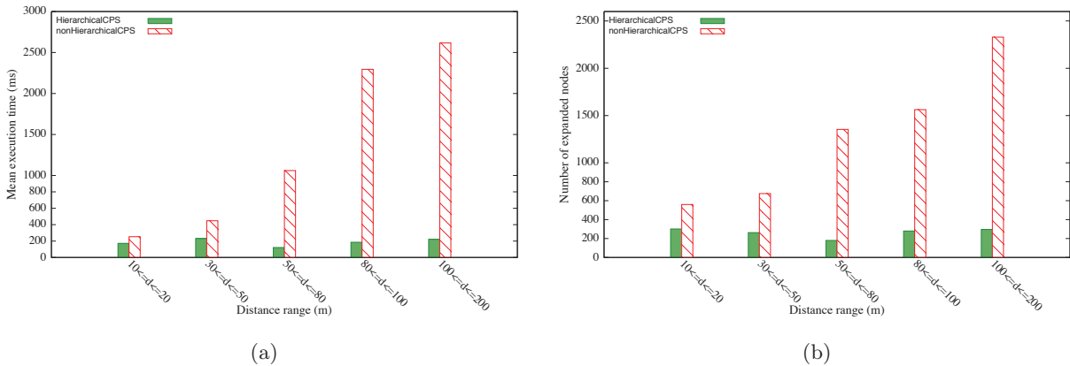
Figure 7.1: Varying the distance parameter: Hierarchical vs. non-Hierarchical Continuous Path Search
