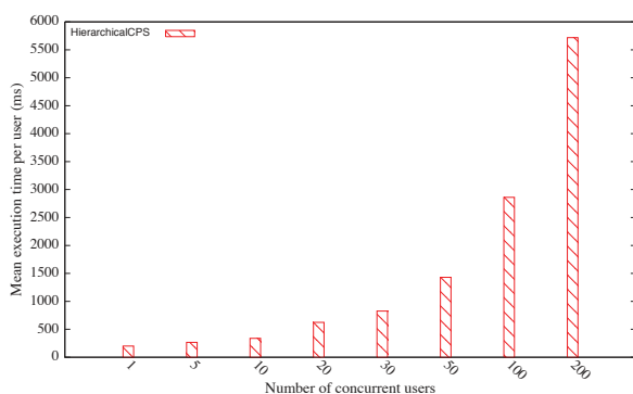
Figure 7.4: Varying the number of concurrent access: Hierarchical Continuous Path Search
