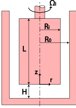
Figure 1.13: Schematic of a concentric cylinder rheometer.
