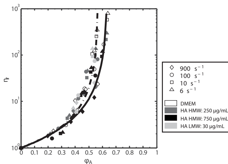
Figure 6.9: Relative viscosity as a function of the effective volume fraction for different HA concentrations and molecular weight and for different shear rates. The solid line is the Krieger and Dougherty model with \varphi_0 = 0.64 , the broken line is the Krieger and Dougherty model with \varphi_0 = 0.57 .
