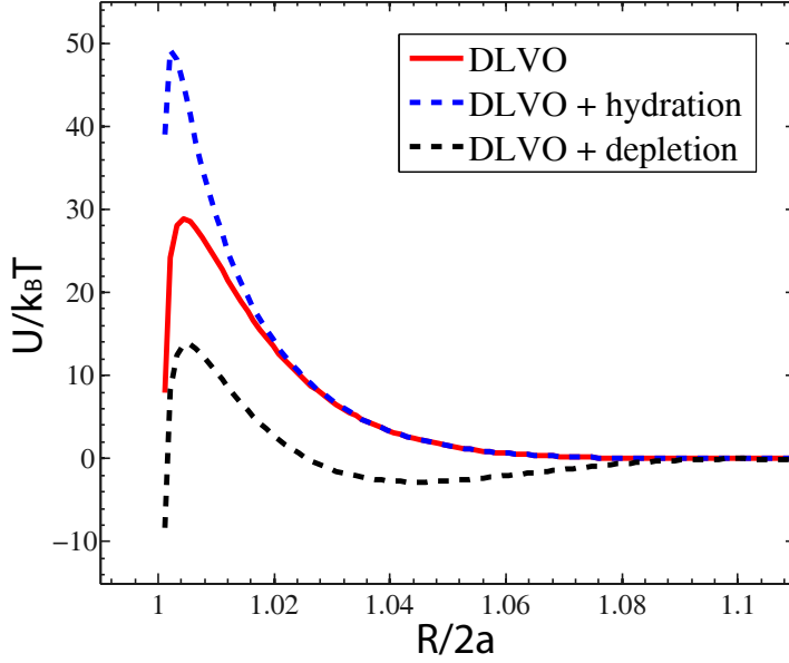
Figure 2.16: Interaction potential for DLVO, hydration and depletion interactions. Data for numerical calculations are: Eq (2.22), A_{pmp} = 4 \times 10^{-21} J; Eq (2.23b), a = 100 nm, \Phi_0 = 25 mV, \kappa a = 35 , \epsilon = 7.08 \times 10^{-10} C 2 /Nm 2 , T = 293 K; Eq (2.26), \Delta G_{pwp} = 0.5 mJ.m 2 , \lambda = 1 nm; Eq. (2.27), \Pi = 10^3 Pa, \delta/a = 0.1 .
