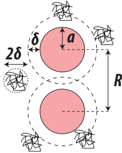
Figure 2.17: Schematic of a pair particles of radius a and with an exclusion radius of \delta .
