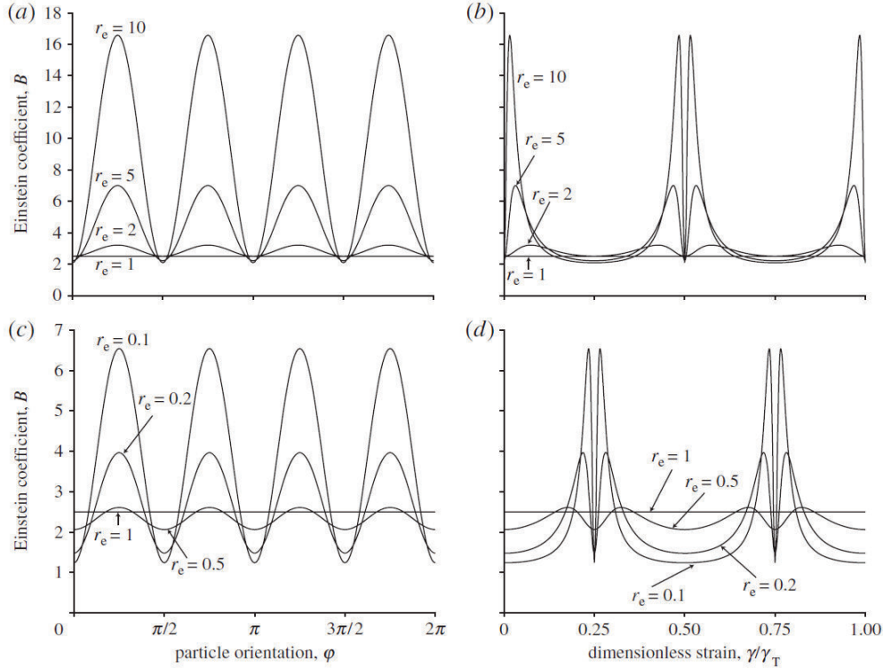
Figure 2.10: Einstein coefficient as a function of particle orientation (a,c) and dimensionless strain (b,d) for various equivalent spheroid aspect ratio, from [56].
