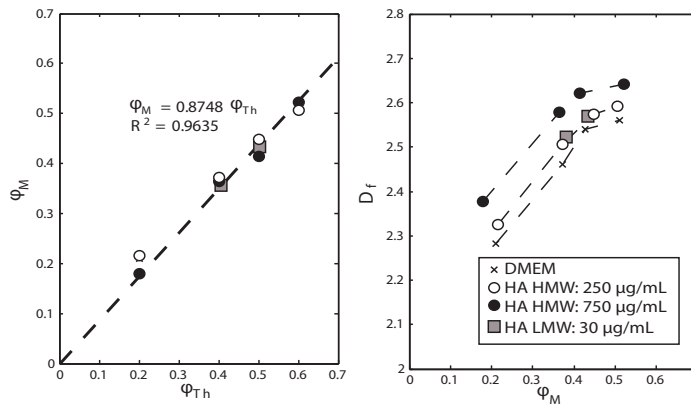
Figure 6.8: (A) Measured volume fraction as a function of the theoretical volume fraction. (B) Measured fractal dimension versus measured volume fraction.
