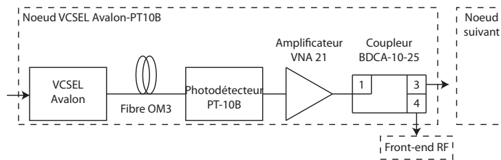
FIGURE 4.5 – Architecture du bloc VCSEL Avalon-PT10B.
