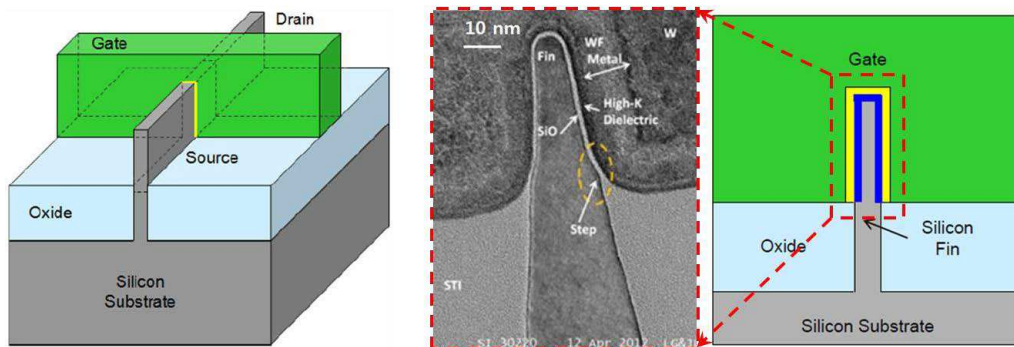
Figure 2. Intel's 22 nm bulk fully-depleted Tri-gate Transistor, 2011.
