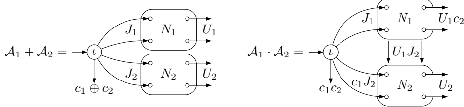
Figure 4.7: Automata for sum and concatenation
