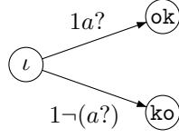
Figure 6.13: Automaton for state formula a
