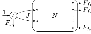
Figure 8.3: Standard pebble probabilistic automaton produced by the construction, from a hybrid probabilistic expression with terms \{\{E_1, E_2, \dots, E_n\}\} . Notice that the initial state \iota may be related to one of the terms, as it is shown on the picture.
