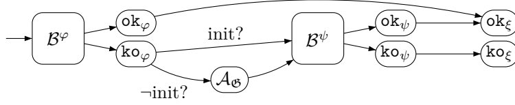
Figure 6.3: Weighted automaton for disjunction \xi = \varphi \vee \psi
