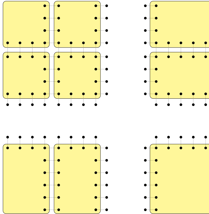
Figure 6.8: Zone partitioning of a picture
