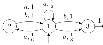
Figure 8.7: A probabilistic finite automaton
