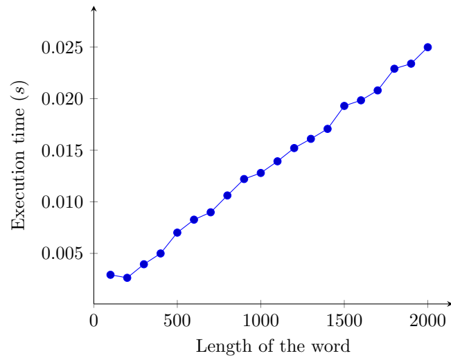
Figure 9.1: Plot of the execution time of the tool over expression (-final? \cdot (0.25 \cdot \rightarrow + 0.75 \cdot \leftarrow))^* \cdot final? as a function of the length of the word
