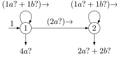
Figure 4.2: Weighted automaton \mathcal{A}'
