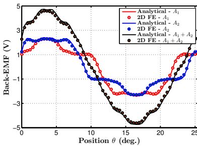
(c) Forme d'onde - 14 dents rotor - \gamma = 2 - n_c = 2
