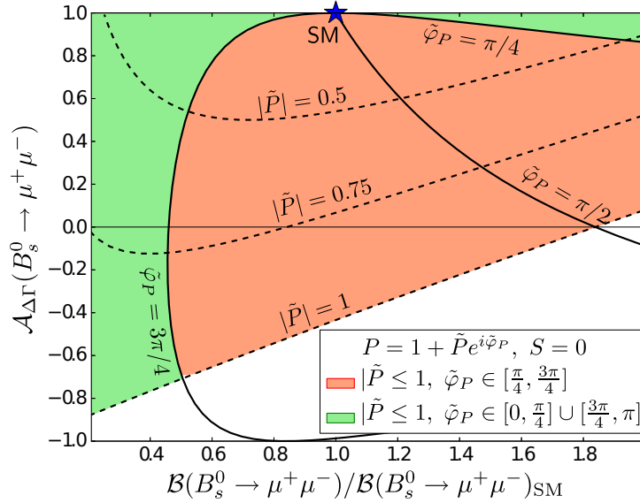
Figure 1.15: Allowed region in the plane \mathcal{B}(B_s^0 \rightarrow \mu^+\mu^-)/\mathcal{B}(B_s^0 \rightarrow \mu^+\mu^-)_{\text{SM}} \times \mathcal{A}_{\Delta\Gamma} . S , P , \varphi_{S,P} are defined in Equation 1.20 [41].
