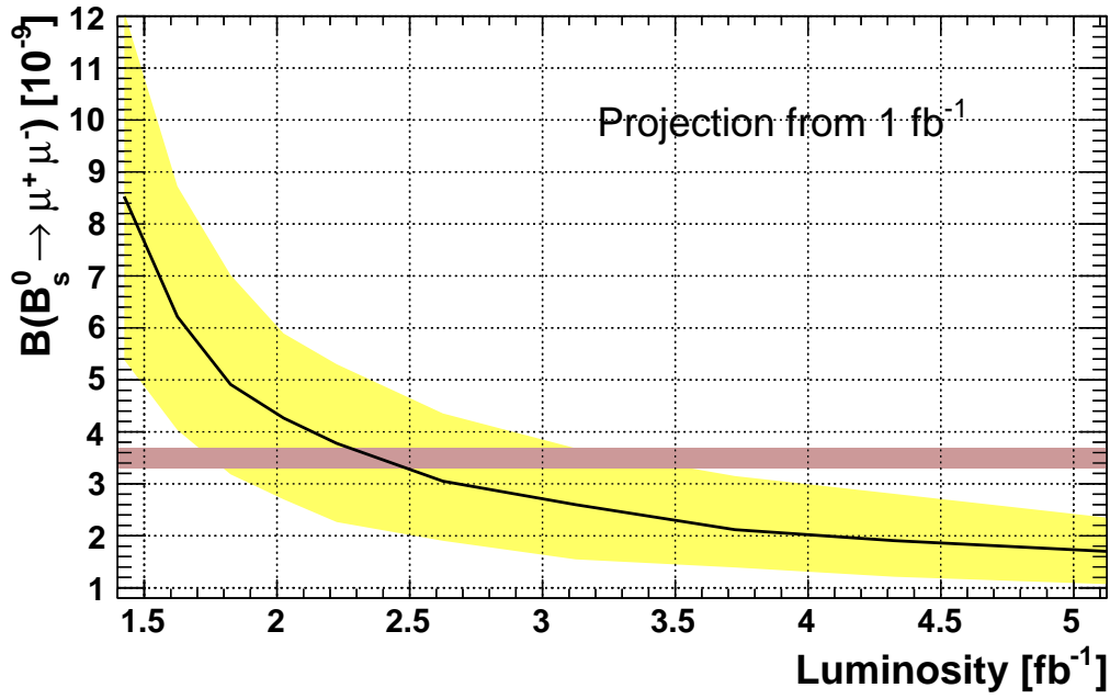
Figure 3.34: B_s^0 \rightarrow \mu^+\mu^- branching fraction at which an evidence with a significance of 3\sigma could be reached as a function of the integrated luminosity. Observed data pattern in the first 1.0\text{fb}^{-1} are accounted for. The black line is the B_s^0 \rightarrow \mu^+\mu^- branching fraction for which the \text{CL}_b distribution median corresponds to a p-value of 2.7 \times 10^{-3} . The yellow area covers all branching fraction values for which an evidence with a significance of 3\sigma could be observed if the \text{CL}_b fluctuated within one standard deviation from its median value. The brown horizontal area is the time integrated branching fraction prediction for the SM.
