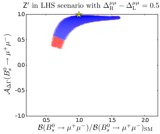
Figure 1.17: Allowed region in the plane \mathcal{B}(B_s^0 \rightarrow \mu^+\mu^-) / \mathcal{B}(B_s^0 \rightarrow \mu^+\mu^-)_{\text{SM}} \times \mathcal{A}_{\Delta\Gamma} assuming only left-handed currents, m_{Z'} = 1 \text{ TeV} , and Z' couplings between muons related as \Delta_R^{\mu\mu} - \Delta_L^{\mu\mu} = 0.5 . The two colours represent two oases of allowed values for the couplings. The star is the SM prediction [41].
