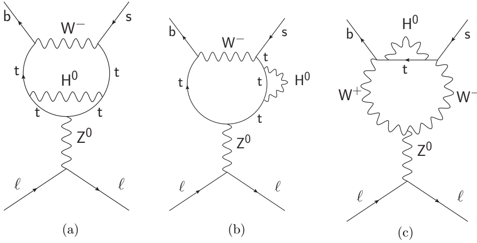
Figure 1.7: Main B_{(s)}^0 \rightarrow \ell^+ \ell^- Feynman diagrams with a SM Higgs boson.
