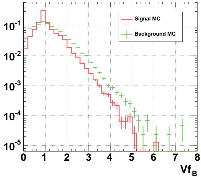
Figure 5.11: V_{f,B} distribution for the signal (red line) and combinatorial background (green crosses) from simulated data.
