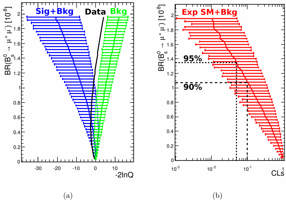
Figure 3.16: (a) Data test statistic compared to the expectations for the background-only and signal-plus-background hypotheses as a function of \mathcal{B}(\text{B}_s^0 \rightarrow \mu^+ \mu^-) . The error bars are centred at the median of the distribution and cover 34% on each side of the median. (b) \text{CL}_s as a function of \mathcal{B}(\text{B}_s^0 \rightarrow \mu^+ \mu^-) . The 95% (90%) C.L. upper limit is obtained for \text{CL}_s = 5\% (10%).
