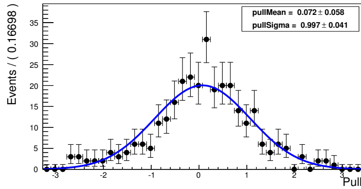
Figure 3.20: Pull of the slope sl2 of the second BDT exponential (see Equation 3.11).
