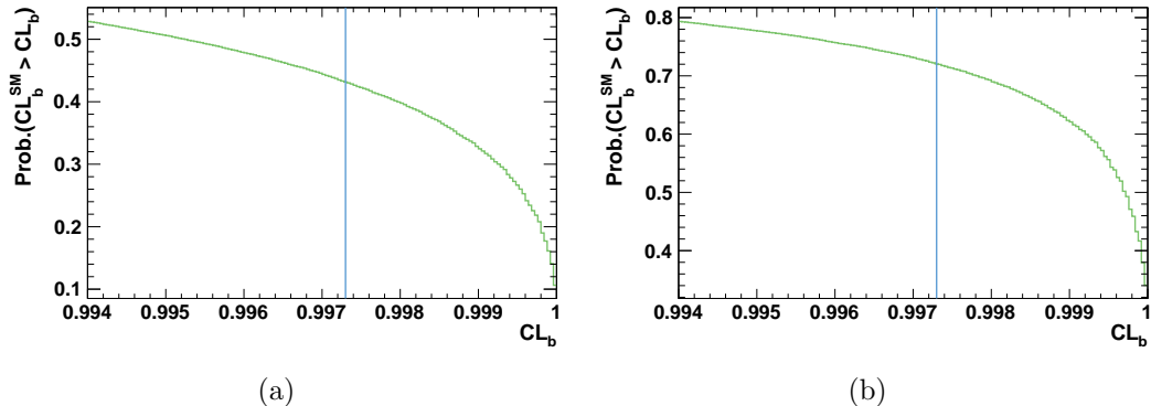
Figure 3.36: Probability to have a CL_b larger than a given value if the signal was observed at the SM rate for the 2012 dataset (a) and combining with one from 2011 (b). The vertical blue lines indicates the CL_b value corresponding to a signal evidence with a significance of 3\sigma
