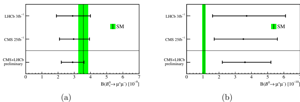
Figure B.6: Comparison of the latest CMS and LHCb results [1, 2], the combined value, and the SM prediction (vertical line) for (a) the time-integrated branching fraction \mathcal{B}(\mathbf{B}_s^0 \rightarrow \mu^+ \mu^-) and (b) \mathcal{B}(\mathbf{B}^0 \rightarrow \mu^+ \mu^-) . The width of the vertical band represents the uncertainty in the SM prediction. The error bars represent the combined statistical and systematic uncertainties.
