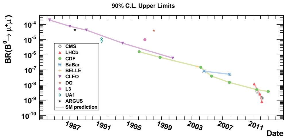
Figure 3.2: Upper limits at 90% C.L. on \mathcal{B}(B^0 \rightarrow \mu^+ \mu^-) since the first analysis in 1984. The results of the analysis described in this thesis are not included.
