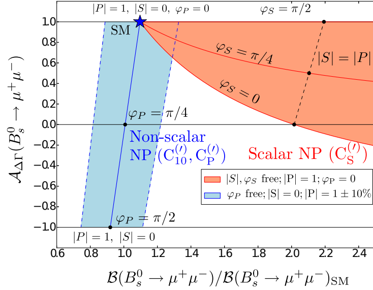
Figure 1.9: Allowed region in the plane \mathcal{B}(B_s^0 \rightarrow \mu^+ \mu^-) / \mathcal{B}(B_s^0 \rightarrow \mu^+ \mu^-)_{SM} \times \mathcal{A}_{\Delta\Gamma} if new physics contributions are or not scalar [40]. S , P , \varphi_{S,P} are defined in Equation 1.20.
