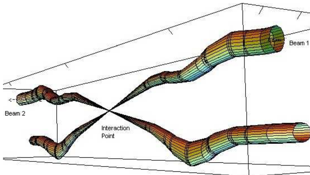
Figure 2.2: Two proton beams around an interaction point.
