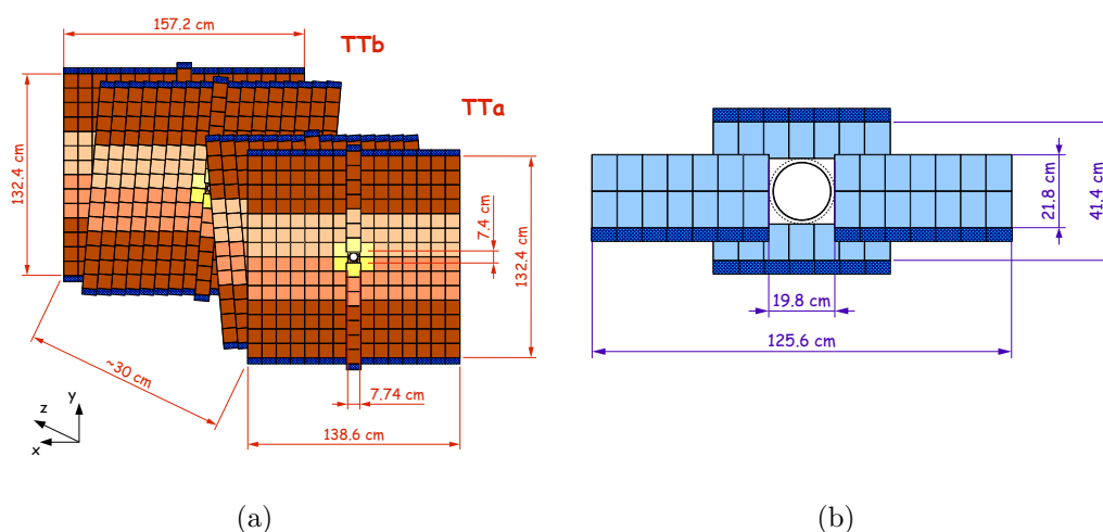
Figure 2.12: Layout of the xvvy TT layers(a) and of one x IT layer (b).
