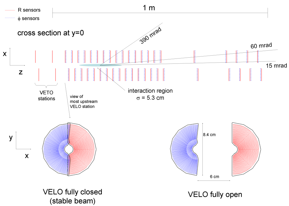
Figure 2.10: VELO dectector layout.
