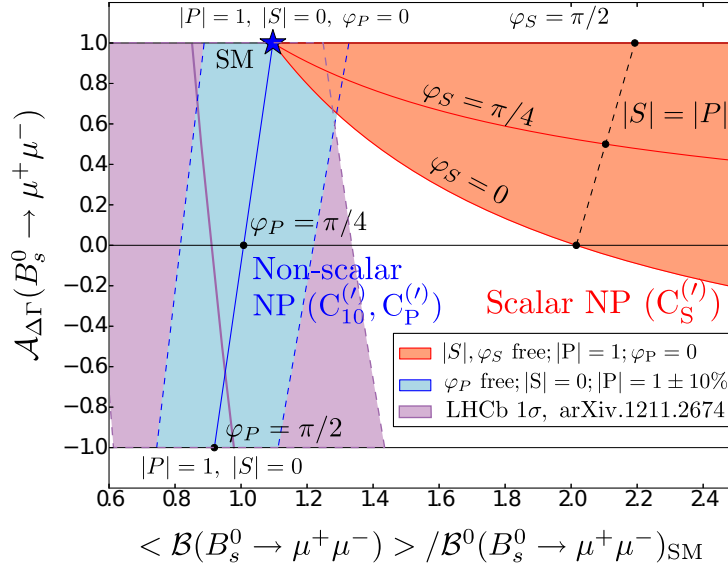
Figure 4.7: Allowed region in the plane \mathcal{B}(B_s^0 \rightarrow \mu^+ \mu^-) / \mathcal{B}(B_s^0 \rightarrow \mu^+ \mu^-)_{SM} \times \mathcal{A}_{\Delta\Gamma} if new physics contributions are scalar or not superimposed with the experimental constraint (modified from [12]). S , P , \varphi_{S,P} are defined in Equation 1.20.
