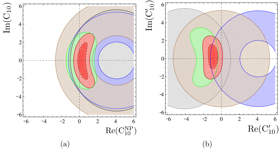
Figure 1.11: Values for the C_{10} (a) and C'_{10} (b) Wilson coefficients consistent at 1\sigma with the experimental results from \mathbf{B}^0 \rightarrow \mathbf{X}_s \ell^+ \ell^- (brown), \mathbf{B}^0 \rightarrow \mathbf{K} \mu^+ \mu^- (blue), \mathbf{B}^0 \rightarrow \mathbf{K}^{*0} \mu^+ \mu^- (green), \mathcal{B}(\mathbf{B}_s^0 \rightarrow \mu^+ \mu^-) = 2.4 \pm 1.6 \times 10^{-9} (gray) and with their combination (red) at 1 and 2 \sigma [26].
