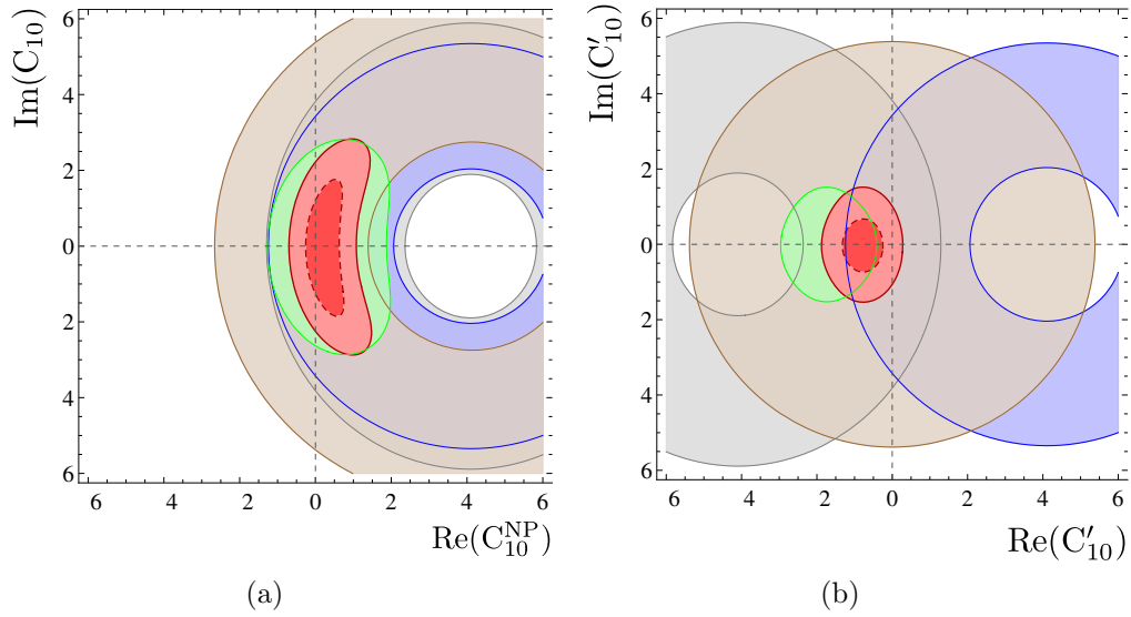
Figure 4.9: Values for the C_{10} (a) and C'_{10} (b) Wilson coefficients consistent at 1\sigma with the experimental results from \text{B}^0 \rightarrow \text{X}_s \ell^+ \ell^- (brown), \text{B}^0 \rightarrow \text{K} \mu^+ \mu^- (blue), \text{B}^0 \rightarrow \text{K}^{*0} \mu^+ \mu^- (green), \mathcal{B}(\text{B}_s^0 \rightarrow \mu^+ \mu^-) = 3.2^{+1.5}_{-1.2} \times 10^{-9} (gray) and with their combination (red) at 1 and 2 \sigma [14]. The constraints improve slightly with respect to Figure 1.11.
