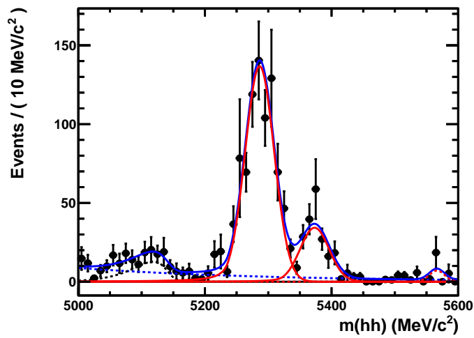
Figure 3.10: Invariant mass distribution of B_{(s)}^0 \rightarrow h^+h^- candidates in the last BDT bin [0.9–1]. The red solid lines show the B^0 \rightarrow h^+h^- and B_s^0 \rightarrow h^+h^- signals, and the red dashed one the \Lambda_b \rightarrow p h^- signal. The combinatorial background is shown by the blue dashed line, while the physical background (partially-reconstructed) is shown by the black dashed line. Hadrons are identified as kaons if DLL(K, \pi) \geq 5 , as pions if -DLL(K, \pi) \geq 5 and rejected if |DLL(K, \pi)| \leq 5 .
