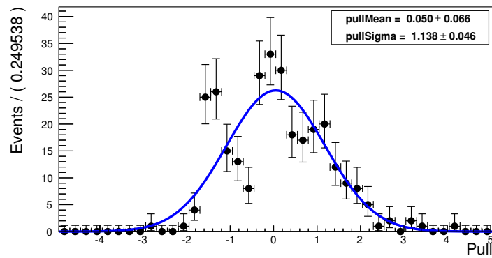
Figure 3.21: Pull of the slope sl3 of the third BDT exponential (see Equation 3.11).
