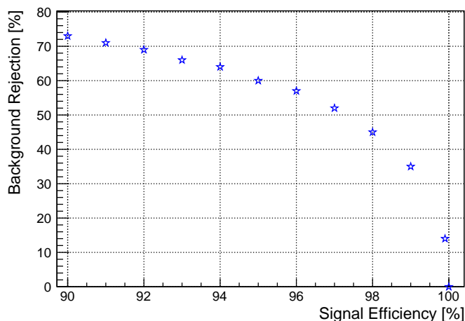
Figure 3.6: Background rejection versus signal efficiency for a BDT based selection computed with simulated B_s^0 \rightarrow \mu^+ \mu^- as signal and B_{(s)}^0 \rightarrow h^+ h'^- data sidebands as background.
