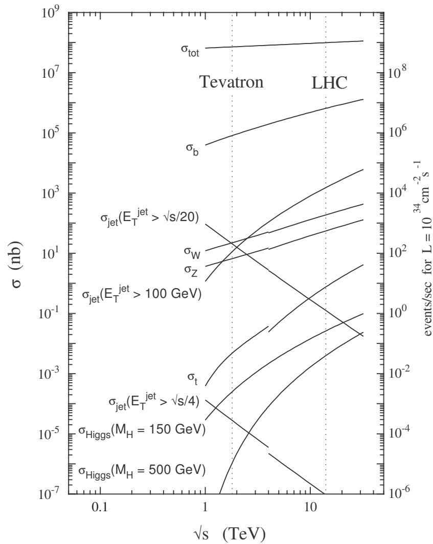
Figure 2.4: Production cross section of various processes as a function of the pp centre of mass energy.
