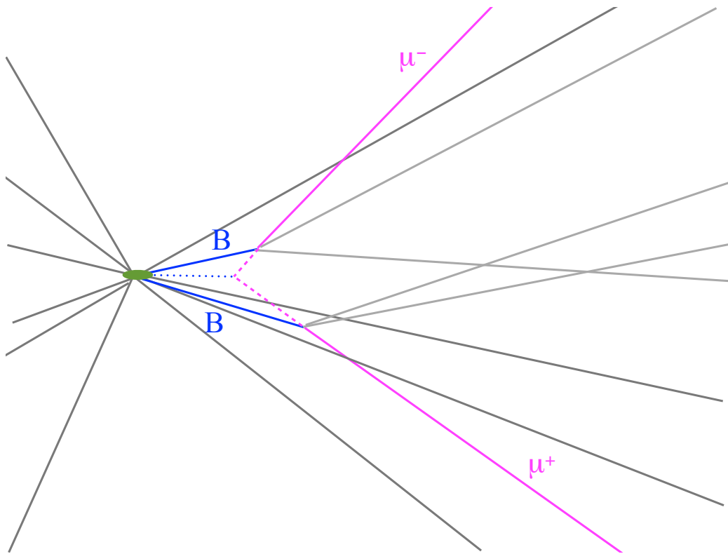
Figure 3.3: Cartoon of a typical combinatorial candidate. The green ellipse is the primary vertex. The two pink lines are muons which originate from the decays of two B mesons (blue). Their extrapolations (dashed pink) cross and make the B candidate vertex (dashed blue).
