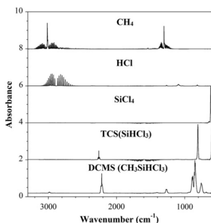
Fig. 6. Experimental IR spectra of pure species (CH 4 , HCl, SiCl 4 , HSiCl 3 , CH 3 SiCl 2 ).
