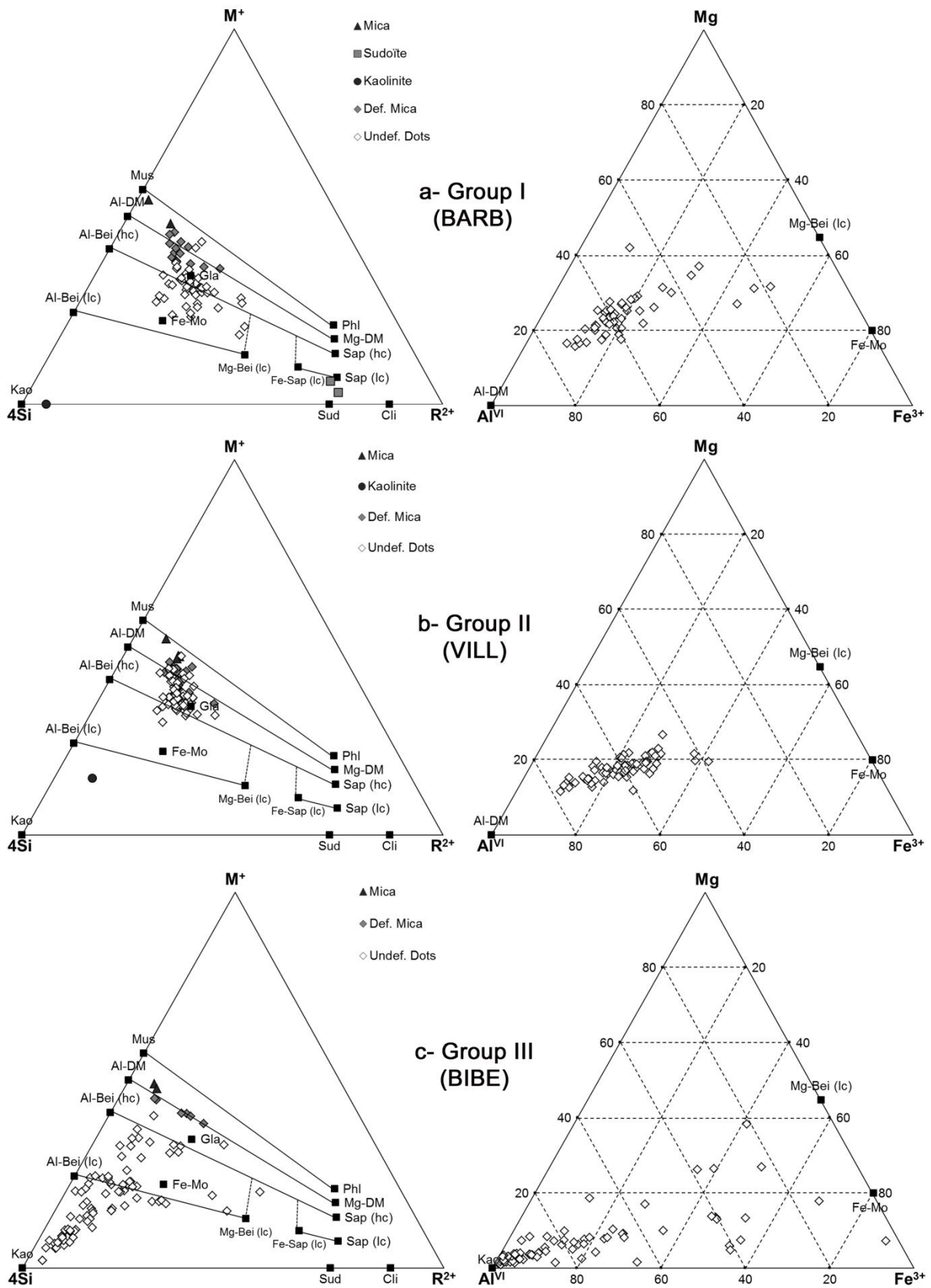
Fig. 2. Results from crystal-chemical composition of < 4 \mu\text{m} fractions of (a) group I (BARB), (b) group II (VILL), and (c) group III (BIBE) plotted in the \text{M}^+ - 4\text{Si} - \text{R}^{2+} (left) and \text{Mg} - \text{Al}^{\text{VI}} - \text{Fe}^{3+} (right, only undefined dots) ternary diagrams (adapted from Meunier & Velde, 1989).
