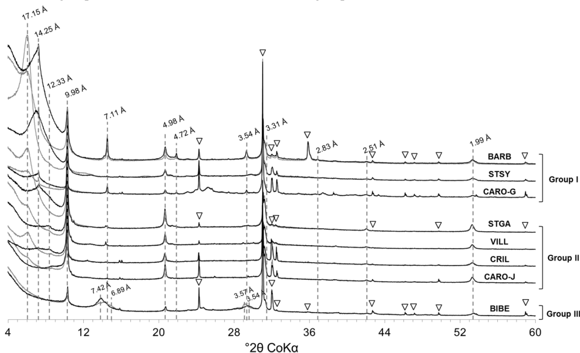
Fig. 1. Normalized experimental XRD patterns of bulk < 4 \mu\text{m} fractions for group I (BARB, STSY, CARO-G), group II (STGA, VILL, CRIL, CARO-J) and group III (BIBE). The solid black and grey lines represent the XRD patterns recorded in AD and after EG solvation, respectively. Open triangles indicate the diffraction peaks related to the presence of quartz, feldspar, rutile, hematite, goethite, ankerite or siderite as accessory minerals.
