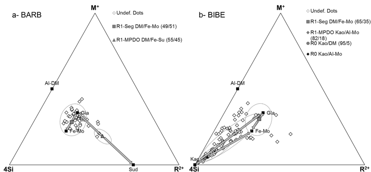
Fig. 7. Clay mineral phases repartition in the M^+–4Si–R^{2+} ternary diagram based on XRD profile modeling results. The grey dotted lines enclose the analytical dots belonging to the corresponding MLM phases used in the profile modeling of XRD patterns.
