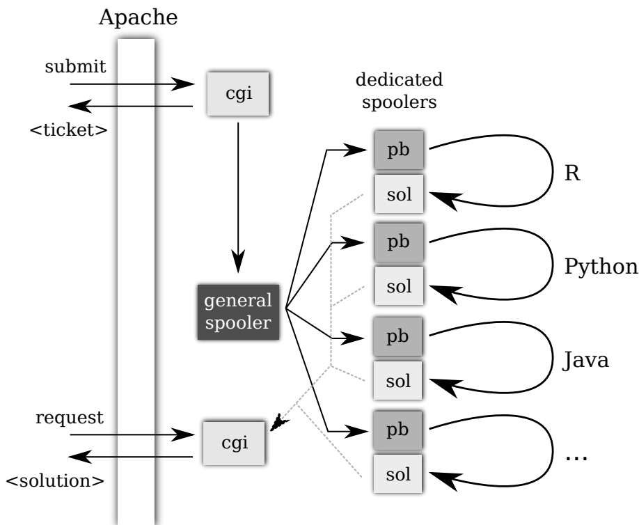
FIGURE 3.2 – Architecture des services-web XMCDA.
