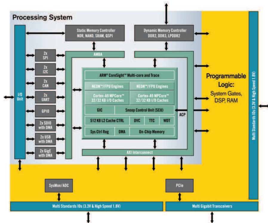
FIGURE 5.3 – Zynq.
