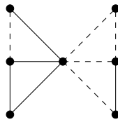
Figure 5.7: A signified outerplanar graph with signified relative clique number 7.
