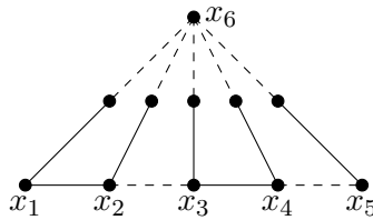
Figure 5.4: (B, \Lambda) is a signified planar graph with girth 5.
