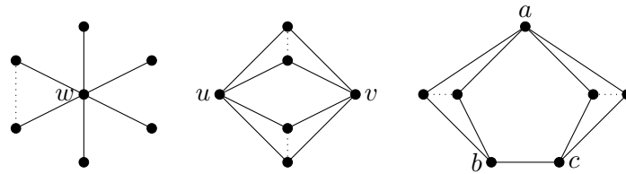
Figure 2.1: List of all triangle-free planar graphs with diameter 2 (Plesnik (1975)).
