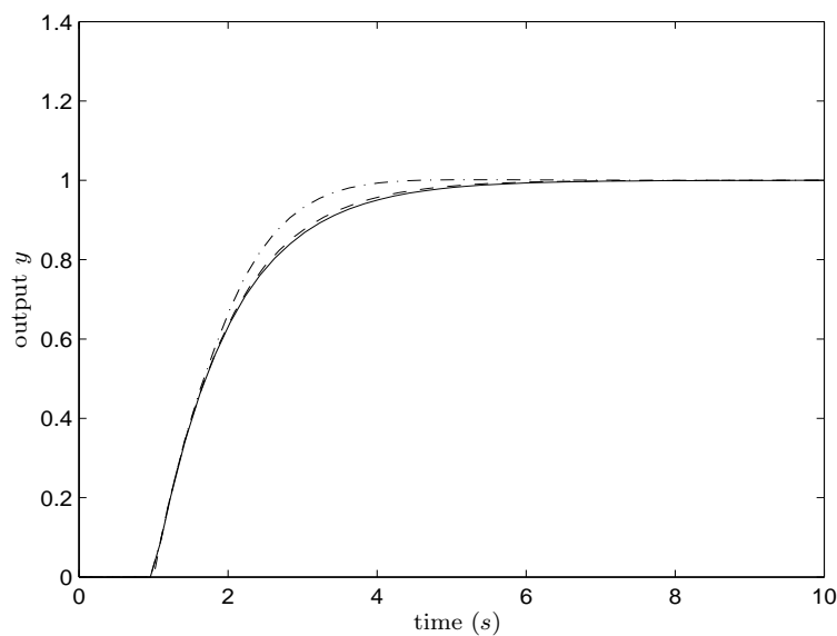
FIGURE 4.4: Step responses for the desired closed-loop (continuous line) and for the closed-loop system with approximation of distributed delay with 5th order (dash) and 2nd order (dot-dash), (Example 4.3).
