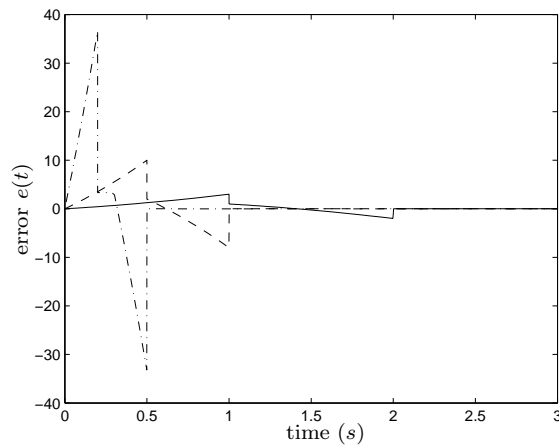
FIGURE 3.15: Trajectory planning control, for \vartheta_1 = \vartheta_2 = 0.5 (dashed), \vartheta_1 = \vartheta_2 = 1 (continuous), and \vartheta_1 = 0.2, \vartheta_2 = 0.3 (dashed-dot) (Example DC-motor).
