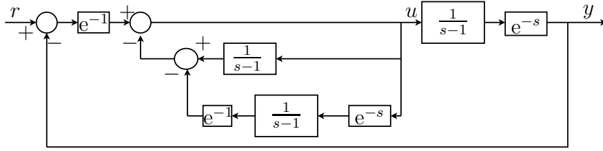
FIGURE 2.4: Stabilizing control of Example 2.2
