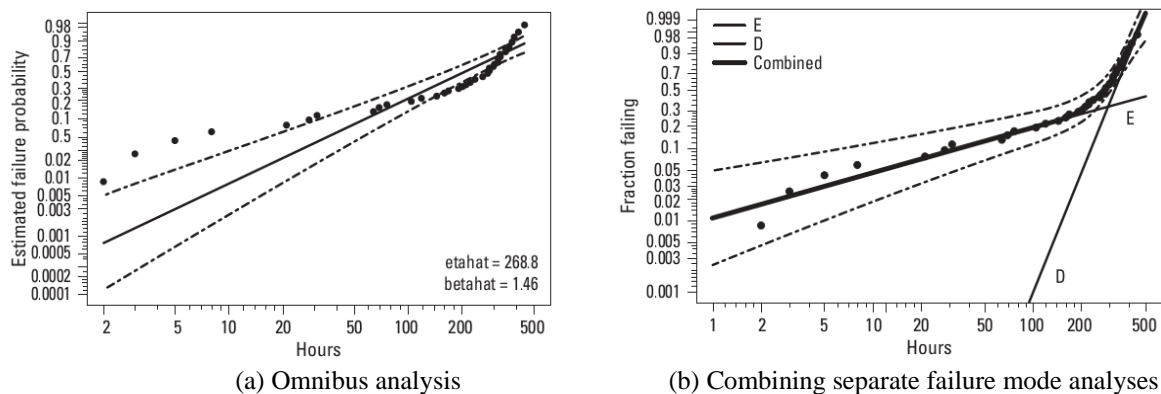
Figure 35: Weibull Probability Plot for Voltage Endurance Data [114].
