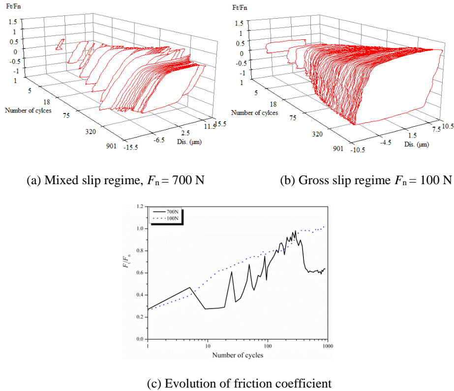
Figure 59: Fretting loops and the evolution of friction force ratio under \pm 10 \mu\text{m} .
