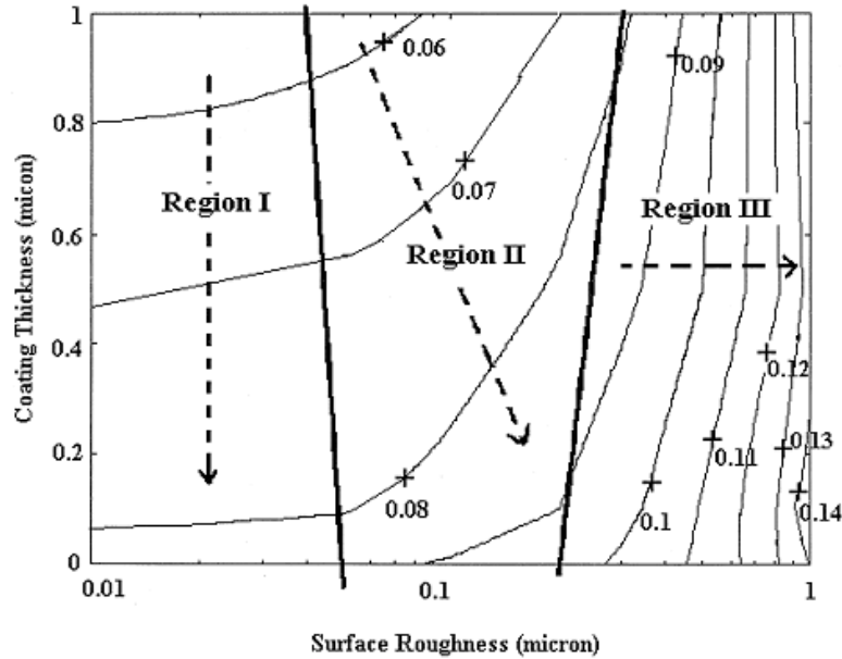
Figure 22: Map showing the effect of surface roughness and MoS T coating thickness on friction coefficient contours are lines of equal friction coefficient [87].
