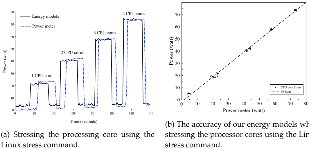
Figure 3.5: Accuracy of CPU model
