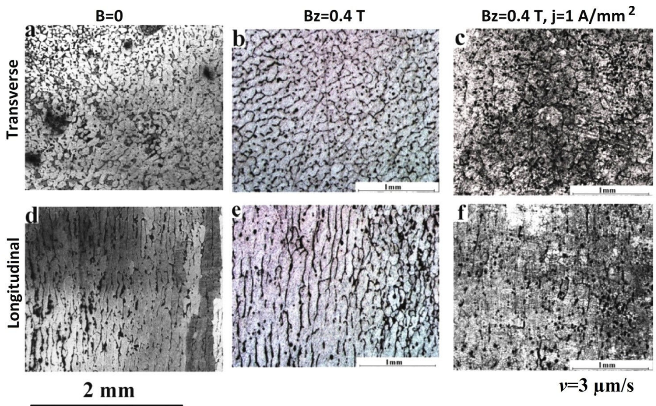
Figure 6.8: Structure of directionally solidified Sn-10%wt.Pb alloy at v=3 \text{ } \mu\text{m/s} : a,d) without field; b,e) with 0.4 T axial field; c,f) with 0.4 T axial field and 1 \text{ A/mm}^2 axial current
