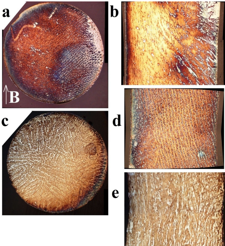
Figure 9.2: Directionally solidified Sn-20%wt.Bi at 10 \mu\text{m/s} ( \theta=8 \text{ K/mm} ); a,b,d) with 0.4 T transverse magnetic field ; c,e) without magnetic field
