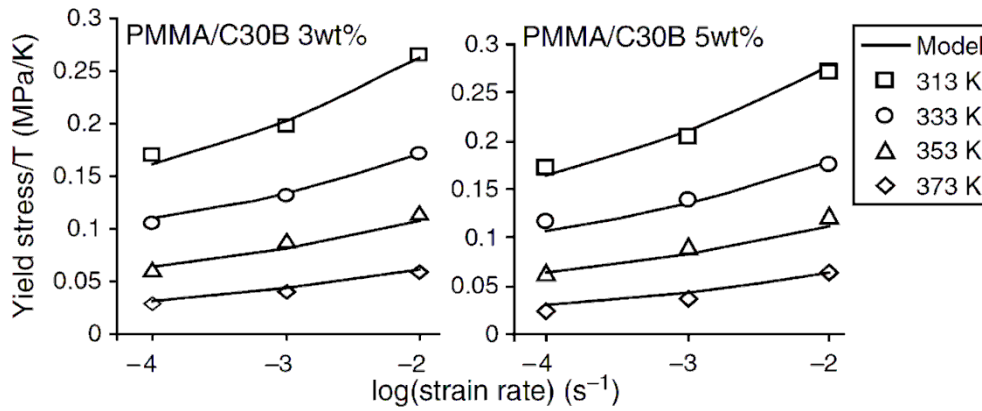
Figure 1-32: Yield stress/temperature versus strain rate of PMMA/organoclay nanocomposites with different clay concentrations [91].
