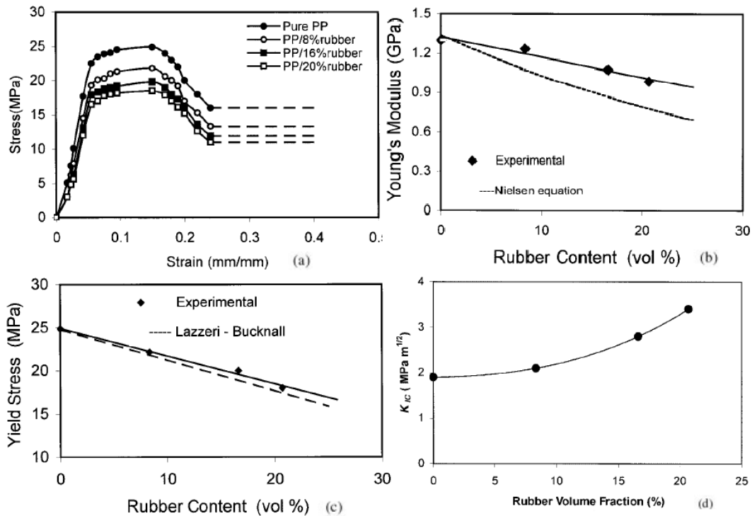
Figure 1-13: Influence of EPM content (a) quasi static tensile stress-strain curves (b) Young's modulus (c) Yield stress (d) fracture toughness (strain rate 0.03 \text{ s}^{-1} ) [24].
