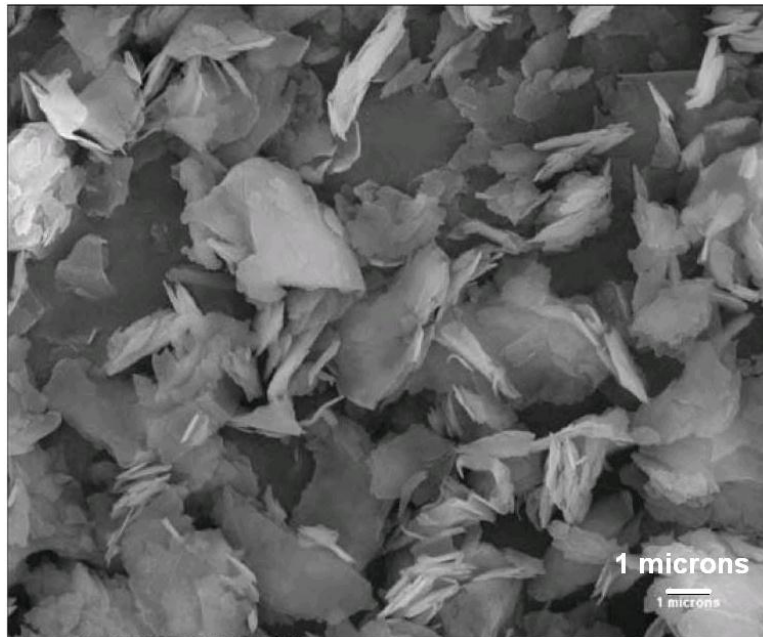
Figure 1-9: micrograph of talc [2].
