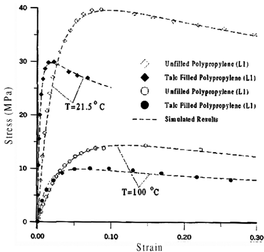
Figure 1-15: Comparison of the stress strain curves of unreinforced and reinforced polypropylene with 40 wt.% talc at 21.5 °C and 100 °C under strain rate 5 min -1 [26].
