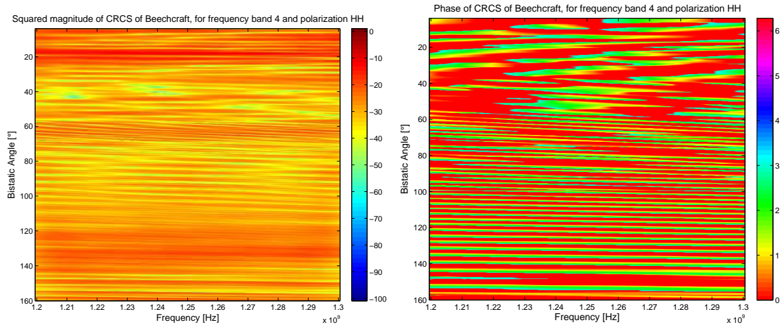
Figure 4.18: Squared magnitude (left) and phase (right) of the BS-CRCSs of a Beechcraft as a function of frequency f and bistatic angle \beta , for FB4 ( f \in [1.2; 1.30] GHz), and for the following fixed parameters: Pol = HH , \theta = 0^\circ , and \phi = -10^\circ .
