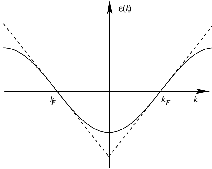
Figure 1.1: The dispersion of a one-dimensional model of fermions (solid line) and the dispersion linearized near the Fermi points.
