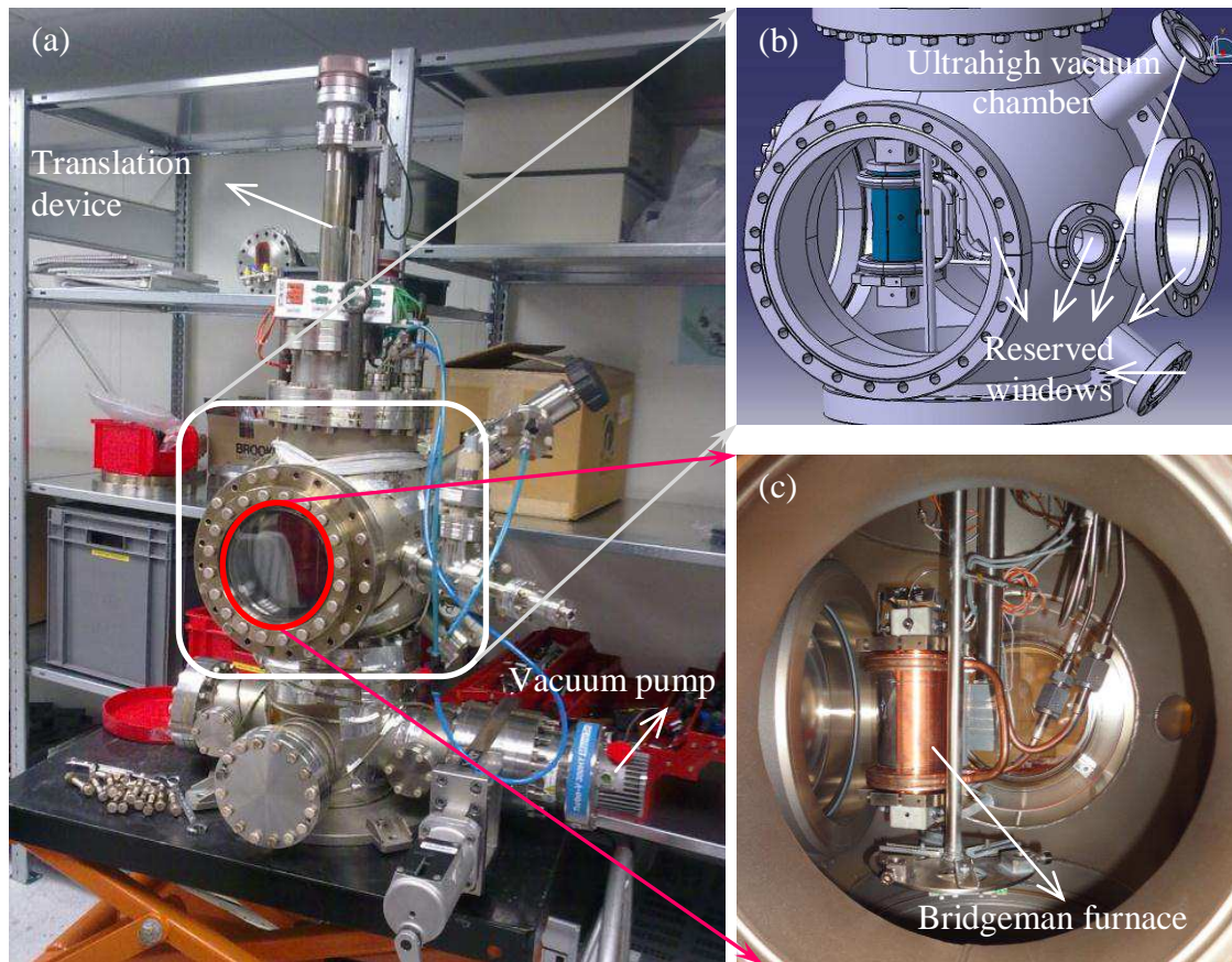
Figure 3.2 Photos and 3D drawing of ultrahigh vacuum Bridgeman furnace.
