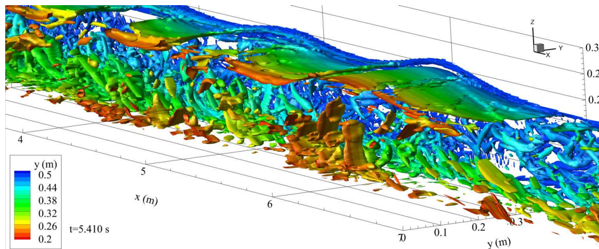
(b) Simulation rad3DSEM, criterion Q plotted for y > 0.2 , bore front at x = 6 m, t = 5.41 s
