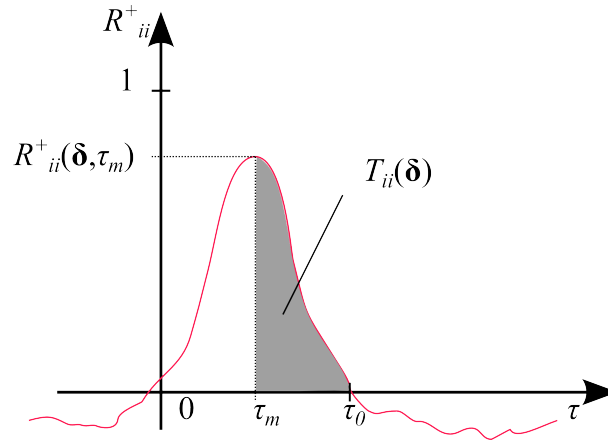
Figure III.8: Definition sketch of cross correlation function and correlation time scale
