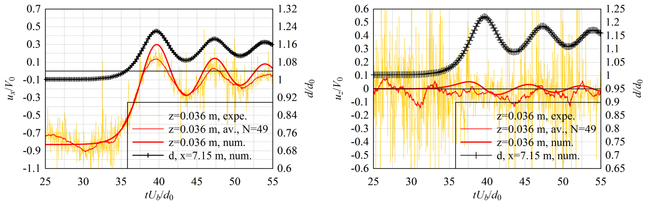
(a) Longitudinal velocity at z/d_0 = 0.181
