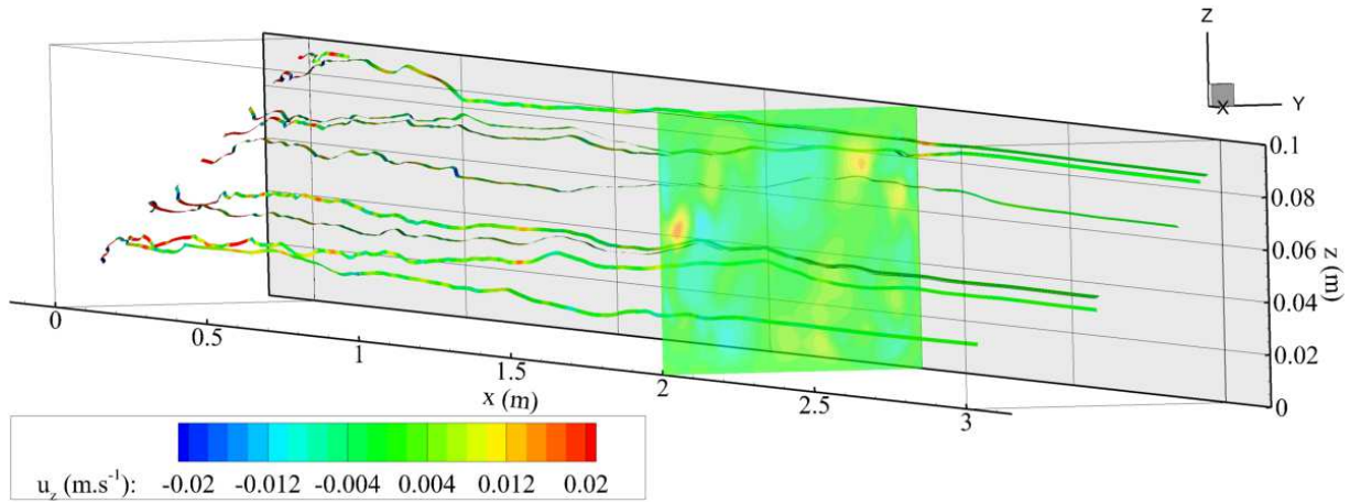
Figure V.7: Numerical domain with streamlines. The slice at x = 2 m indicates the position of the damping layer downstream the channel. Run 4 at t = 21.53 s
