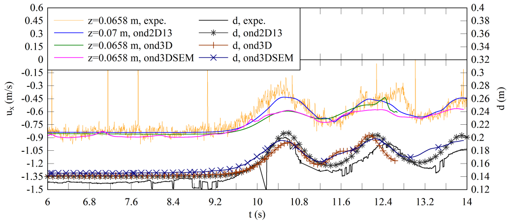
(a) Longitudinal component
