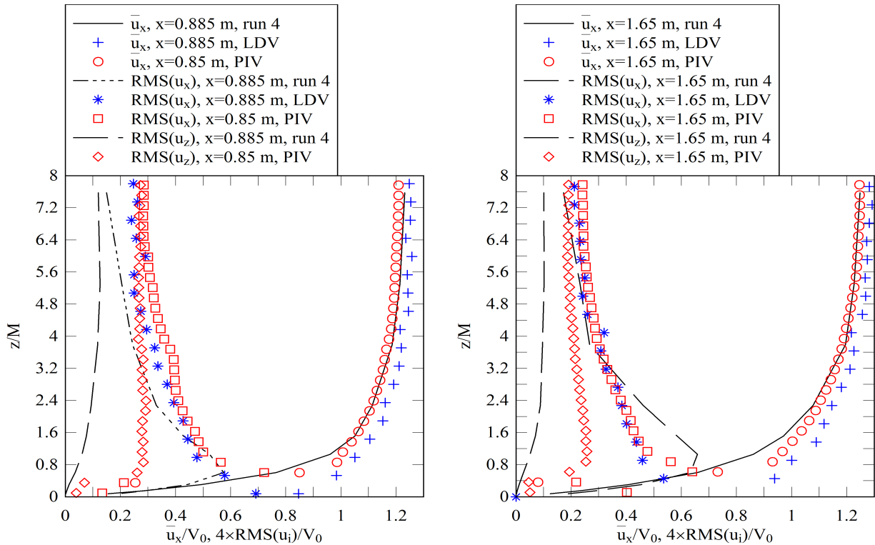
(b) Half of the vertical profile at x \approx 0.9 m and y = 0.05 m and (c) Half of the vertical profile at x = 1.65 m and y = 0.05 m
