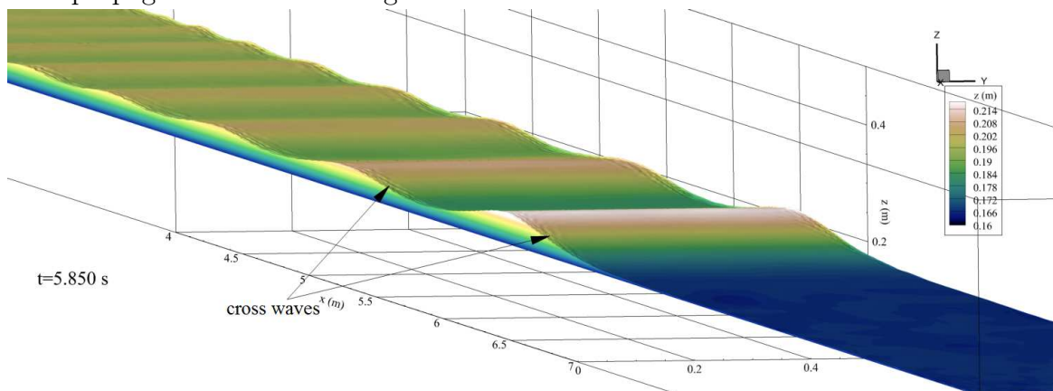
Figure VI.12: Details of the undular bore propagation at t = 5.85 \text{ s} for the simulation rad3DSEM
