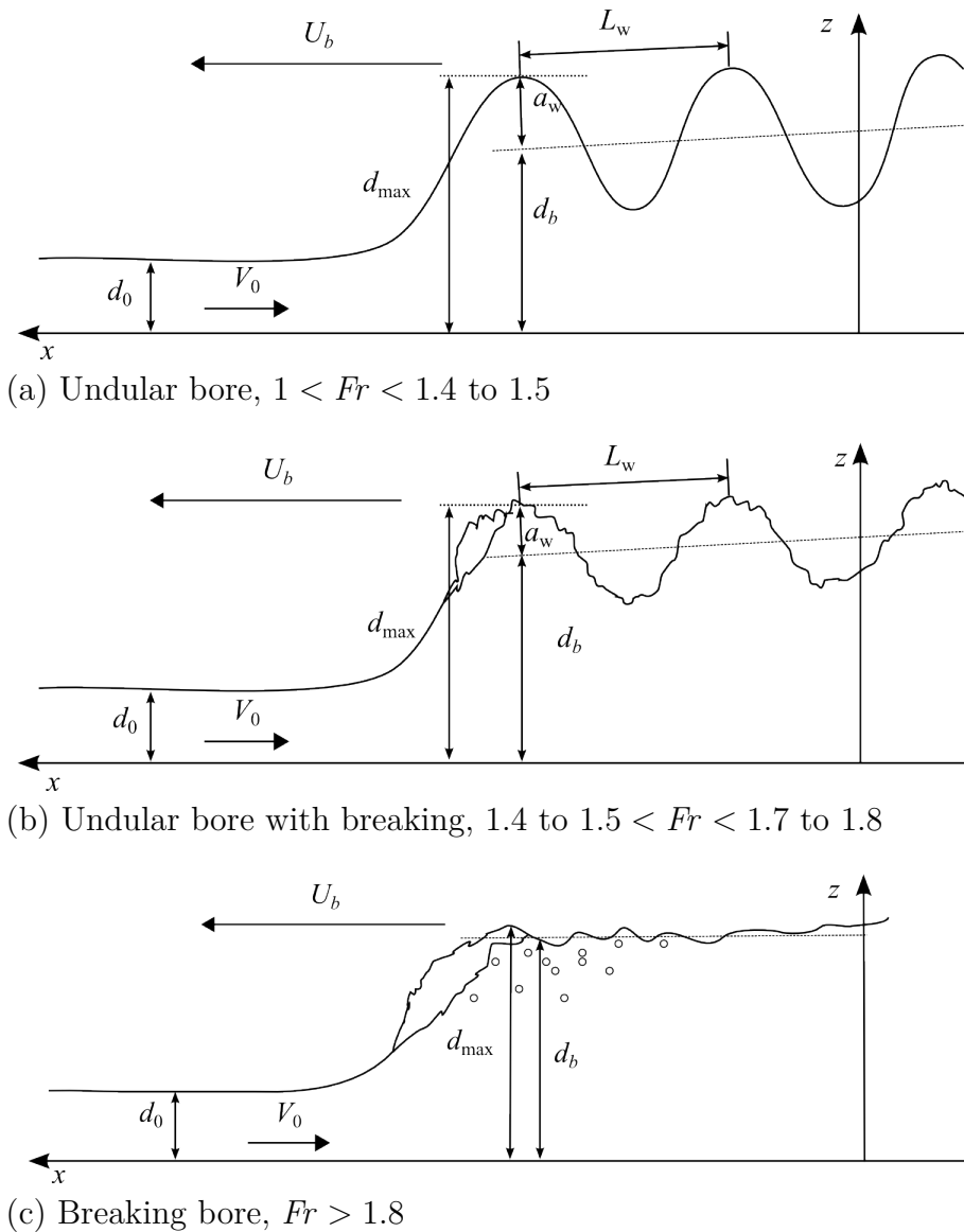
Figure IV.13: Definition sketches of bores observed in the present study
