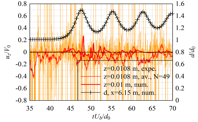
(b) Vertical velocity at z/d_0 = 0.078
