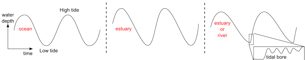
(b) Typical tidal cycle evolution as the tide propagate from the ocean to the river leading to the appearance of a tidal bore, with zoom on a tidal bore
