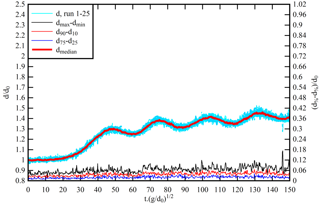
Figure A.1: Ensemble averaged free surface data for an undular bore. Flow conditions: Fr = 1.14 , Q = 0.036 \text{ m}^3 \cdot \text{s}^{-1} , d_0 = 0.088 \text{ m} , h_g = 57 \text{ mm}
