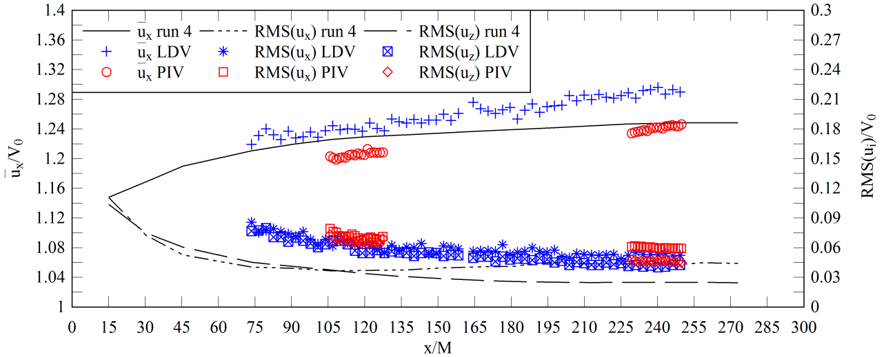
(a) Longitudinal profile on the channel centreline
