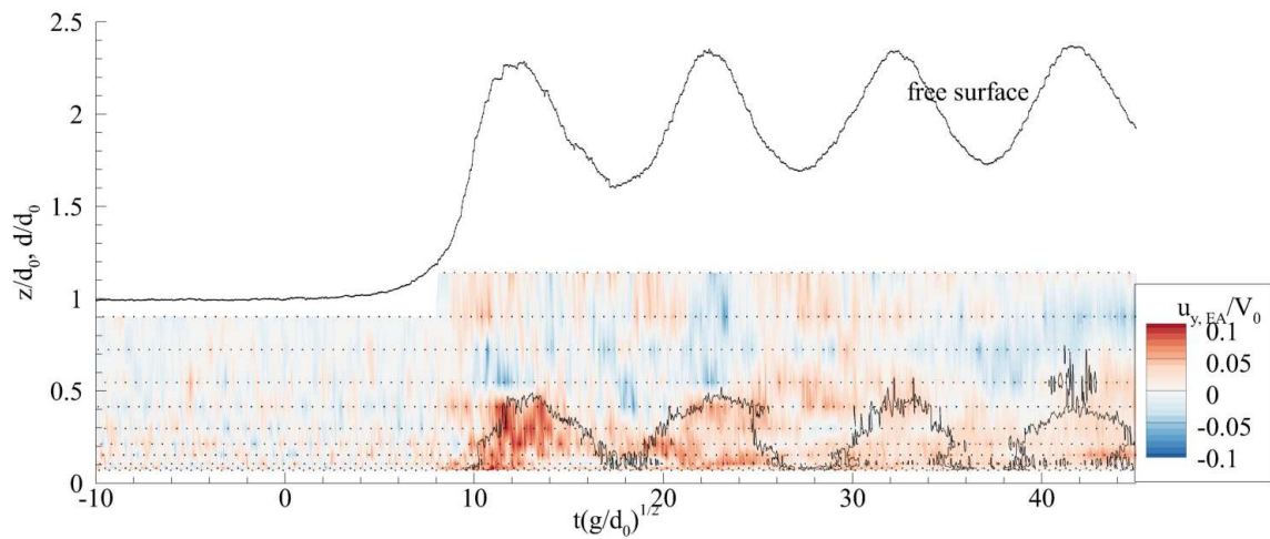
(b) Transversal velocity
