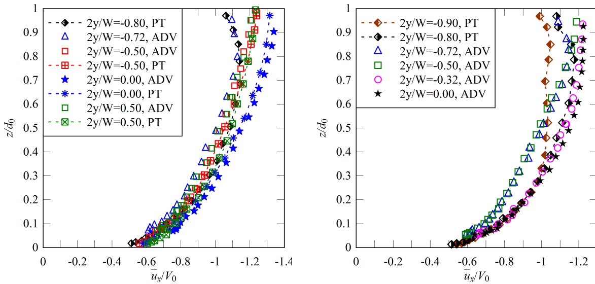
(a) Comparison between Pitot tube (PT) and ADV data, Q = 0.036 \text{ m}^3 \cdot \text{s}^{-1}
