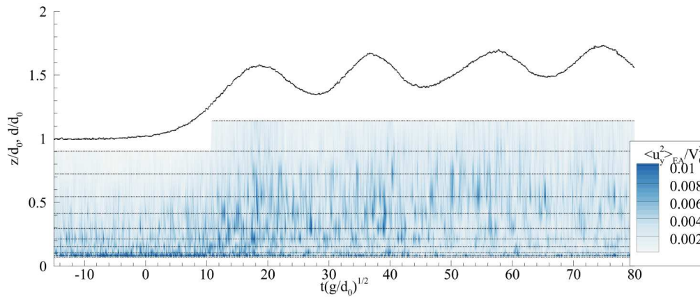
(b) Transversal velocity
