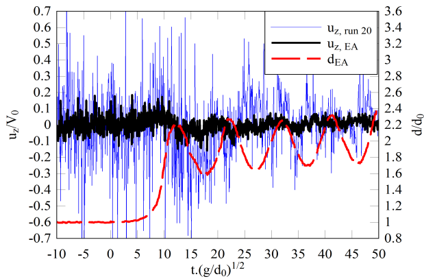
(e) Vertical velocity at z/d_0 = 0.15
