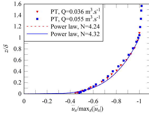
Figure IV.6: Dimensionless distributions of longitudinal velocity component in the developing boundary layer at x = 6.13 m on the channel centre line. Comparison between Pitot tube (PT) data and power law
