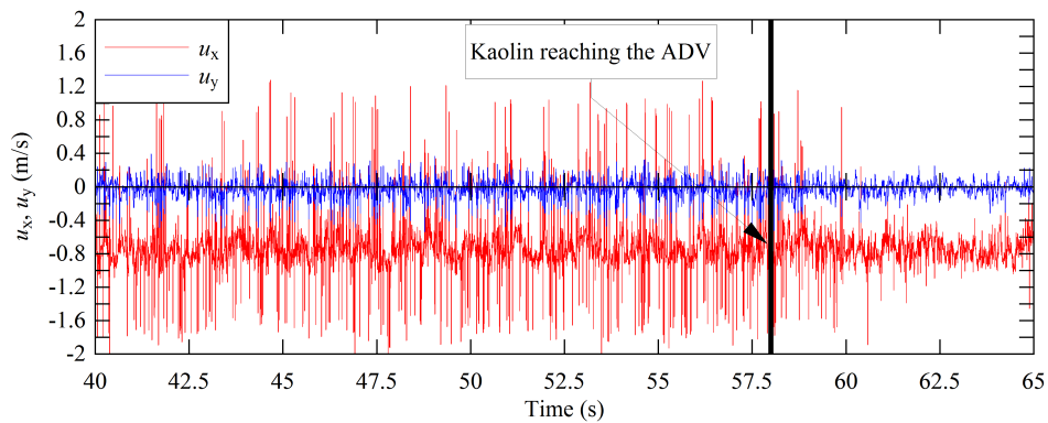
(a) Longitudinal and transversal velocity
