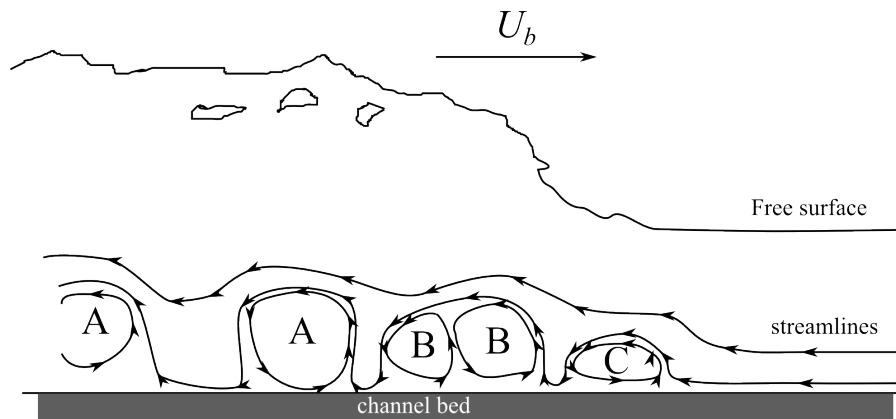
Figure II.4: Sketch of streamlines indicating recirculation structures under a propagating breaking tidal bore. (A) indicates macro-structures propagating downstream, (B) shows separating structures, shedding and propagating downstream and (C) is the main recirculation structure propagating upstream with the bore. Based on Lubin et al. (2010a)
