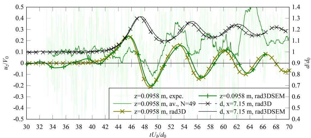
(c) Vertical component
