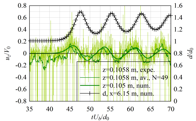
(f) Vertical velocity at z/d_0 = 0.764
