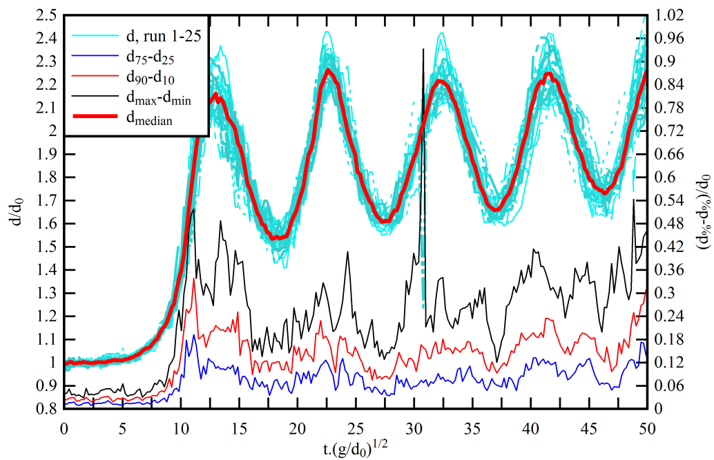
Figure A.9: Ensemble averaged free surface data for a breaking bore. Flow conditions: Fr = 1.56 , Q = 0.036 \text{ m}^3 \cdot \text{s}^{-1} , d_0 = 0.088 \text{ m} , h_g = 0 \text{ mm}
