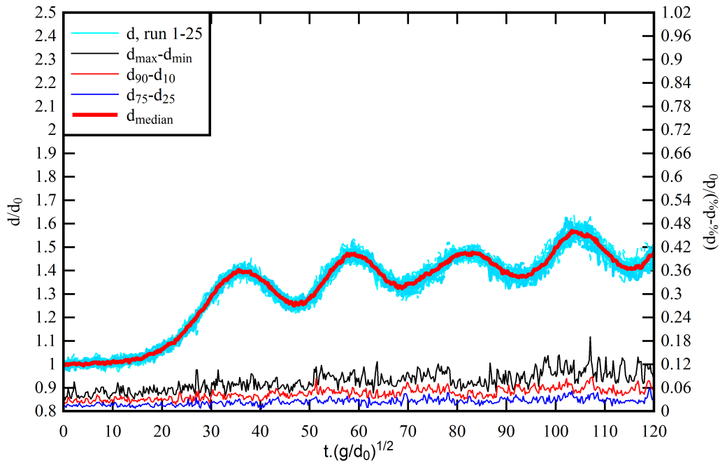
Figure A.2: Ensemble averaged free surface data for an undular bore. Flow conditions: Fr = 1.18 , Q = 0.036 \text{ m}^3 \cdot \text{s}^{-1} , d_0 = 0.089 \text{ m} , h_g = 51 \text{ mm}
