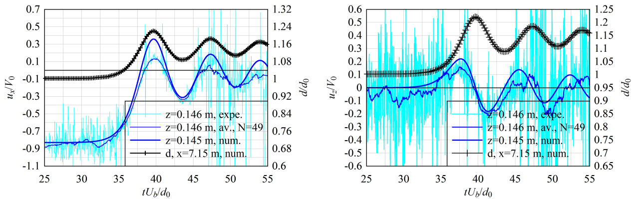
(c) Longitudinal velocity at z/d_0 = 0.734
