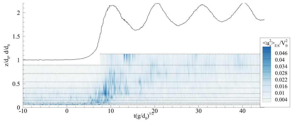
(a) Longitudinal velocity stress
