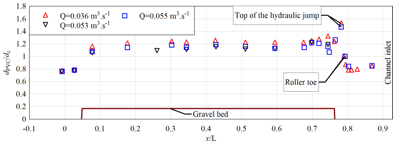
Figure IV.2: Dimensionless free surface profiles along the channel centreline in steady flows. The flow direction from right to left with the gate at x = 0 where L = 12 \text{ m} was the channel length. Note that the gravel bed height is not at scale
