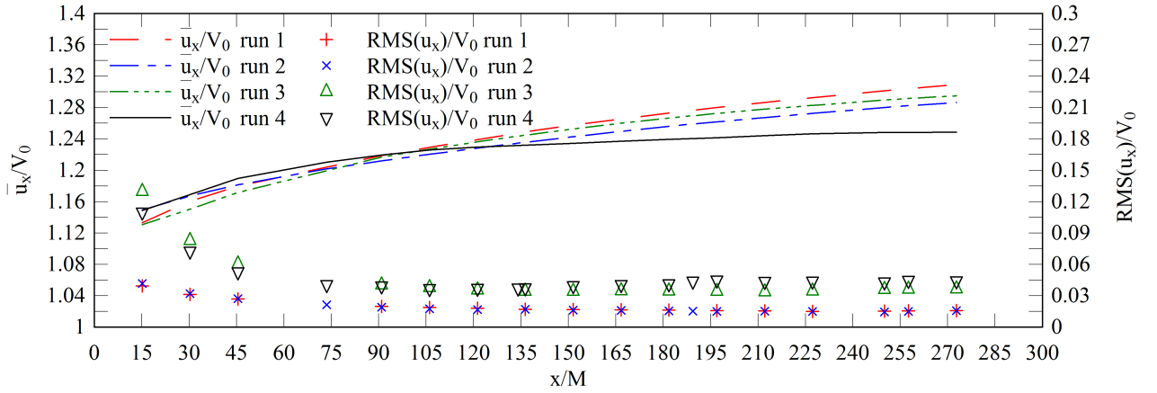
(a) Longitudinal velocity and RMS profiles
