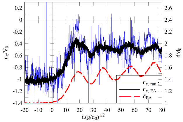
(b) Longitudinal velocity at z/d_0 = 0.29
