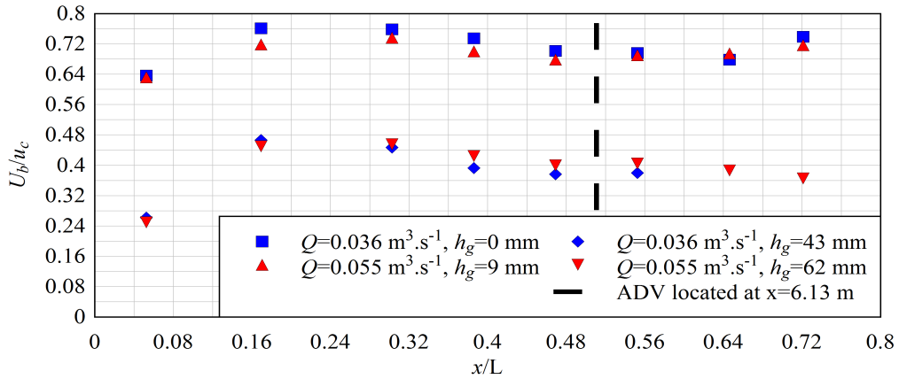
(a) Ensemble-averaged bore celerity
