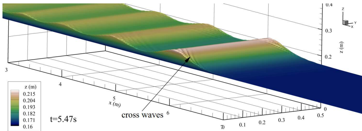
Figure VI.10: Details of the undular bore propagation at t = 5.47 s for the simulation rad3D the secondary undulations close to the sidewalls when the water level increased in the case of simulation rad3D (Figures VI.10). As the bore propagated, the end of the wave train (tail) detached from the gate. New undulations appeared from the tail. Between the tail of the secondary undulations and the gate ( x = 0 ), the water level remained globally unchanged during the bore propagation with small variations within the size of the mesh ( \Delta_z = 2.4 mm). The wave length and amplitude of the secondary undulations from the front to the tail progressively decreased (Figure VI.9 and VI.11). Overall, the bore propagation showed a two dimensional aspect similar to the experiment (Chanson, 2010a) and similar to the two dimensional simulation rad2D13 with the addition of small cross waves on the sidewalls also seen during experiments (Chanson, 2010a).
