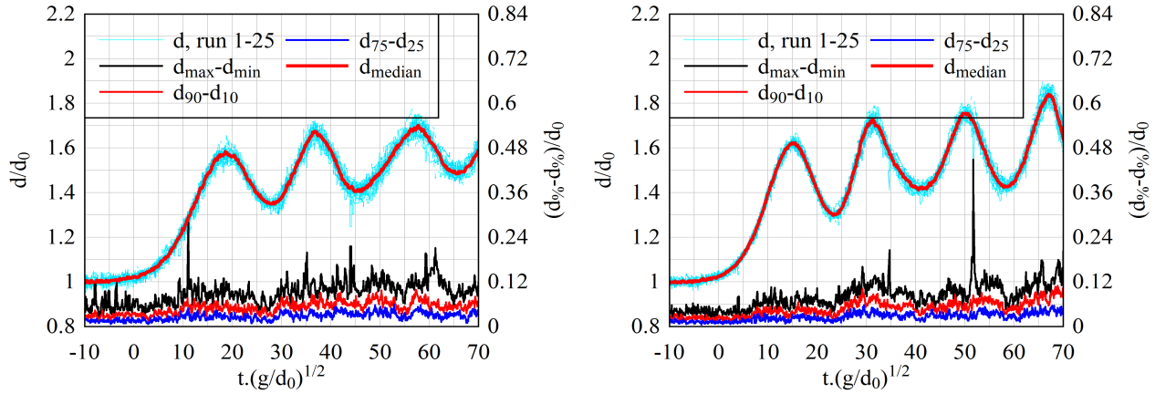
(a) Q = 0.036 \text{ m}^3 \cdot \text{s}^{-1} , d_0 = 0.086 \text{ m} , Fr = 1.29 , h_g = 43 \text{ mm} (b) Q = 0.055 \text{ m}^3 \cdot \text{s}^{-1} , d_0 = 0.111 \text{ m} , Fr = 1.31 , h_g = 62 \text{ mm}
