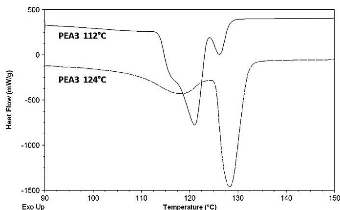
Figure 13.2. DSC curves of PEA3 sample annealed from the melt at 112^{\circ}\text{C} or 124^{\circ}\text{C} for 30 minutes- 10^{\circ}\text{C}\cdot\text{min}^{-1} .
