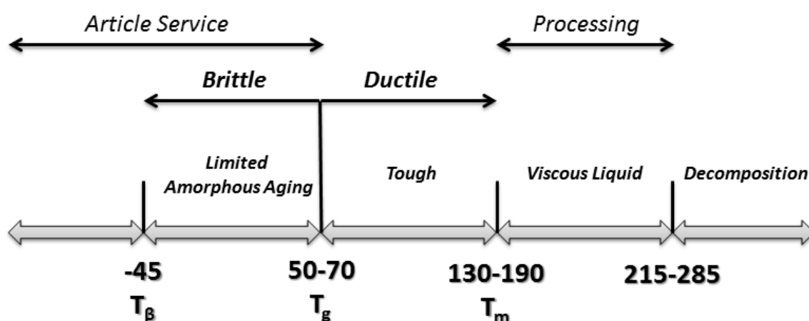
Figure 4.1. Metastable states of high molecular weight semicrystalline PLA
