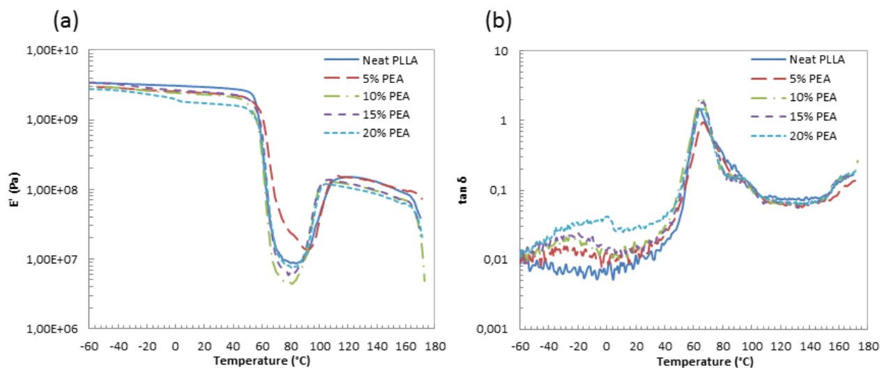
Figure 30.2. (a) Storage modulus and (b) \tan \delta as a function of temperature for neat PLLA and the blends.
