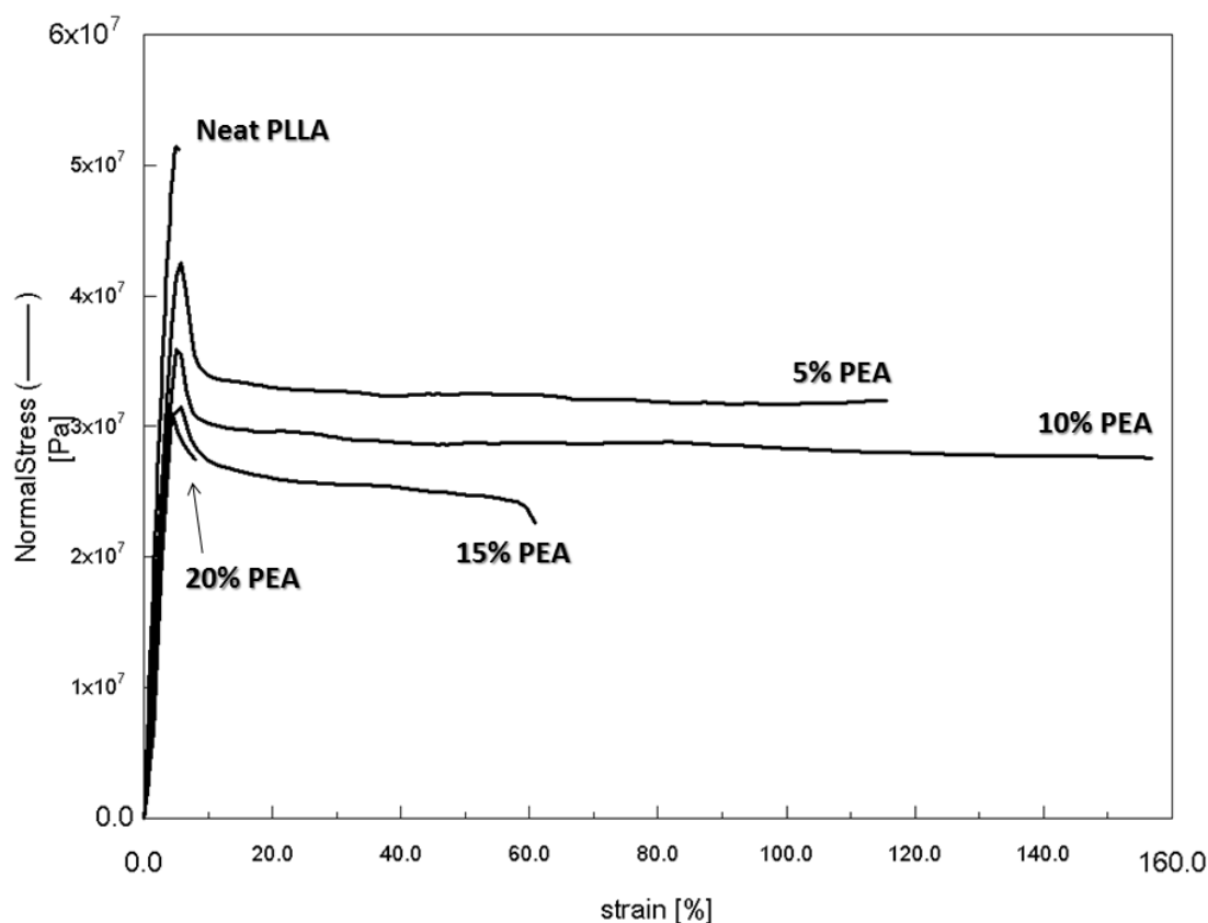
Figure 31.2. Stress-strain curves for neat PLLA and the blends. v=10 \text{ mm.min}^{-1} .
