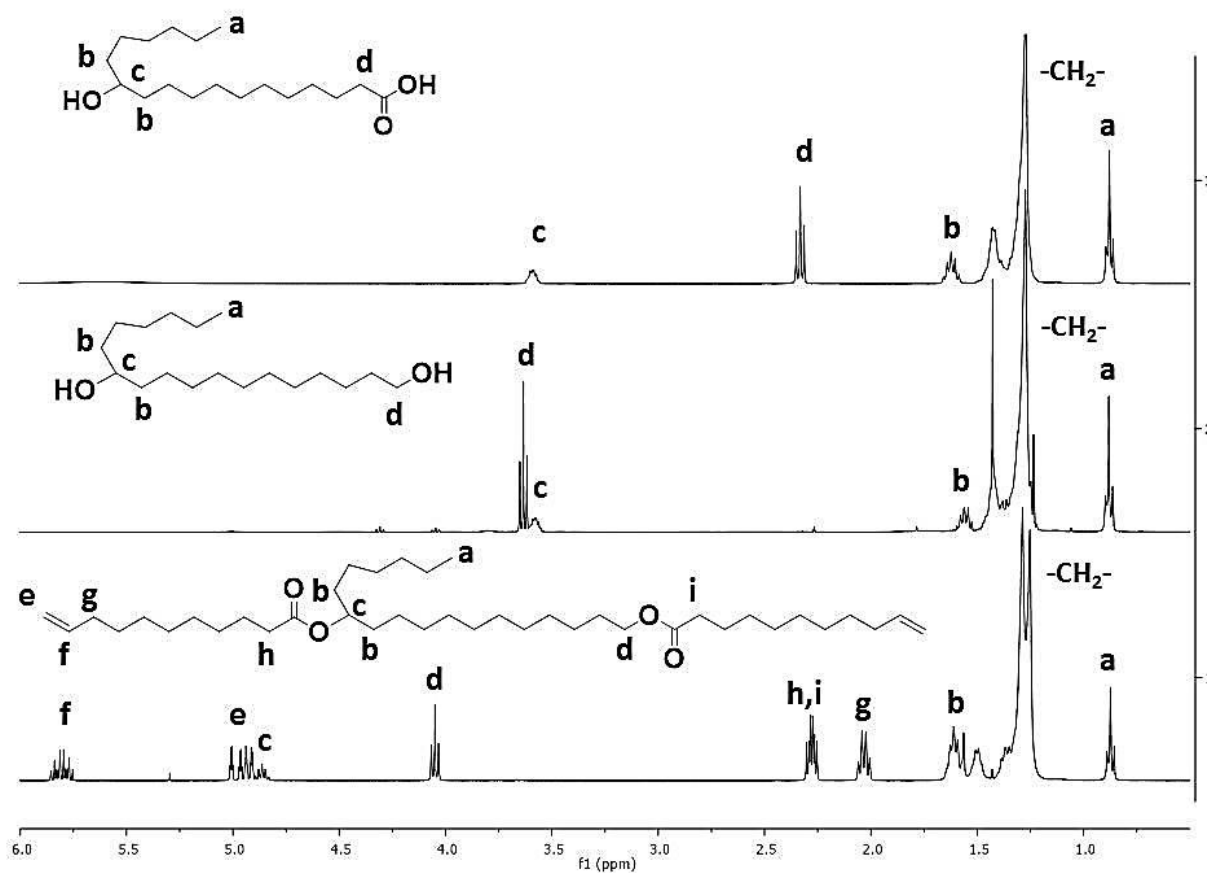
Figure 23.5. ^1\text{H-NMR} stacked spectra of 12-hydroxystearic acid, 12-hydroxystearyl alcohol and branched \alpha,\omega -diene in \text{CDCl}_3 .
