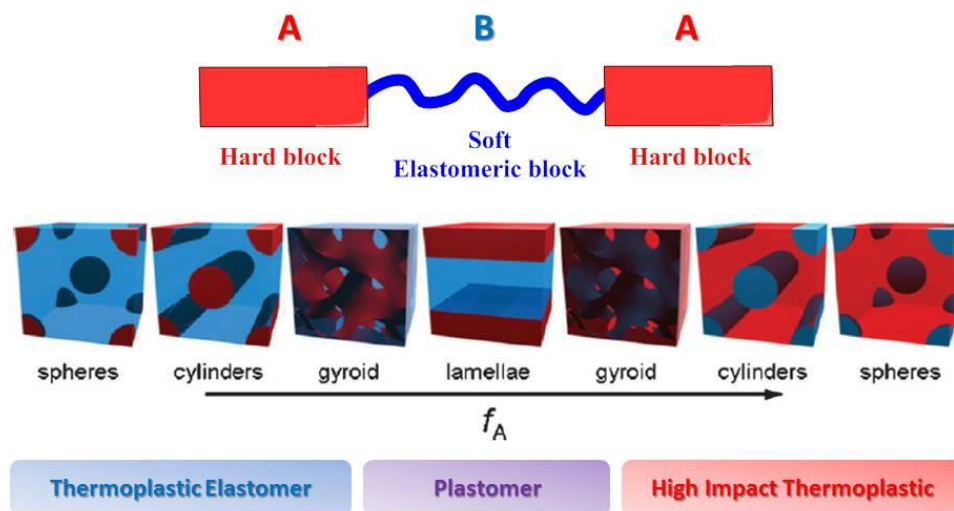
Figure 13.1. Morphologies and mechanical behaviors of block copolymers as a function of the composition
