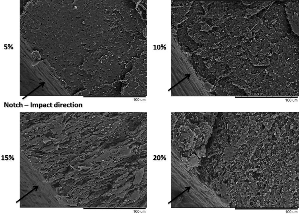
Figure 33.2. SEM images of the impact fractured surfaces of the blends. Images were taken close to the notch.
