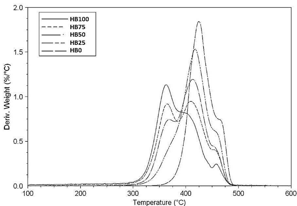
Figure 27.5. TGA derivative curves of the saturated polyesters. 10°C.min -1 .
