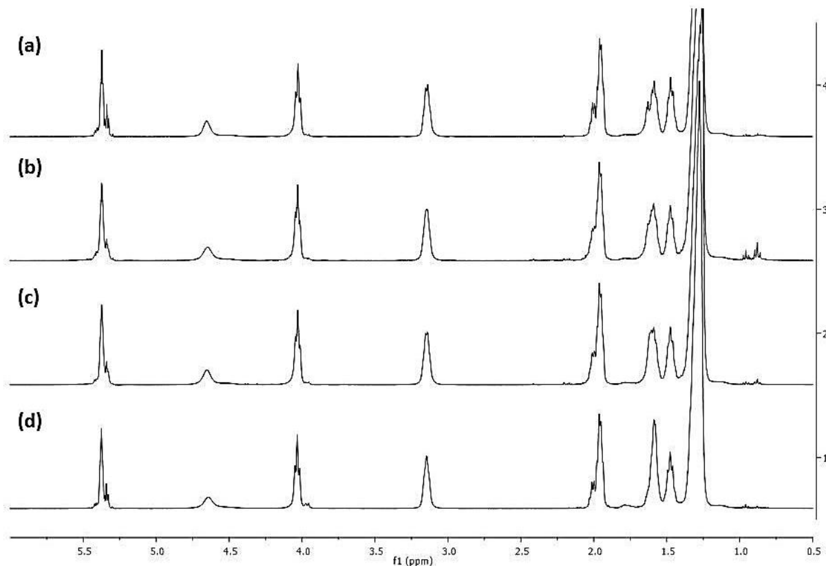
Figure 8.5. 1 H-NMR stacked spectra of the polyurethanes synthesized in bulk from (a) C1, (b) C2, (c) C3 and (d) C4. CDCl 3 .
