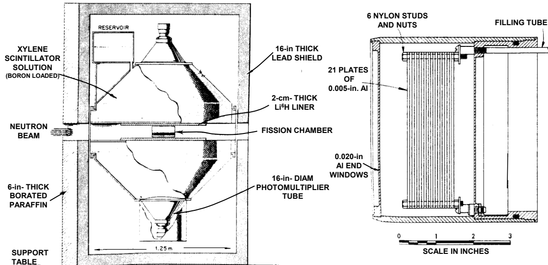
Figure 3.2: Schematic view of the experimental set-up, liquid-scintillator tank and fission chamber. Detail of the ^{233}\text{U} fission ionisation chamber on the right [Weston 68].
