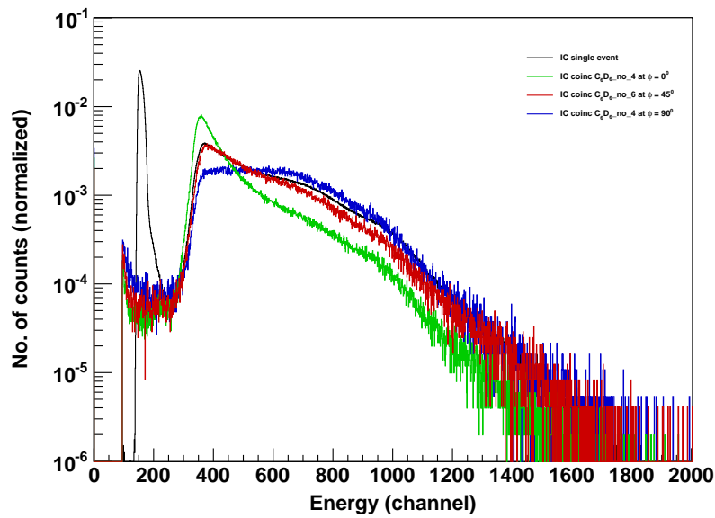
Figure 5.22: Spectra of IC in single event and in coincidence with three C_6D_6 scintillators, placed in different geometries. The IC spectra is normalized to the same number of FF. The coincidence spectrum are obtained in coincidence with C_6D_6\_4 in position 1 at \phi = 0 , and in position 2 at \phi = 90^\circ . The same coincidence was obtained with C_6D_6\_6 in position 2 at \phi = 45^\circ .
