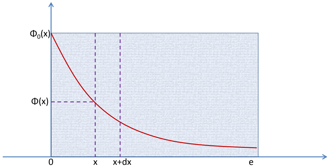
Figure 4.6: Neutron flux attenuation versus thickness e (in cm) of attenuating material.
