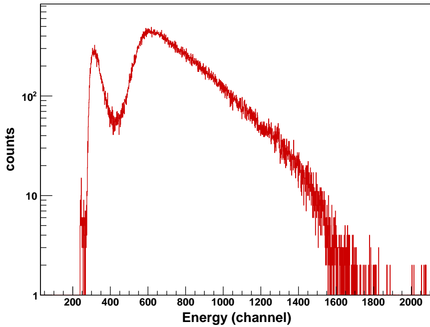
Figure 5.29: The pulse height fission spectra of the IC obtained with ^{233}\text{U} sample in thermalized neutrons at AIFIRA facility.
