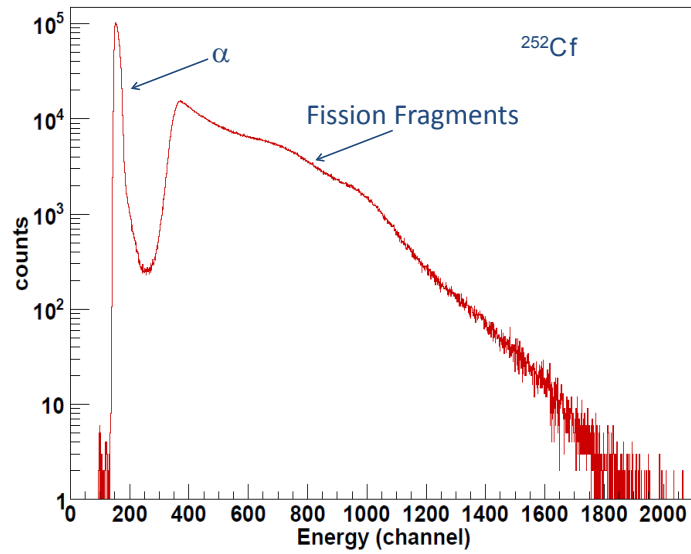
Figure 5.2: Pulse height distribution from the ionisation chamber measurement of ^{252}\text{Cf} spontaneous source. The peak at the channel 150 is caused by alpha particles, while the broad distribution above 300 channel is caused by fission fragments.
