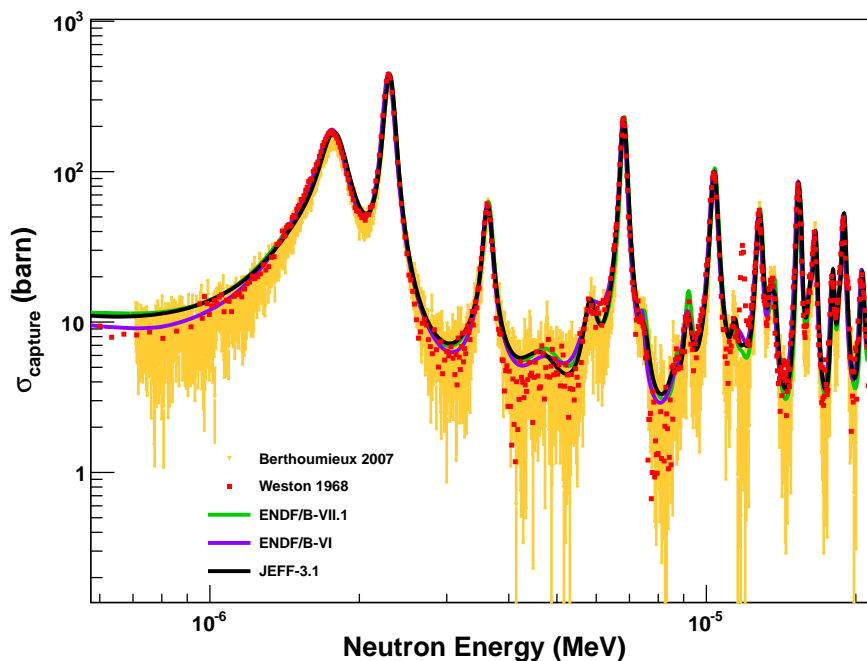
Figure 3.11: Comparison between the only existing experimental data of neutron capture cross-section of ^{233}\text{U} [Berthoumieux 07, Weston 68] and the evaluation of nuclear data libraries ENDF/B-VII.1, ENDF/B-VI and JEFF-3.1 in the energy range from 0.6\text{eV} to 20\text{eV} .
