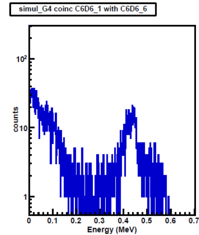
Figure 5.7: Simulated coincidence spectra with ^{137}\text{Cs} point like source ( 10^7 particles). The energy of the \gamma -ray is 661 keV and the corresponding Compton edge is 477 keV.
