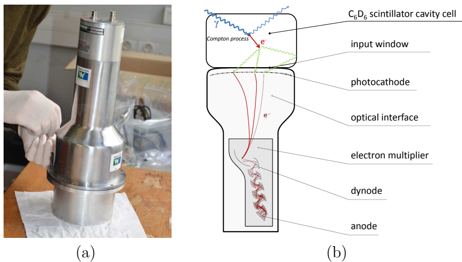
Figure 4.11: (a) Picture of one C_6D_6 detector used in our experiment: a module consists of a C_6D_6 cavity cell, a photomultiplier tube and a voltage divider. (b) Generation of the electronic signal in the anode for a Compton event.
