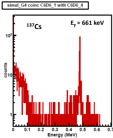
Figure 5.7: Simulated coincidence spectra with ^{137}\text{Cs} point like source ( 10^7 particles). The energy of the \gamma -ray is 661 keV and the corresponding Compton edge is 477 keV.
