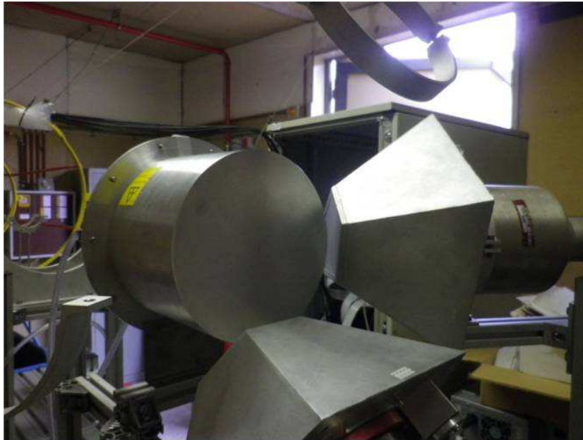
Figure 5.33: Picture of the experimental set-up for PSD response function prompt fission neutrons and \gamma -ray discrimination at Gelina.
