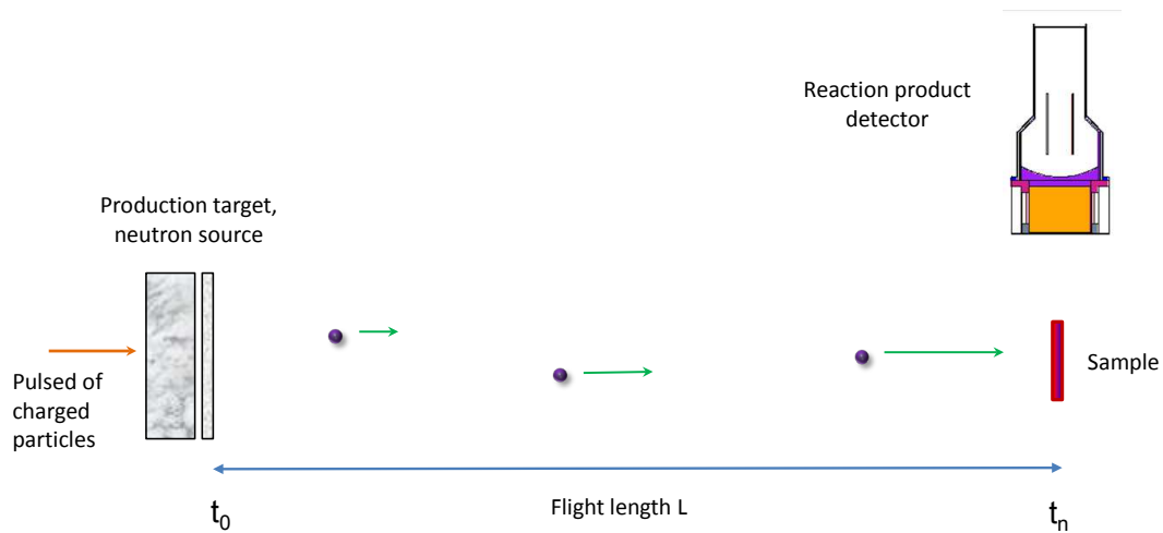
Figure 4.4: The principle of time-of-flight method
