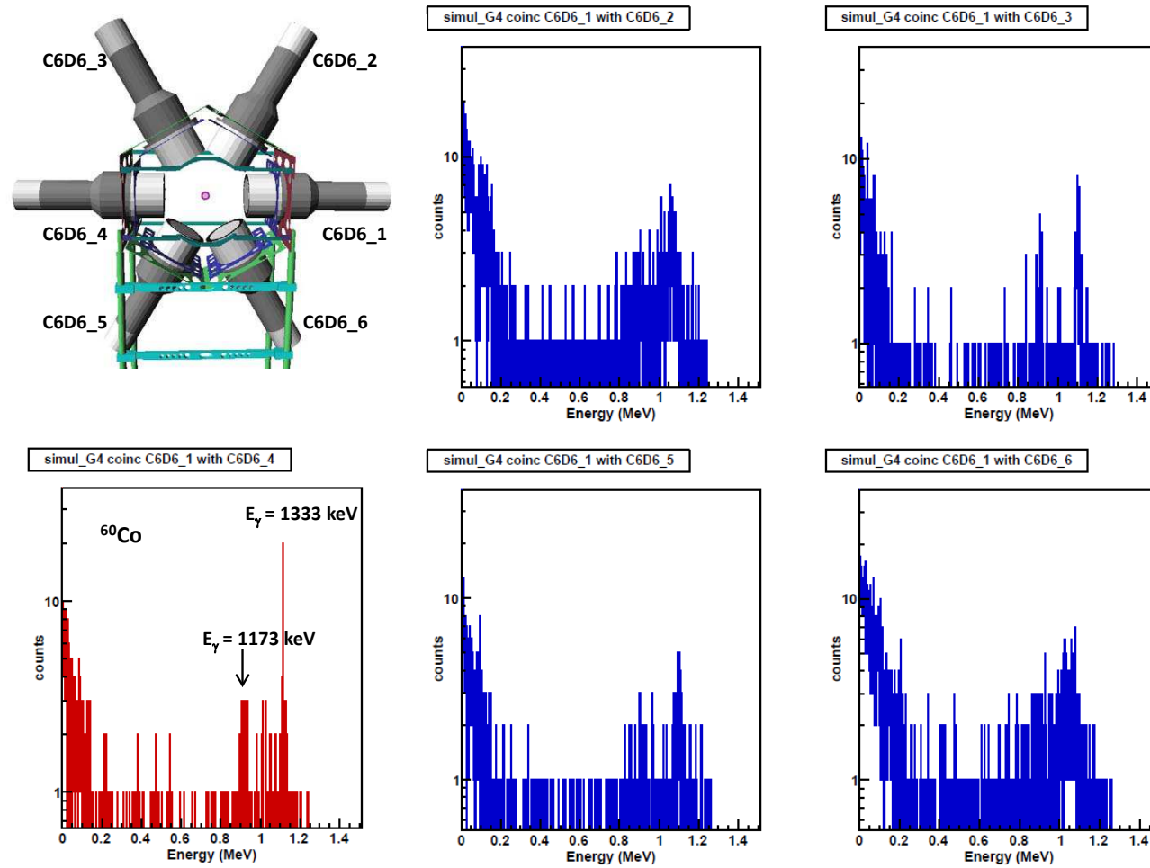
Figure 5.8: Simulated coincidence spectra with ^{60}\text{Co} point like source ( 10^7 particles). The energy of the \gamma -rays are 1173 keV and 1333 keV and the corresponding Compton edges are 963 keV and 1119 keV respectively.
