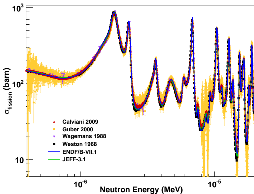
Figure 3.5: Evaluated ENDF/B-VII.1 and JEFF-3.1 ^{233}\text{U}(n, f) cross-section in the RRR compared with four experimental data [Calviani 09, Guber 01, Wagemans 88, Weston 68] obtained by different methods and experimental set-up conditions, at different neutron facilities.
