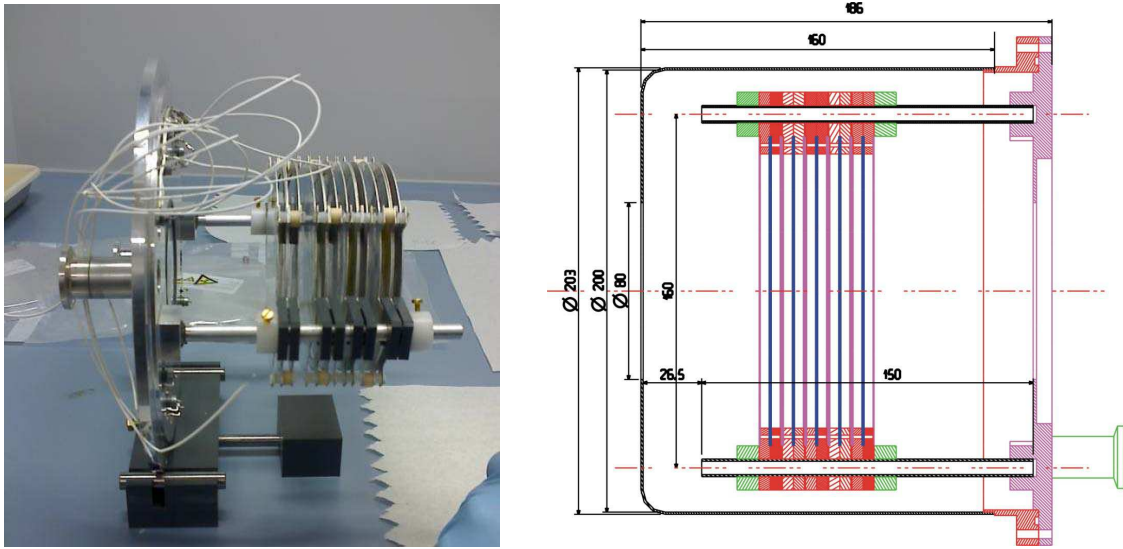
Figure 4.7: Photo of the inside of the ionisation chamber with three ^{233}\text{U} samples taken during the assembly. A detailed schematic view of the ionisation chamber on the right.
