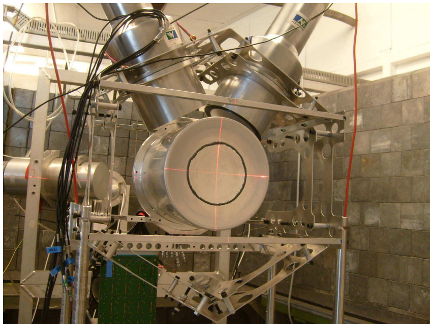
Figure 5.11: Experimental set-up used at Gelina facility for the preliminary test experiment using different ^{233}\text{U} targets in the IC and only two \text{C}_6\text{D}_6 detectors
