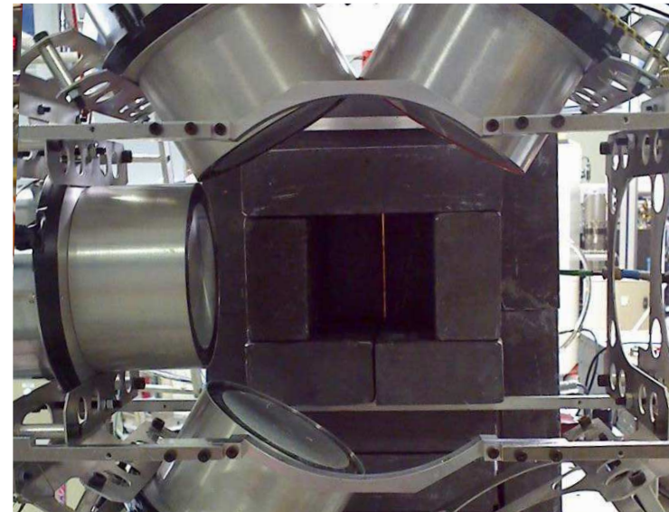
Figure 5.32: Experimental set-up used for the efficiency of the IC measurement using ^{233}\text{U} target at AIFIRA facility at CENBG.
