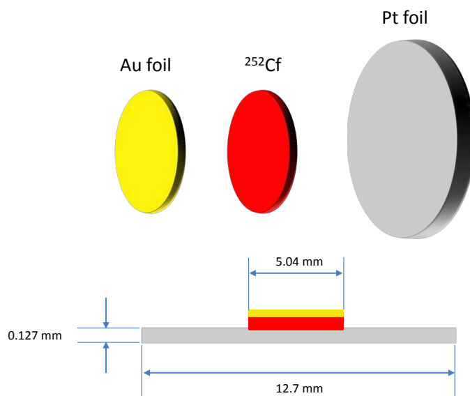
Figure 5.1: The ^{252}\text{Cf} spontaneous fission sample technical details.
