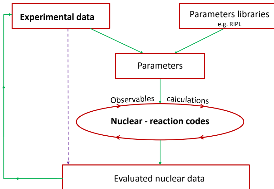
Figure 1.6: Conceptual scheme of different steps between experimental nuclear data, model parameters and evaluated nuclear data.
