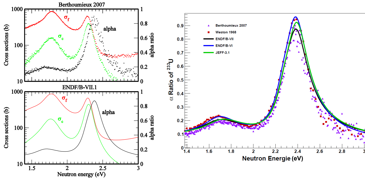
Figure 3.16: On the left it is shown the ^{233}\text{U}(n, f) and ^{233}\text{U}(n, \gamma) cross sections with the associated \alpha ratio determined using Berthoumieux data (left up) and ENDF/B-VII.1 data (left down) for the first two resonances. On the right a comparison between \alpha ratio derived from different experimental and evaluated data of ^{233}\text{U} for the first two resonances. The lower \alpha ratio value from the results of Berthoumieux may be attributed to the better energy resolution of the n_TOF facility compared to the RPI facility according to [Berthoumieux 07].
