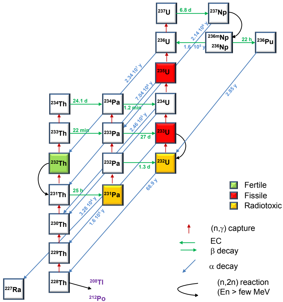
Figure 1.3: Nuclear transformations in ^{232}\text{Th}/^{233}\text{U} cycle [Abbondanno 01].
