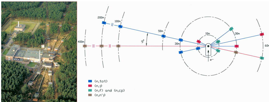
Figure 4.1: Gelina site on the left picture. A schematic view of the flight paths on the right. Neutron measurements can be performed simultaneously at 12 flight paths with lengths ranging from 10 up to 400 m, located in radial direction from the target [Mondelaers 06]. Many types of neutron cross section measurements are possible: transmission experiments, as well as capture, fission, elastic and inelastic cross section experiments.
