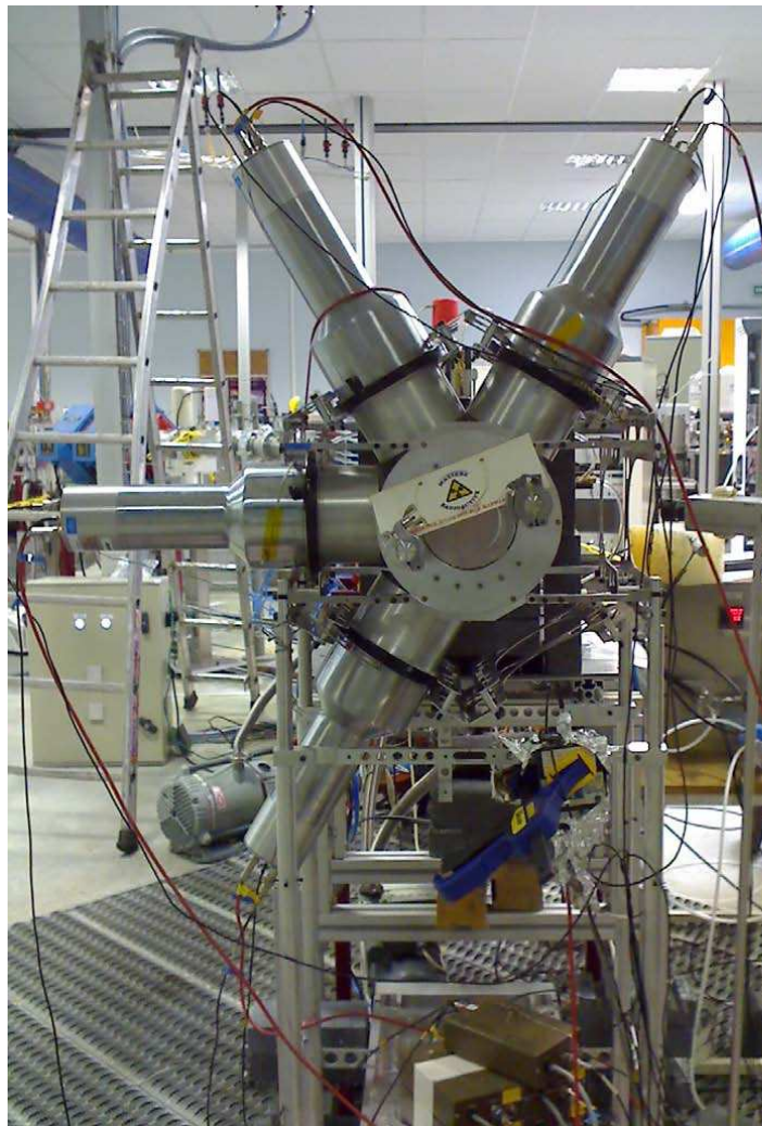
Figure 5.32: Experimental set-up used for the efficiency of the IC measurement using ^{233}\text{U} target at AIFIRA facility at CENBG.
