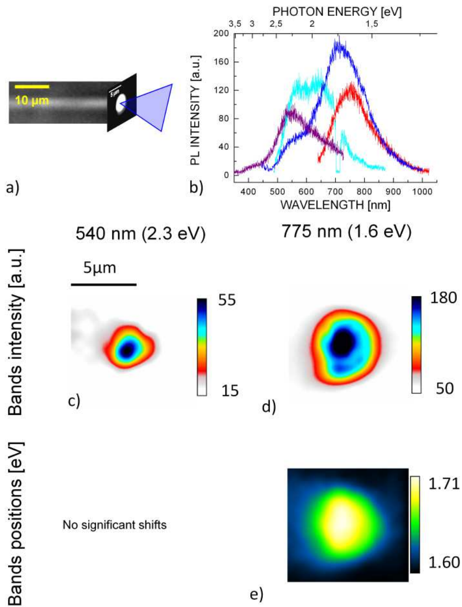
Figure 8.4: a) PCM image of type II-NGN modification in BK7 glass showing schematically the geometry of cross-section map spectroscopy. b) The associated cross-section PL spectra, where color indications of different excitation sources are the same as in Fig. 8.2. Bottom: 2D spectral maps of c) the 540 nm band. d) The 775 nm band intensities and e) 775 nm band shift upon excitation with HeCd (442 nm) light.
