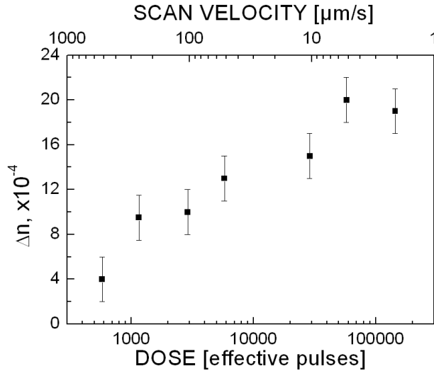
Figure 5.11: Refractive index changes induced for type I waveguides written with different velocities of the translation stage. Waveguides were fabricated with 1 \mu\text{J} laser pulses following at the repetition rate of 10 kHz, focused by a \text{NA}_{eff}=0.3 objective.
