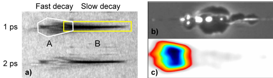
Figure 6.10: a) Time resolved OTM images of fused silica irradiated taken at 1 and 2 ps after irradiation ( E=4.3 \mu\text{J} , 150 fs, NA_{eff}=0.4 ). The images show strong electron absorption due to the generated free electrons. It allows to divide the zone of electron generation in two parts: A (white hexagon) with fast electron relaxation ( <1 ps) and part B (yellow rectangle) with slow electron relaxation ( \sim 100 ps), where permanent refractive index changes are taking place [Mau10]. For 30 \mu\text{J} , 150 fs pulses b) PCM image of permanent refractive index changes and c) NBOHC generation map show a separation corresponding to the division in zones of fast and slow relaxation.
