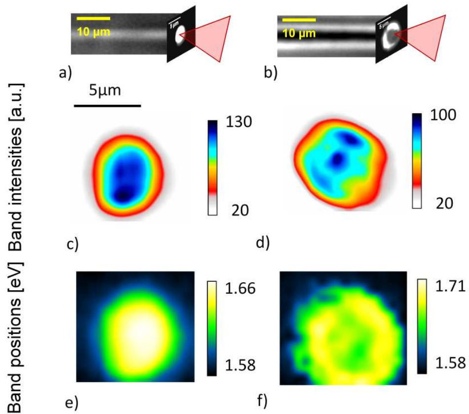
Figure 8.6: PCM image of a) type II-NG and b) type II-G modifications in BK7 glass showing schematically the geometry of cross-section map spectroscopy. Bottom: 2D spectral maps of c), d) the 775 nm band intensities and e), f) the 775 nm band shifts upon excitation with HeNe (633 nm) light of the type II-NG and the type II-G modifications, respectively.
