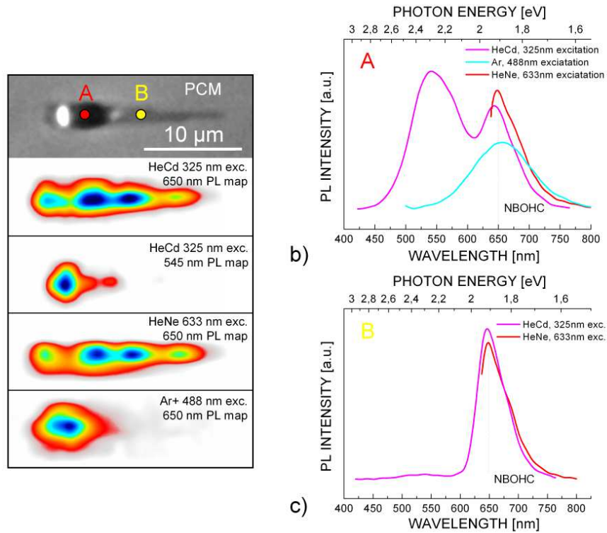
Figure 6.7: a) PCM image of static traces in fused silica irradiated by N=20 pulses with an energy of E=1 \mu\text{J} focused by the NA_{eff}=0.4 objective, and the corresponding 2D spectral maps of different PL bands arising under 633, 488 and 325 nm excitation, notably the 545 nm and 650 nm PL bands. Typical PL spectra: b) spectra collected from the region looking white and dark black (denoted as A) on the PCM image of the trace. c) Spectra collected from the filament-like region looking gray (denoted as B) of the same trace under 633 and 325 nm excitation. PL signal from the 488 nm excitation is negligible and, thus, not shown.
