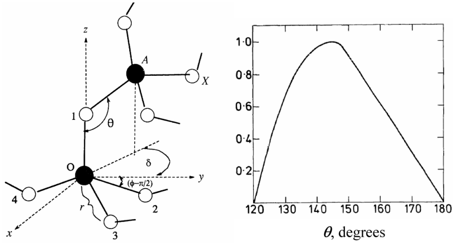
Figure 2.1: a) Segment of \text{SiO}_2 network presenting its local order parameters: the length of the Si–O bond r , interbonding Si–O–Si angle \theta , and intertetrahedral tilt angle \delta [BGME93]. b) Statistical distribution of the Si–O–Si bonding angles in amorphous \text{SiO}_2 , as determined from X-rays diffraction data by [MW69].
