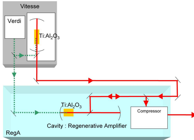
Figure 4.2: Schematic representation of a regeneratively amplified femtosecond laser system from Coherent. The green arrow represents the pump beam and the red arrow the seed and amplified femtosecond pulses.
