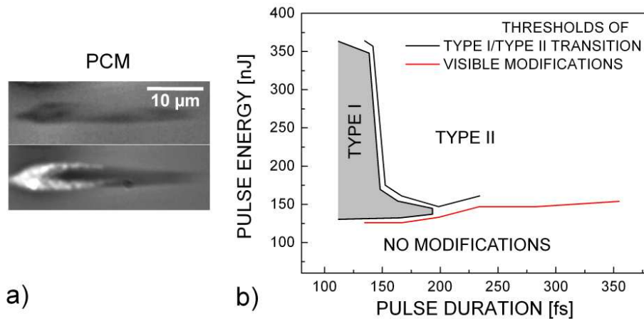
Figure 5.3: a) Static traces of N=50000 1 \mu\text{J} focused by OB2 objective with \text{NA}_{\text{eff}}=0.3 for pulse durations of 140 (type I, top) and 150 fs (type II, bottom) b) Dependence of the produced modification threshold as a function of pulse duration for moderately focused laser pulses. Writing window for type I positive smooth refractive index changes (gray filling) is situated between energetic thresholds of visible modification (red line) and type I/II transition (black line) produced by N=50000 pulses in static conditions.
