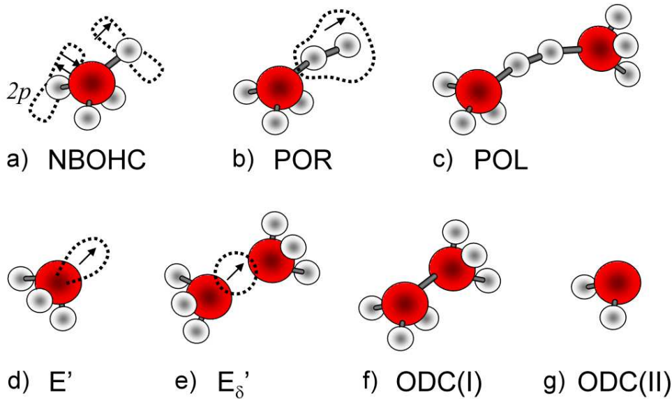
Figure 2.6: Structural models for oxygen excess defects: a) non-bridging oxygen hole center, NBOHC, b) peroxy radical, POR, c) peroxy linkage, POL; and defects with deficit of oxygen: d) E' and e) E'_\delta centers, f) relaxed oxygen vacancy, ODC(I) and g) divalent silicon, ODC(II). Spin states are indicated by the arrows.
