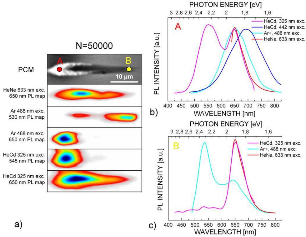
Figure 6.9: PL spectral maps measured for type II static multiple shot damage traces, produced by N=50000 , E=1.5 \mu\text{J} , \tau_p=150 \text{ fs} pulses focused by an \text{NA}_{\text{eff}}=0.3 objective. a) PCM image of the laser-induced modification and spectral maps of the associated PL bands for 633, 488 and 325 nm excitation, notably 530, 545 and 650 nm bands. b) and c) Arbitrary normalized PL spectra collected in the regions marked A and B on the PCM image, corresponded to the birefringent region and region of filament-like propagation respectively under 633 (red line), 488 (blue line), 442 (dark blue line) and 325 nm (magenta line) excitation sources.
