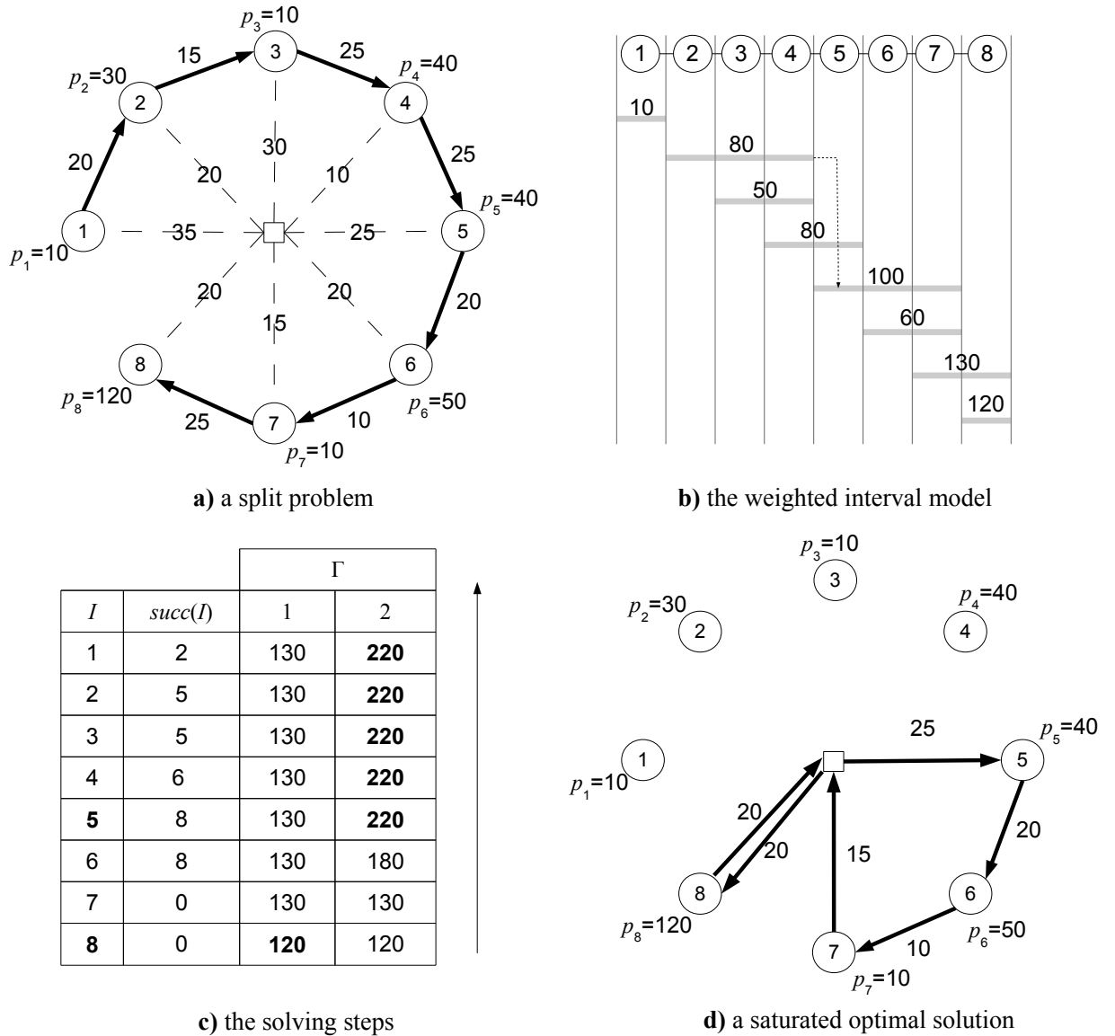
Figure 3.1: The new evaluation process for the same split problem described in [25] with 8 customers, m = 2 and L = 70 .
