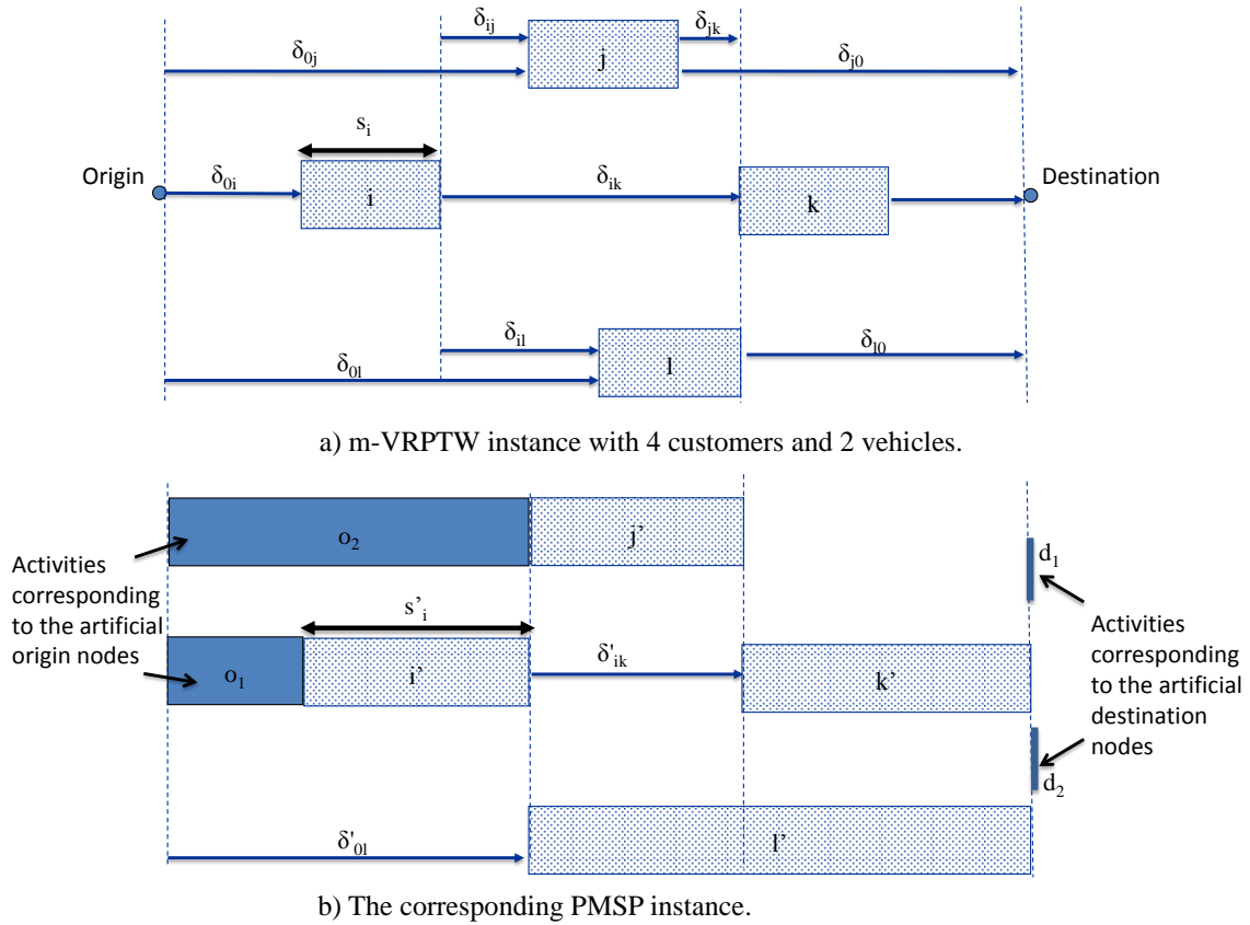
Figure 5.3: An example of m-VRPTW instance related to PMSP instance.
