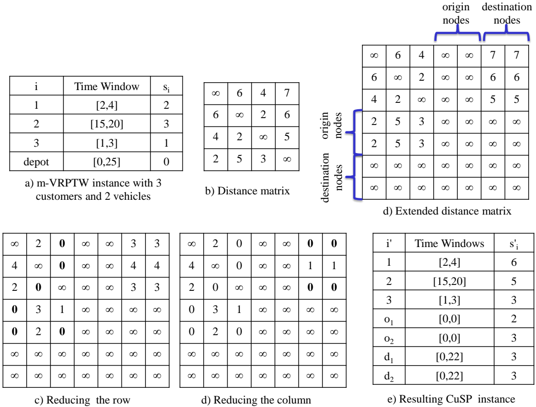
Figure 5.4: An example of reducing the rows and the columns of the extended distance matrix.
