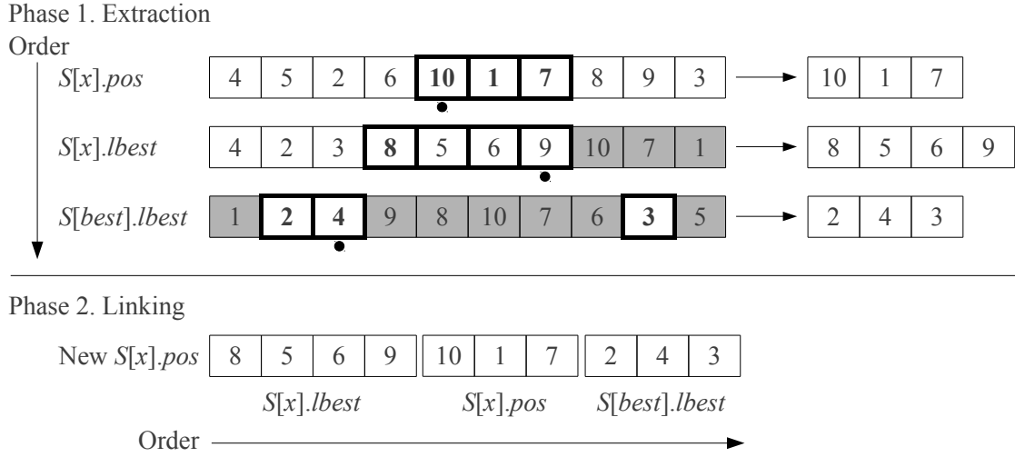
Figure 3.2: An example of position update for an arbitrary instance of ten customers. Black dots represent random generated locations r and shaded boxes represent marked customers from M during Phase 1.
