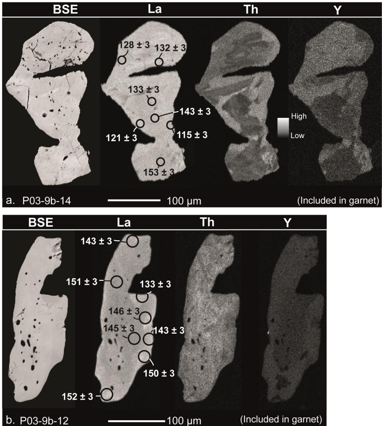
Figure 7: BSE images and La, Th, and Y X-ray maps of M1i monazites included in garnet from Sidironero (P03-9 sample). Circles show the location of the LA-ICPMS pits (11 \mu m) and their corresponding ^{208}\text{Pb}/^{232}\text{Th} ages ( 2\sigma level).
