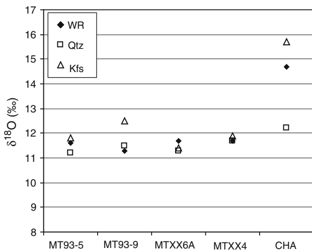
Fig. 11 Oxygen isotope composition of quartz, feldspar and whole rock from Montasset (MT93-5, MT93-9, MTXX6A, MTXX4) and Charron (CHA). The graph highlights isotopic disequilibrium in all samples
