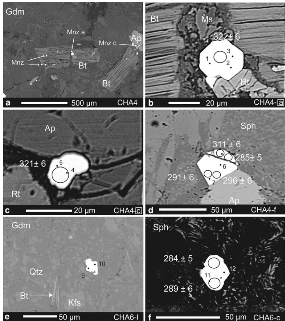
Fig. 5 BSE images of Charron monazites. Monazite is associated with apatite ( a, c, d ) and biotite ( a, b ) is in the groundmass ( e ), or is in spherulite ( f ). It is euhedral ( b, d, f ) to sub-euhedral ( c, e ). Numbers correspond to microprobe analyses reported in Table 3, and circles show the location of LA-ICPMS pits (7 \mu\text{m} ) and their corresponding ^{208}\text{Pb}/^{232}\text{Th} ages in Ma ( 2\sigma level). Ap apatite, Bt biotite, Gdm groundmass, Kfs K-feldspar, Mnz monazite, Ms muscovite, Pl plagioclase, Qtz quartz, Rt rutile, Sph spherulite, CHA Charron microgranite
