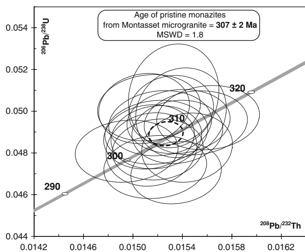
Fig. 8 ^{206}\text{Pb}/^{238}\text{U} versus ^{208}\text{Pb}/^{232}\text{Th} diagram of analyses in pristine monazites from the Montasset microgranite giving a concordant age at 307 \pm 2 Ma
