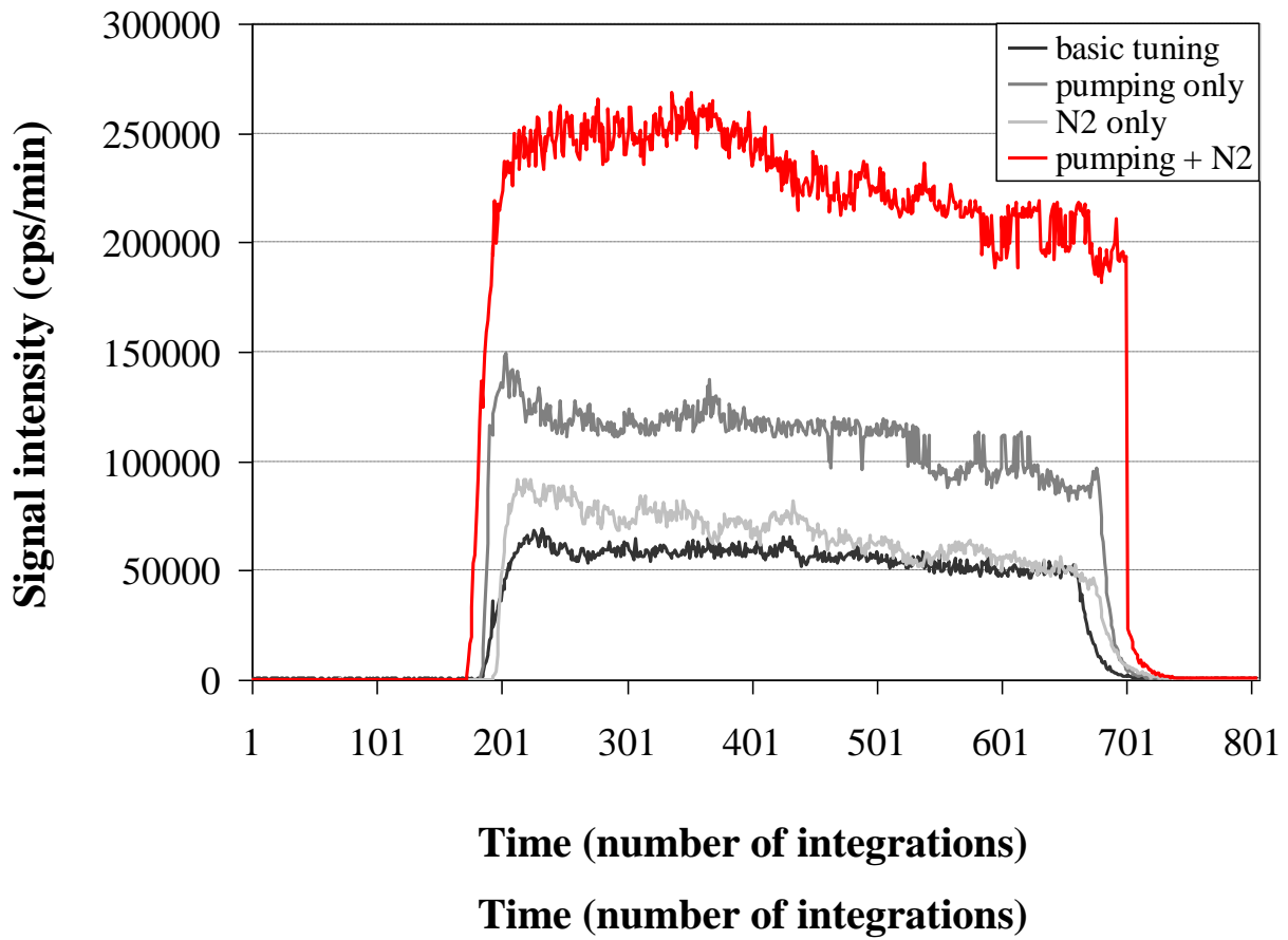
Figure 2: Signal profiles for the 91500 zircon reference material during 60s spot analyses.
