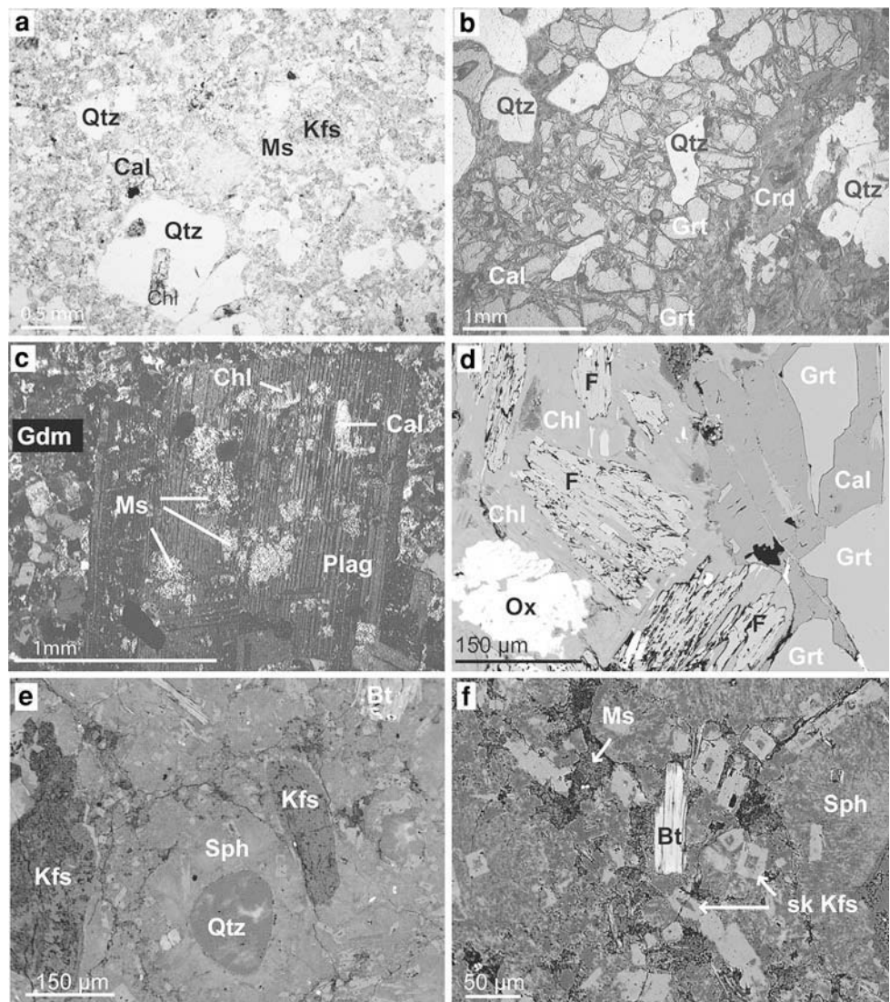
Fig. 2 a–c Photomicrographs and d BSE image of Montasset microgranite. a Porphyric texture of microgranite with phenocrysts of corroded quartz, K-feldspar, chlorite and secondary muscovite. b Garnets strongly fractured in several pieces. Fractures are filled with calcite and sometimes chlorite. c Plurimillimetric plagioclase replaced by calcite and muscovite. d Fluorite replacing chlorite, and calcite filling garnet fractures. e and f Back-scattered electron images of the porphyric Charron microgranite with phenocrysts of K-feldspar, quartz and biotite. In (e) , quartz is surrounded by spherulitic structures, indicating a fast cooling rate. In (f) , K-feldspars are skeletal. Bt biotite, Cal calcite, Chl chlorite, F fluorite, Grt garnet, Kfs K-feldspar, Mnz monazite, Ms muscovite, Ox iron oxide, Qtz quartz, Gdm groundmass, Th Th-silicate, sk Kfs skeletal K-feldspars, Sph spherulite
