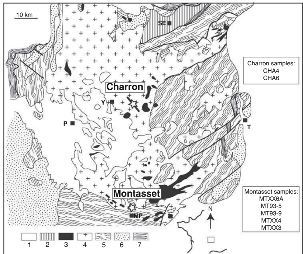
Fig. 1 Geologic map of Velay with locations of the Montasset and Charron microgranites (the stars in the south and middle of the map, respectively). MP Montpezat-sous-Bauzon, P Le Puy, SE Saint-Etienne, T Tournon, Y Yssingeaux. (1) Post-Palaeozoic sediments and volcanics, (2) Stephanian basin, (3) post-anatectic granites, (4) Velay granite, (5) Lower Gneiss Unit, (6) other granites, (7) Upper Gneiss Unit (Map modified after Montel et al. 2002b)
