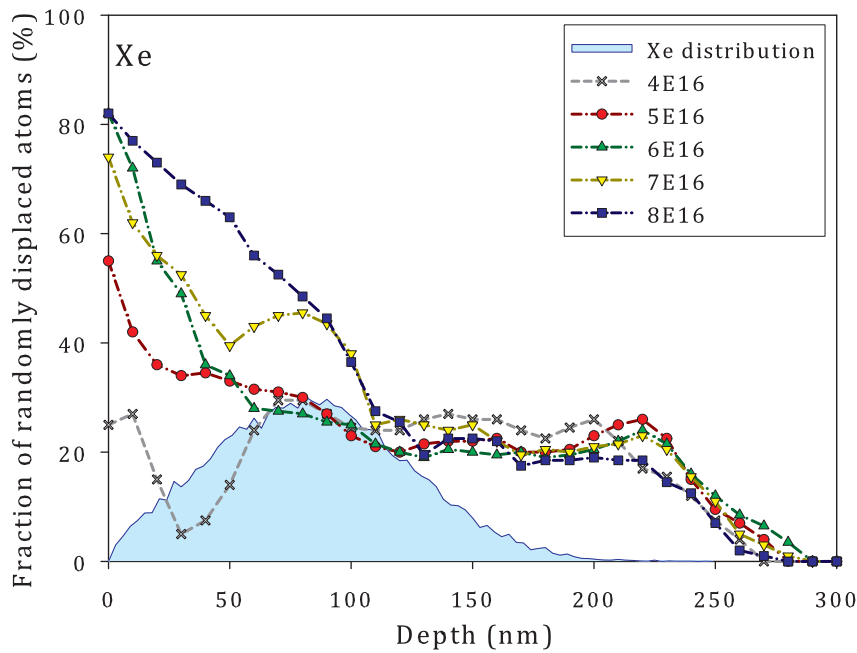
Figure 4-12: Distributions of RDA versus depth measured for Xe^- implanted UO_2 crystal at very high fluence (corresponding to over 5 at. % of implanted Xe in the matrix) derived from simulations. BC is parameterized by L = 5 \text{ nm} and \eta = 1.5^\circ . Fluences are measured in the unit of cm^{-2} . Xe implantation profile calculated by SRIM (represented by filled area) is plotted in arbitrary unit.
