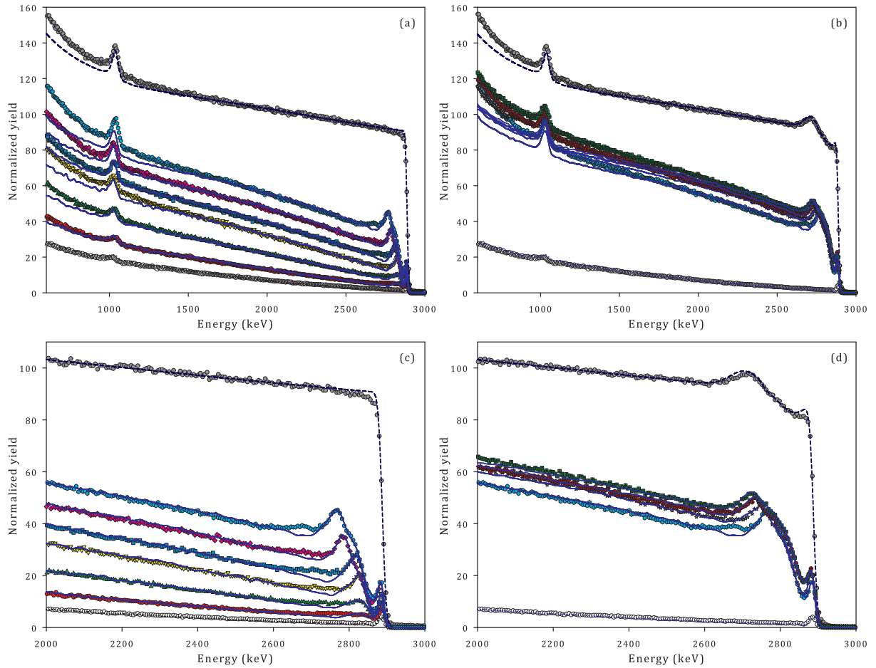
Figure 4-8: Best MC simulations to RBS/C spectra recorded for Ce-implanted UO_2 crystal at low (a) and high (b) fluences. The zooms on high energy part are shown on figure (c) and (d) respectively. Dashed lines and dotted lines denote the best fits to random and axial virgin spectra. Solid lines denote best MC simulations to axial aligned spectra recorded for irradiated crystal. Experimental channelling spectra are plotted in symbols for fluences of \Phi = 2 \times 10^{14}\text{ cm}^{-2} (red circle), 7 \times 10^{14}\text{ cm}^{-2} (green triangle up), 8 \times 10^{14}\text{ cm}^{-2} (yellow triangle down), 1 \times 10^{15}\text{ cm}^{-2} (violet square), 2.5 \times 10^{15}\text{ cm}^{-2} (pink diamond), 5 \times 10^{15}\text{ cm}^{-2} (cyan hexagon), 1 \times 10^{16}\text{ cm}^{-2} (gray star), 3 \times 10^{16}\text{ cm}^{-2} (red crossed-circle) and 4 \times 10^{16}\text{ cm}^{-2} (green crossed-square). Fits were performed assuming L = 5\text{ nm} and \eta = 1.5^\circ .
