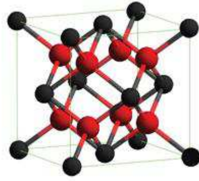
Figure 1-1: Uranium dioxide crystal with uranium atoms located at fcc positions (black) and oxygen atoms located at tetrahedral positions (red).
