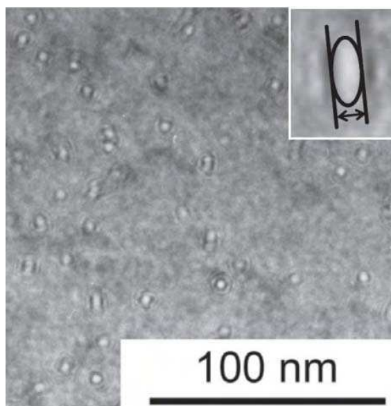
Figure 1-8: Typical images of ion tracks in UO_2 under irradiation with 210 MeV Xe^{14+} ions to fluence of 5 \times 10^{11} cm -2 at room temperature [69].
