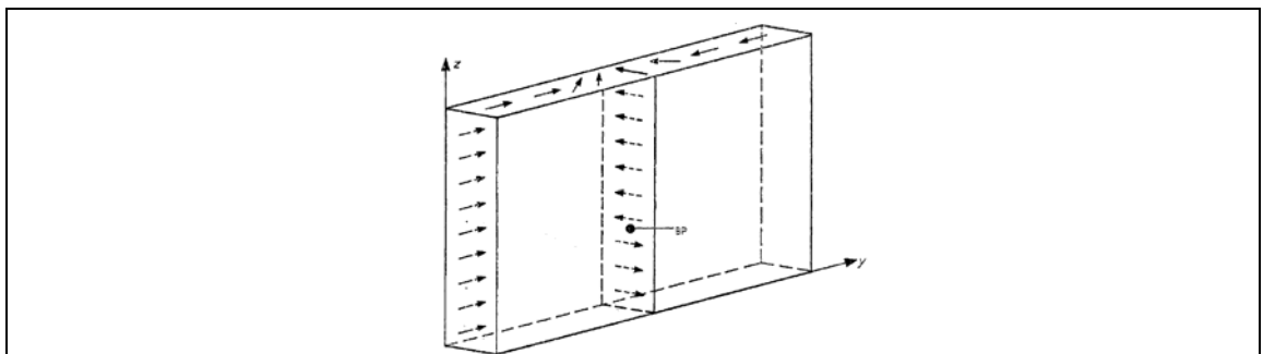
Fig. 1.3: The figure shows a section of a 180^\circ Bloch wall containing a vertical Bloch line (BL) in the centre. The magnetization directions indicated are those of the centre of the wall. The Bloch line carries a Bloch point (BP).
