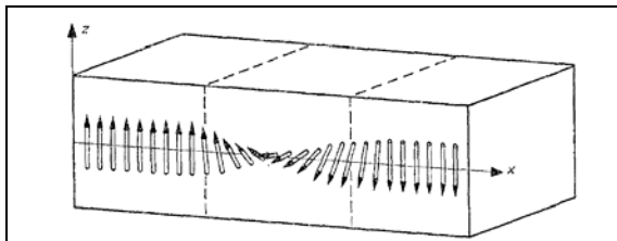
Fig. 1.1: Structure of a Bloch wall in a uniaxial crystal. The magnetization vector remains always normal to the x direction. [LEE80]
