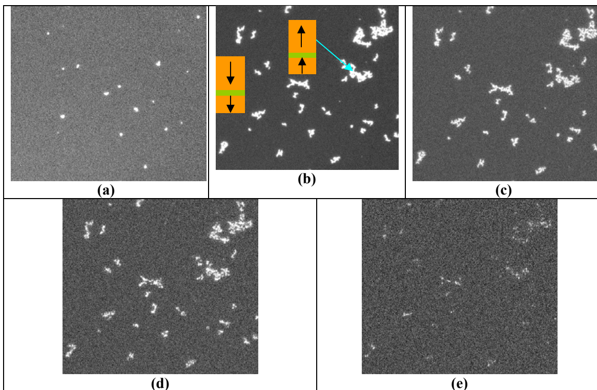
Fig. 5.9: PMOKE images for magnetic behaviors of the hard layer.
