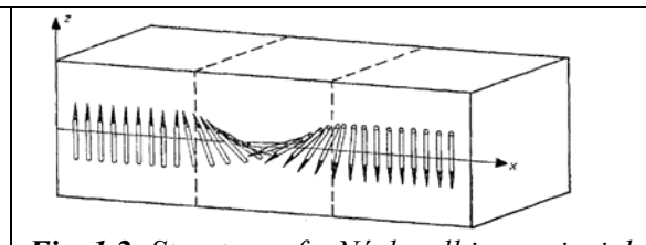
Fig. 1.2: Structure of a Néel wall in a uniaxial crystal. The magnetization vector remains always parallel to the xz plane. [LEE80]
