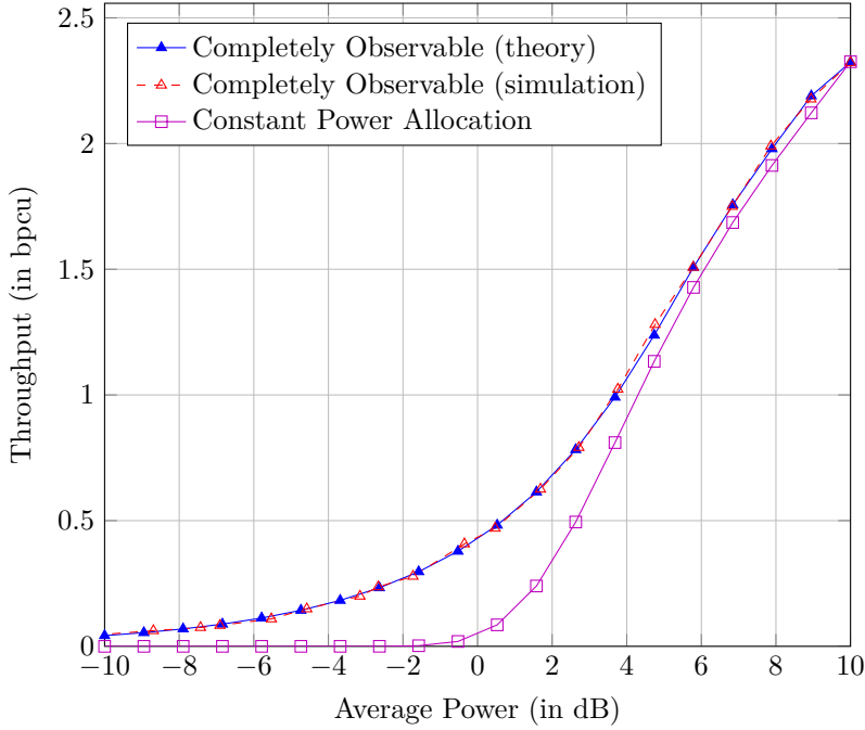
Figure 3.6 – Comparison of the throughput of constant power allocation and variable power allocation as a function of Average SNR for an IR-HARQ protocol. Simulations parameters: N_T = 5 , R = 7 bpcu, \bar{\alpha} = 1 , P_{min} = -10 dBW, P_{max} = 10 dBW, N_I = 16 , and N_a = 64 .
