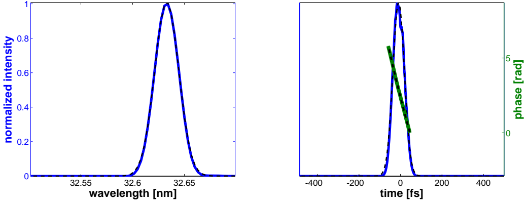
Figure III.14: Perseo output with \chi_1 = 10 \text{ MeV/ps} , \chi_2 = 0 \text{ MeV/ps}^2 and seed non-chirped. Full lines are simulation results and dotted lines their interpolations (Gaussian for the intensity profiles and parabolic for the phase).
