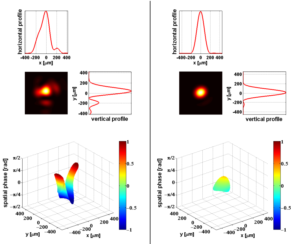
Figure II.30: Propagated electric field: intensity and wavefront at the back focal plane of lens 3, without (left) and with (right) modal filtering. The wavefront is displayed only where the intensity is higher than \frac{1}{e^2} of the maximum intensity.
