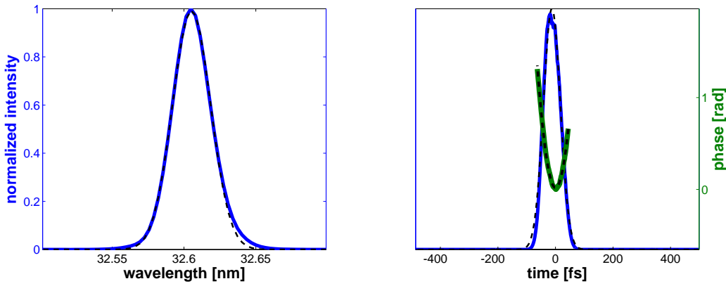
Figure III.16: Perseo output with \chi_2 = 50 \text{ MeV}/ps^2 , \chi_1 = 0 \text{ MeV}/ps and seed non-chirped. Full lines are simulation results and dotted lines their interpolations (Gaussian for the intensity profiles and parabolic for the phase).
