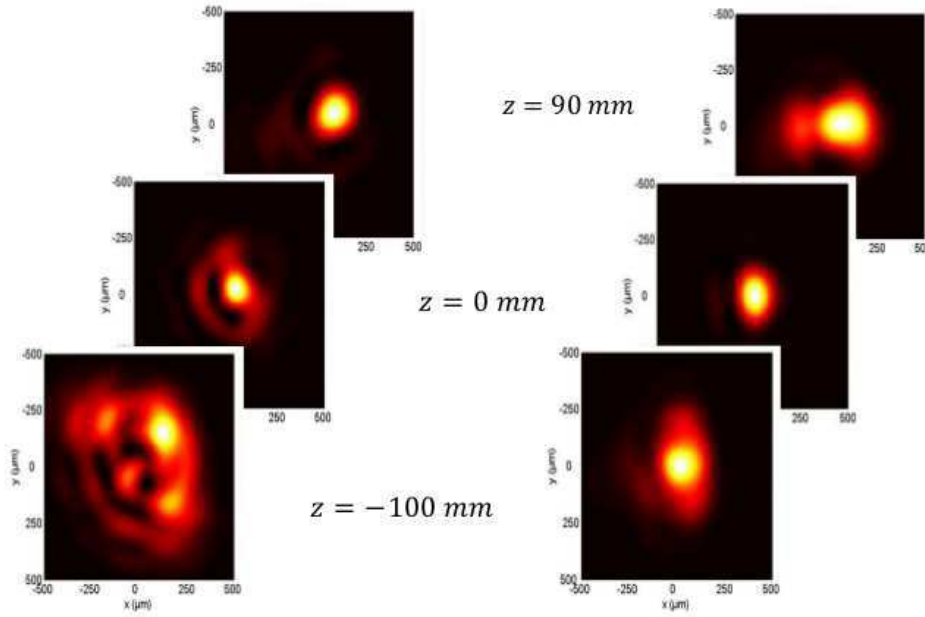
Figure II.31: Intensity of the IR beam before ( z = -100 \text{ mm} ), at ( z = 0 \text{ mm} ) and after ( z = 90 \text{ mm} ) the focus of lens 3, for the non-filtered (a) and filtered (b) beam, according to numerical propagation of the laser field in free space in the paraxial approximation. [Courtesy of D. Gauthier]
