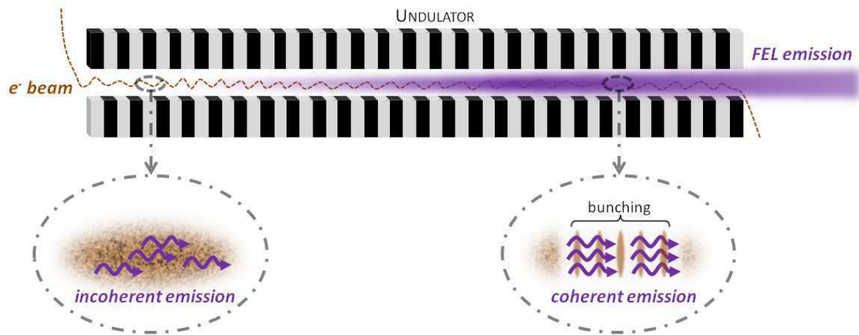
Figure I.8: Basic layout of a SASE FEL.
