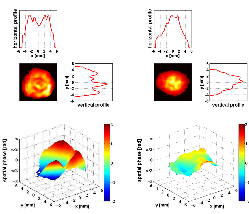
Figure II.29: Shack-Hartmann measurements: intensity and wavefront without (left) and with (right) the fiber. In both cases, the beam mean intensity is similar ( \approx 15 \text{ TW/cm}^2 ).
