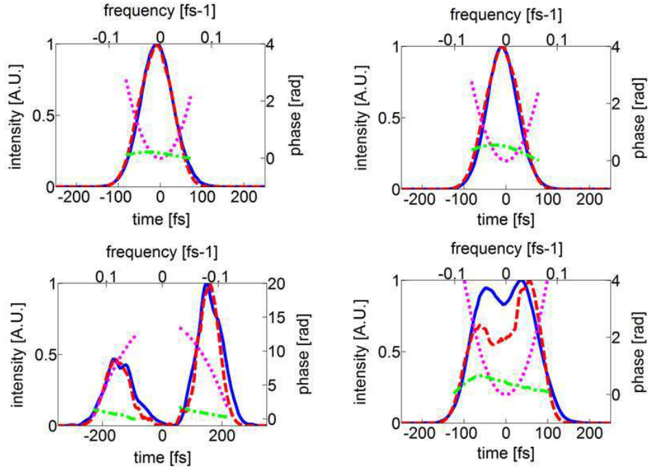
Figure IV.35: Comparison between the temporal (continuous line) and spectral (dashed line) profiles obtained using the numerical code PERSEO: (top left) single pulse, slightly saturated regime with ideal electron beam; (top right) single pulse, slightly saturated regime with quadratic electron-beam energy profile (energy curvature: 5 \text{ MeV}/ps^2 ); (bottom left) double-pulse regime; (bottom right) single pulse, over-saturated regime. In each panel, the temporal scale (bottom axis) is obtained from the spectral one (top axis), using the homothetic transformation given in Eq. IV.9. The phase is separated into the dotted curves representing the quadratic part n\Gamma_i t^2 (with n = 8 ) and the dot-dashed curves correspond to the other phase terms.
