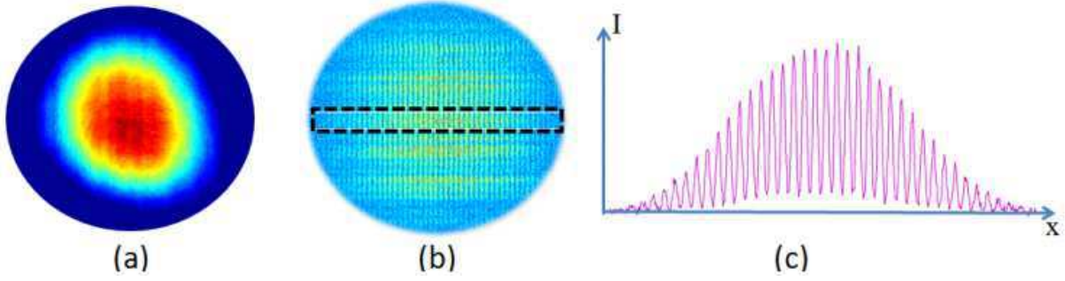
Figure II.3: Typical pattern observed on the CCD without slits inserted (a); pattern with slits separated by d = 1 \text{ mm} , with a region of interest (b); integrated profile of the region of interest (c).
