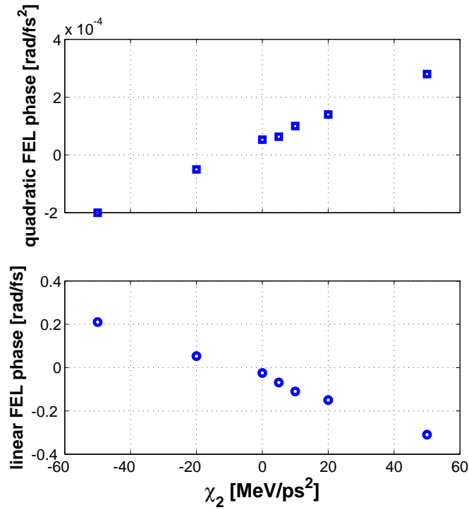
Figure III.18: Quadratic and linear terms of the parabolic interpolation of the temporal phase of the FEL emission as a function of the \chi_2 parameter of the electrons energy, with \chi_1 = 0 \text{ MeV/ps} and seed non-chirped.
