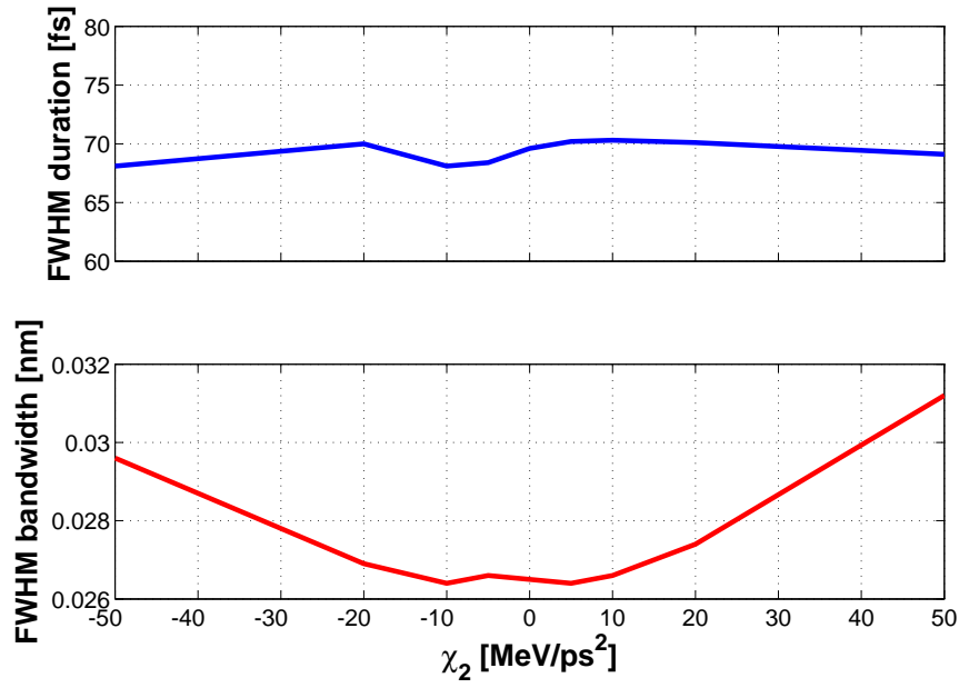
Figure III.17: FWHM duration (top panel) and bandwidth (bottom panel) of the FEL emission as a function of the \chi_2 parameter of the electrons energy, with \chi_1 = 0 \text{ MeV/ps} and seed non-chirped.
