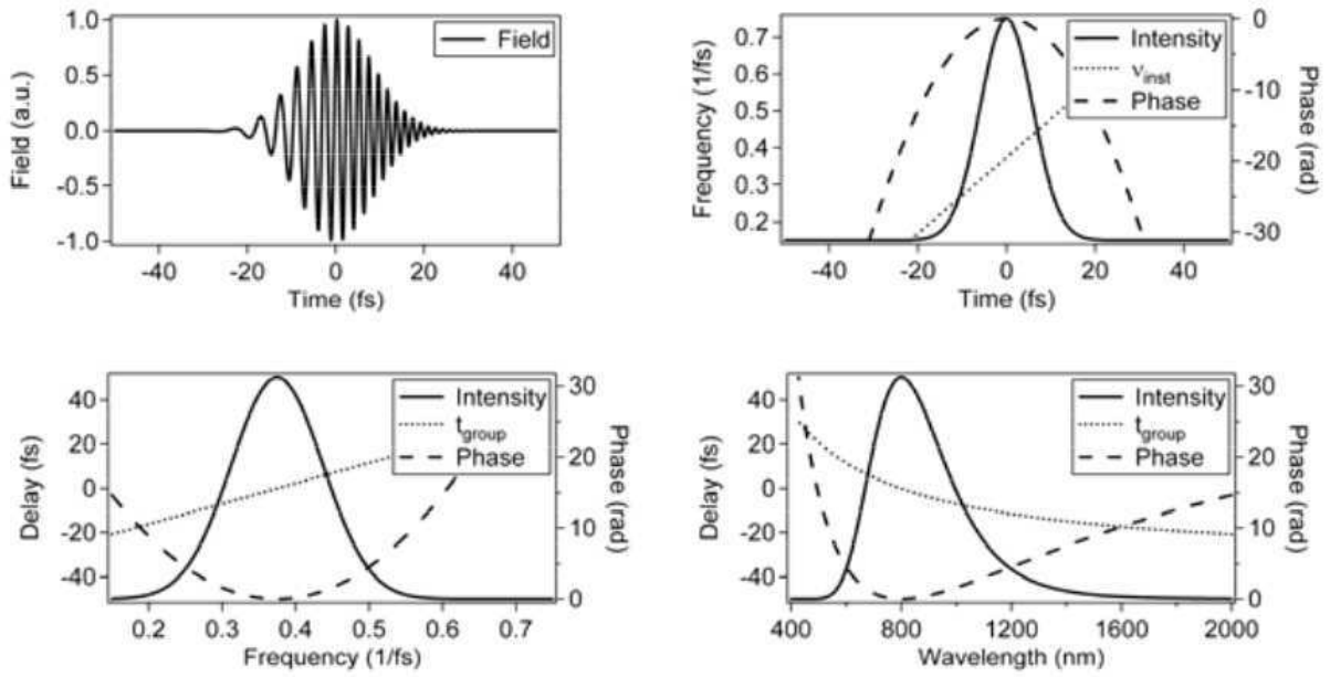
Figure I.5: Top left: temporal electric field. Top right: intensity, temporal phase, and instantaneous frequency vs. time. Bottom left: spectrum, spectral phase and group delay vs. frequency. Bottom right: spectrum, spectral phase and group delay vs. wavelength. (taken from [16])
