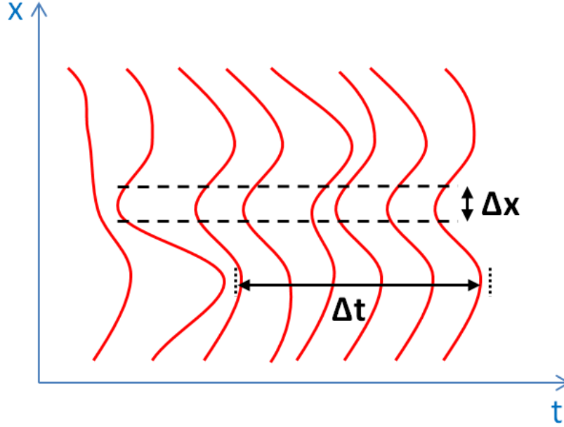
Figure I.7: Wavefront propagations with areas of spatial coherence ( \Delta x ) and temporal coherence ( \Delta t ).
