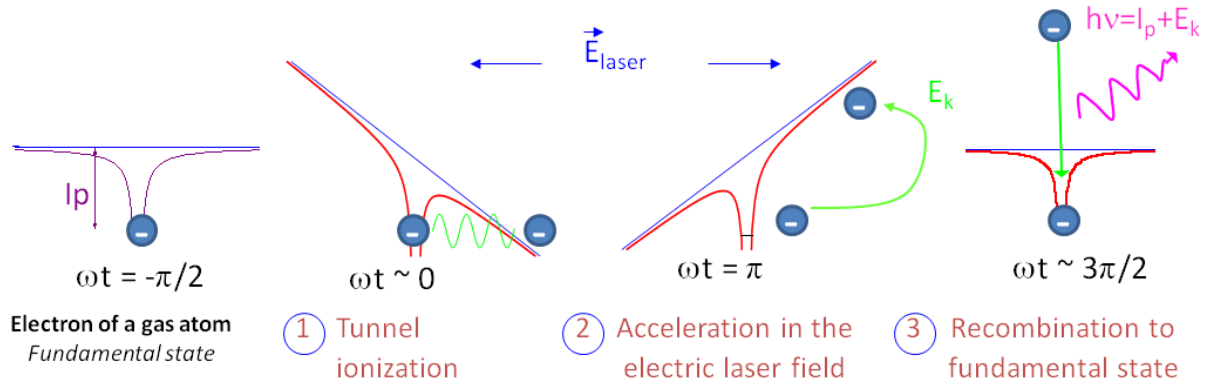
Figure I.17: Steps of the semi-classical model for the HHG.
