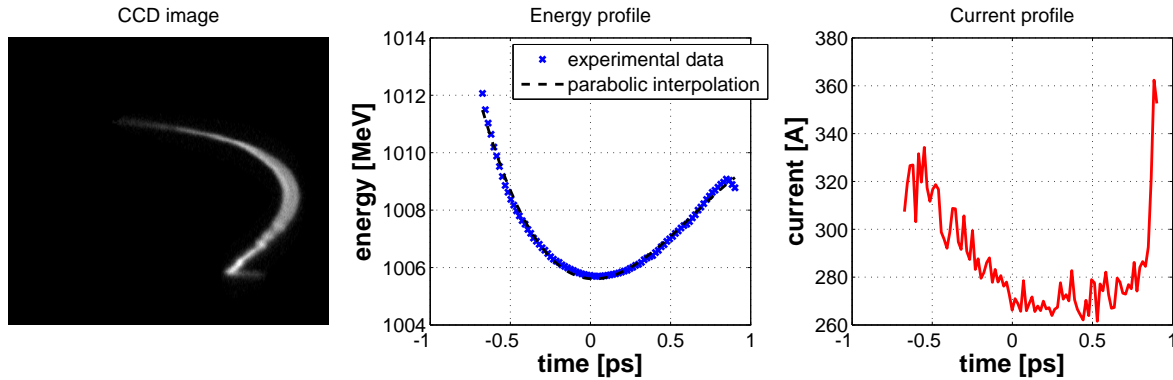
Figure IV.13: Longitudinal phase space measured at the end of the FERMI@Elettra linac for the results shown in Fig. IV.12. Left: image observed by a CCD on the YAG crystal; center: analysis of the left picture, showing the energy profile; right: analysis of the left picture, showing the current profile. Larger values of time correspond to a displacement from the tail to the head of the bunch.
