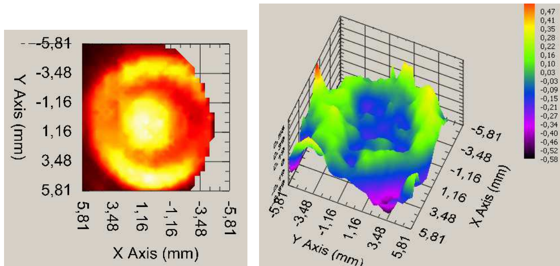
Figure II.18: Output of the Haso software: FEL spot normalized to the maximum intensity (left) and wavefront given in units of the wavelength of FEL emission (right) i.e., \lambda = 20 \text{ nm} .
