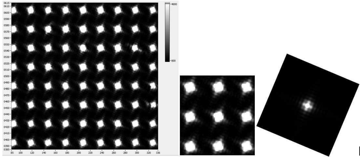
Figure II.17: Image collected on the camera of the wavefront sensor (left), zoom on a selection of pixels (center) and simulation of the expected pattern (right).
