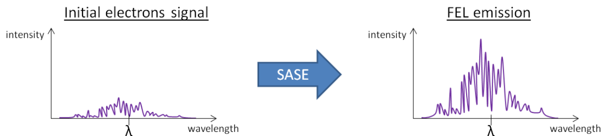
Figure I.9: Typical SASE spectrum.
