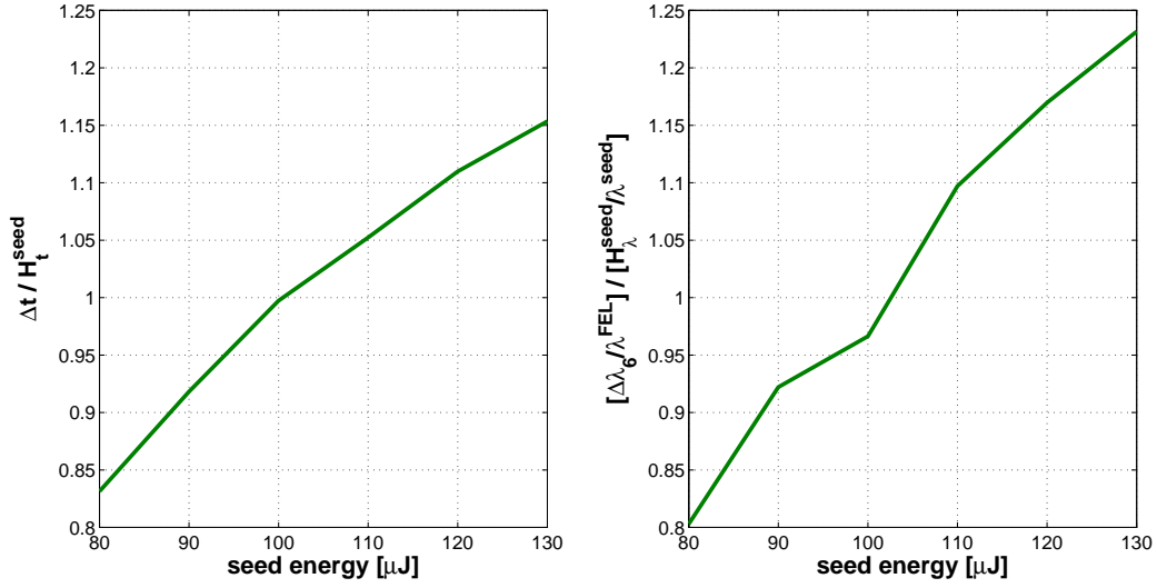
Figure IV.23: Left panel: evolution, as a function of the seed energy, of the ratio of the temporal distance between the sub-pulses vs. the FWHM duration of the seed. Right panel: evolution, as a function of the seed energy, of the ratio of the peaks spectral separation (relatively to the central wavelength of FEL emission) vs. the relative FWHM bandwidth of the seed.
