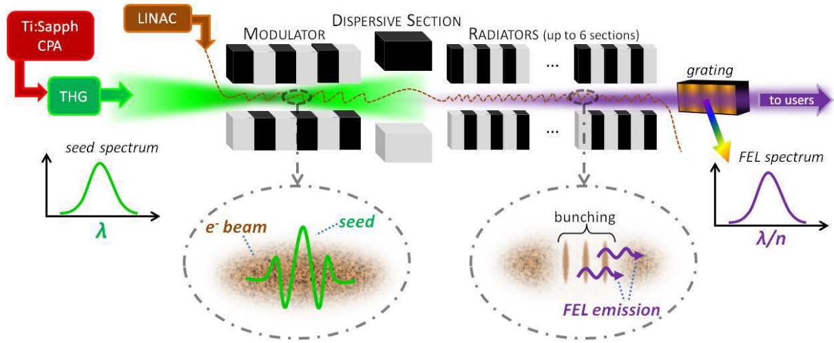
Figure I.13: Basic layout of FERMI@Elettra.
