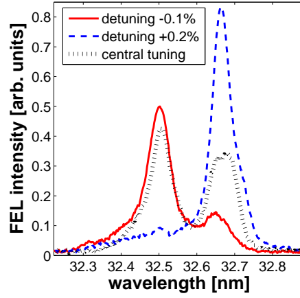
Figure IV.9: Double peak for different tuning conditions of the radiators. The radiators are tuned at the 8 th harmonic of the seed (32.6 nm). Here the seed energy per pulse is about 70 \mu\text{J} and R_{56} = 60 \mu\text{m} . The configuration of the rest of the machine was different than the one described in Table IV.1: the radiators were tuned at the 8 th harmonic of the seed (32.6 nm), R_{56} = 60 \mu\text{m} and the electron beam had following parameters: mean energy 1175 MeV, \chi_1 \approx 0 \text{ MeV/ps} , \chi_2 \approx 10 \text{ MeV/ps}^2 , FWHM duration 0.8 ps, peak current \approx 600 \text{ A} .
