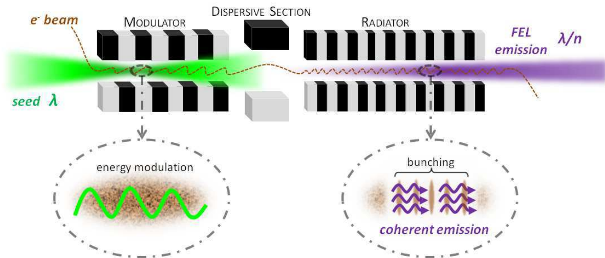
Figure I.10: Basic layout of a CHG FEL.
