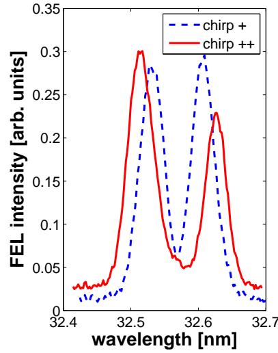
Figure IV.11: Double peak for two different chirp values of the seed (b), corresponding to the standard positive chirp ("chirp +", \sigma_\lambda \approx 0.45 nm and \sigma_t \approx 90 fs, with a seed energy of \approx 70 \mu J) and a stronger chirp ("chirp ++", \sigma_\lambda \approx 0.5 nm and \sigma_t \approx 160 fs, with a seed energy of \approx 75 \mu J) induced by adding a piece of \text{CaF}_2 of 5-cm thickness. The radiators were tuned at the 8 th harmonic of the seed (32.6 nm), R_{56} = 80 \mu m and the electron beam is similar the one shown in the top half of Fig. III.9.
