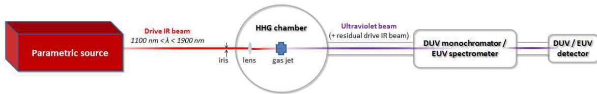
Figure V.1: Layout of the experiment.
