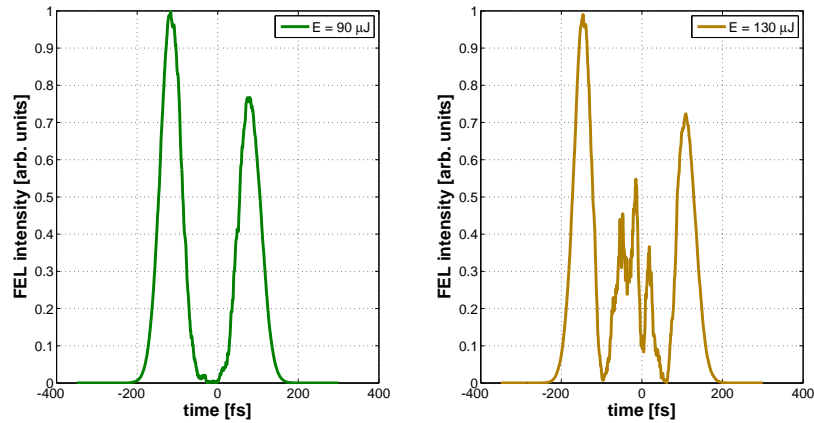
Figure IV.31: Temporal profile of the FEL emission given by simulations with a flat electrons' energy profile, for an energy per pulse of the seed of 90 \mu J and of 130 \mu J .
