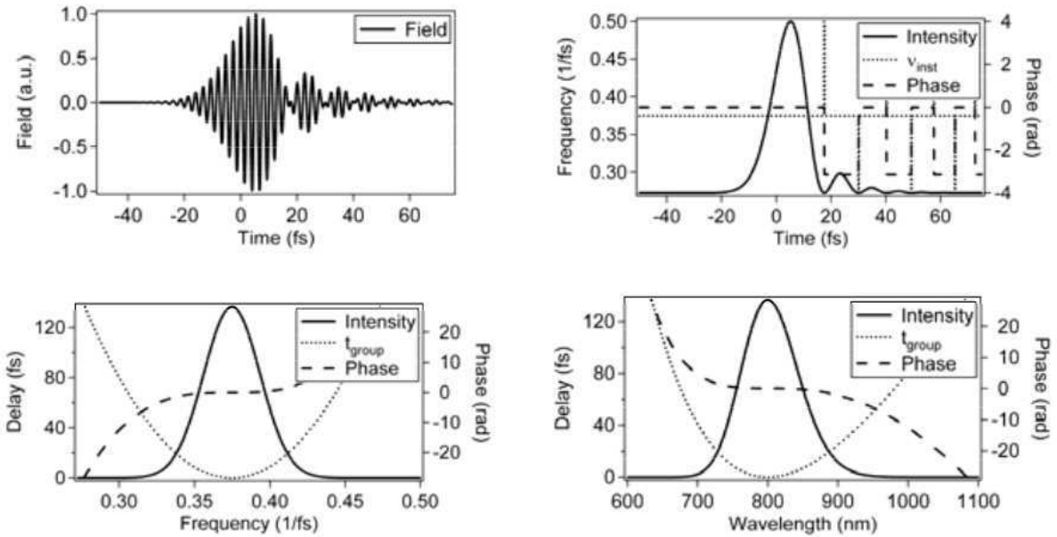
Figure I.6: Top left: temporal electric field. Top right: intensity, temporal phase, and instantaneous frequency vs. time. Bottom left: spectrum, spectral phase and group delay vs. frequency. Bottom right: spectrum, spectral phase and group delay vs. wavelength. (taken from [16])
