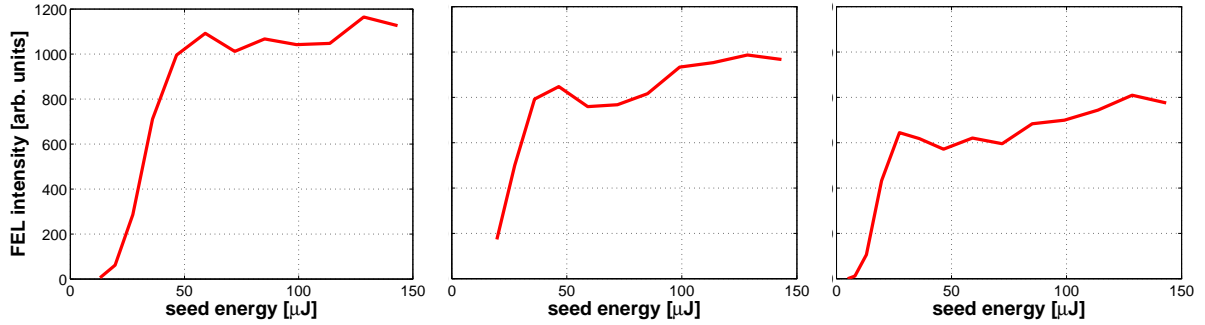
Figure IV.8: Overall intensity of the FEL radiation as a function of the seed energy for different values of R_{56} : 23.4 \mu\text{m} (left), 29.6 \mu\text{m} (middle) and 36.6 \mu\text{m} (right).
