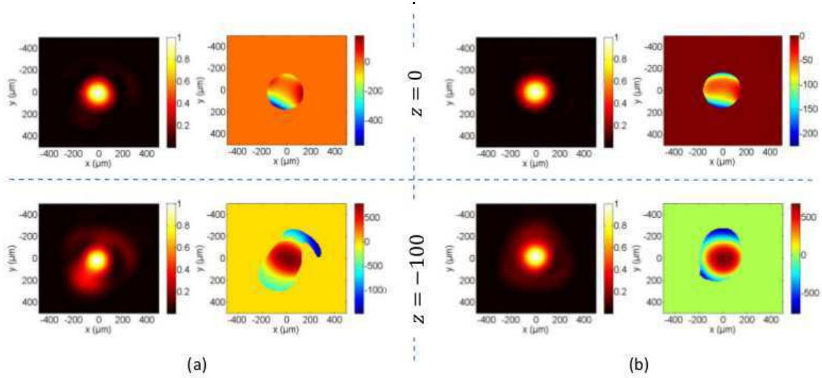
Figure II.32: Simulations of intensity and wavefront of the IR beam at z = -100 mm and z = 0 mm for the non-filtered (a) and filtered (b) beam with iris 3 closed at a diameter of 22 mm. In each quadrant, the left picture corresponds to the intensity pattern and the right one to the wavefront. The wavefront is displayed only where the intensity is higher than \frac{1}{e^2} of the maximum intensity. [Courtesy of D. Gauthier]
