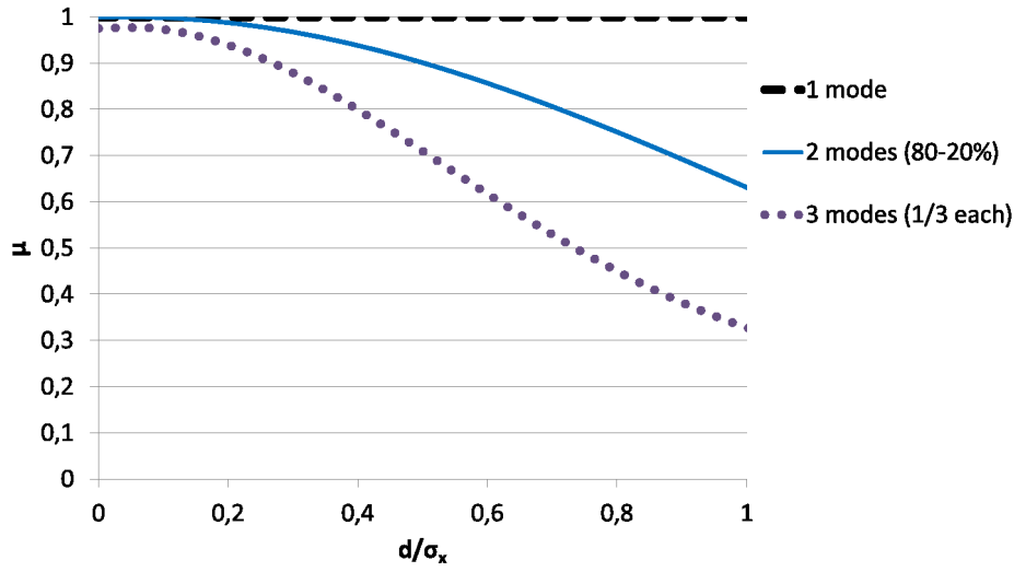
Figure II.15: Degree of coherence as a function of the relative slits' separation for a GSM beam whose cross-spectral density is described with only \Psi_0 (dashed line), with 80% of \Psi_0 and 20% of \Psi_1 (full line) and the sum of one third of \Psi_0 , one third of \Psi_1 and one third of \Psi_2 .
