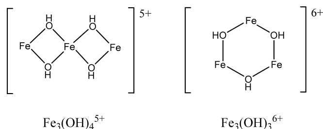
Scheme 4.3 Proposed molecular structures for the \text{Fe(III)} trimer.
