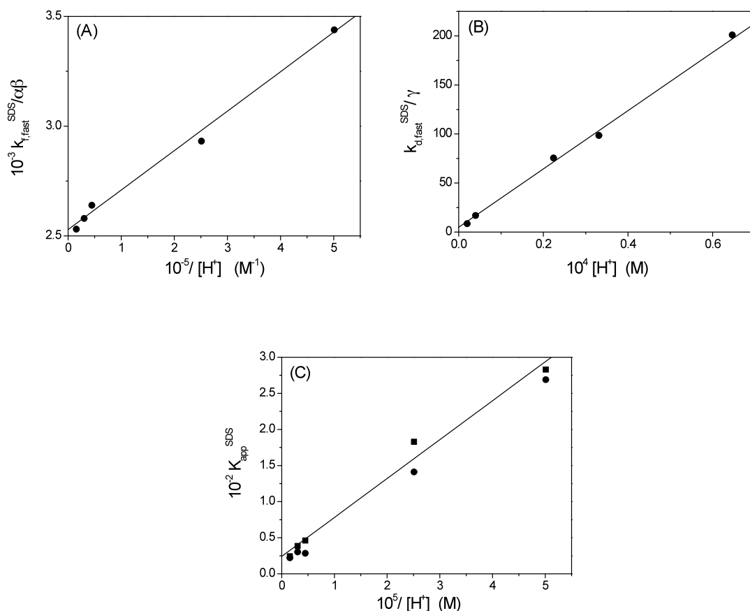
Figure 3.11 Kinetic behavior for the fast effect of the Ni(II)/SHA reaction in SDS 3.5 \times 10^{-2} \text{ M} , I = 0.2 \text{ M} , T = 298 \text{ K} . (A) Dependence of the forward rate constant, k_{f,fast}^S , on hydrogen ion concentration. (B) Dependence of the reverse rate constant, k_{d,fast}^S , on hydrogen ion concentration. (C) Dependence of K_{app}^S on hydrogen concentration, evaluated from kinetic experiments, as k_{f,fast}^S/k_{d,fast}^S (■) and from spectrophotometric titrations (●).
