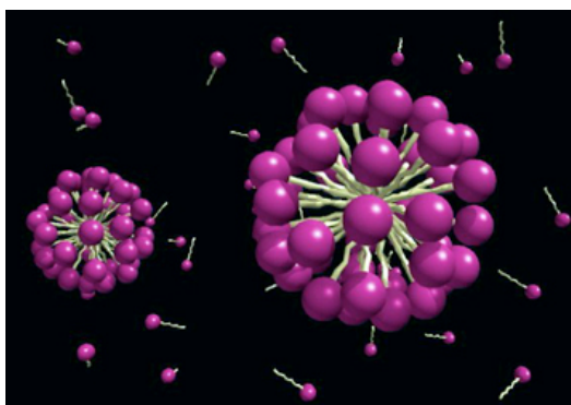
Figure 3.2 Structure of a spherical micelle.
