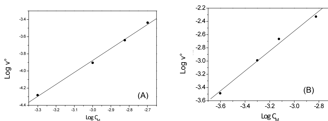
Figure 5.8 Dependence of the initial rate on metal ion concentration for the \text{Cu(II)}/(S)\text{-}\alpha\text{-Alaha} system. C_L = 5.0 \times 10^{-4} M, \text{pH} = 4.75 , \lambda = 340\text{nm} , T = 298 K; (A) I = 0.1 M, (B) I = 0.9 M.
