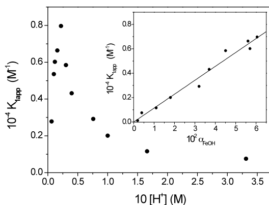
Figure 4.8 Dependence of the apparent binding constant, K_{\text{lapp}} , for the Fe(III)/BHA system on [\text{H}^+] at I = 1\text{ M} ( \text{HClO}_4/\text{NaClO}_4 ) and T = 298\text{ K} . Inset: dependence of K_{\text{lapp}} on \alpha_{\text{FeOH}} , the molar fraction of \text{FeOH}^{2+} ion.
