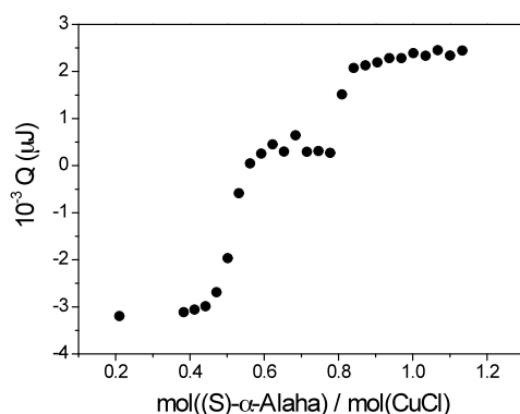
Figure 5.14 ITC curve for the system Cu(II)/(S)- \alpha -Alaha. \text{pH} = 4.5 , I = 0.1 \text{ M} , T = 298 \text{ K} .
