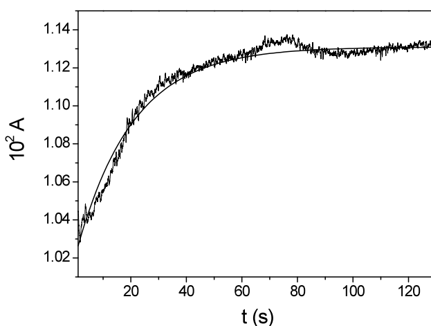
Figure 5.19 Monophasic kinetic curve for the reaction of 12-MC-4 with La(III) and excess Cu(II); C_{La} = 1.23 \times 10^{-1} M , C_{Cu} = 1 \times 10^{-2} M ; I = 0.1 M ; pH = 4.5 ; \lambda = 580 nm ; T = 298 K .
