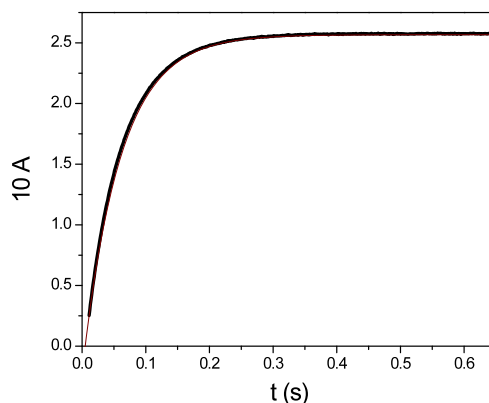
Figure 4.11 Stopped-flow traces recorded at \lambda = 520 nm upon mixing BHA 2.5 \times 10^{-4} M and Fe(ClO_4)_3 9.0 \times 10^{-3} M at I = 1 M ( HClO_4/NaClO_4 ) and T = 298 K.
