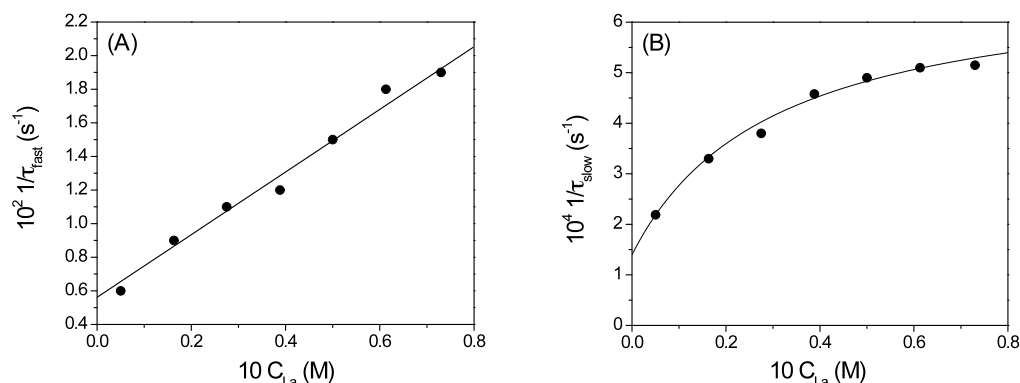
Figure 5.17 Time constant dependence on La(III) concentration for the fast and slow kinetic effect observed for the 12-MC-4/La(III) reaction. \text{pH} = 4.5 , I = 0.1 \text{ M} ; T = 298 \text{ K} .
