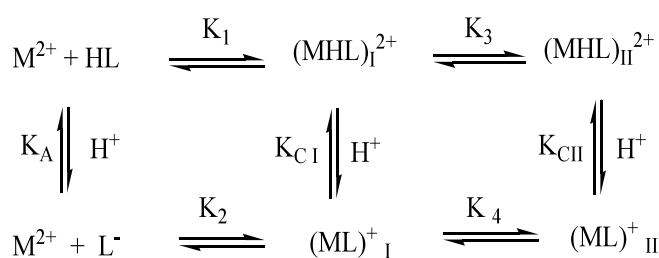
Scheme 3.2 Reactive scheme for the Ni(II)/SHA system, involving the slow effect, in SDS micellar solution.
