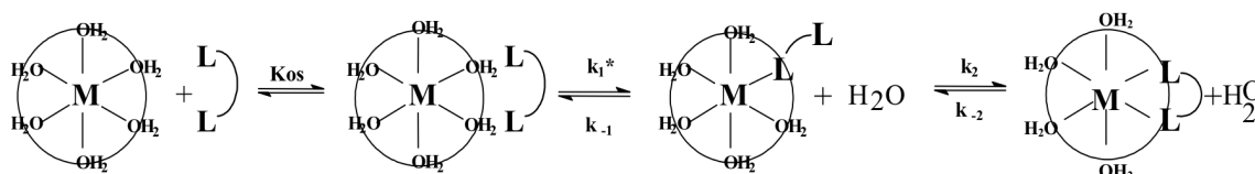
Scheme 1.14 Eigen-Wilkins mechanism.
