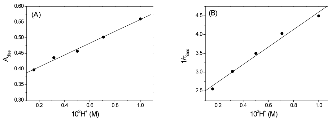
Figure 5.11 (A) Amplitudes, A_{\text{diss}} , and (B) rate constants, 1/\tau_{\text{diss}} , dependence on [H^+] for the reverse reaction of \text{Cu(II)}/(\text{S}) - \alpha -Alaha 12-MC-4 self assembly; I = 0.1 \text{ M} , \lambda = 340 \text{ nm} , T = 298 \text{ K} .
