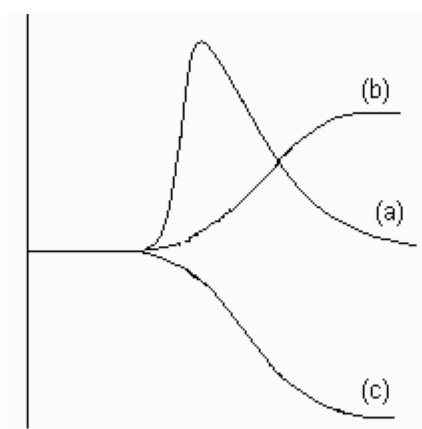
Figure 3.4 Effect of surfactants on reaction rates. Curves (a) and (b) represent micellar catalysis while curve (c) is a typical example of micellar inhibition.
