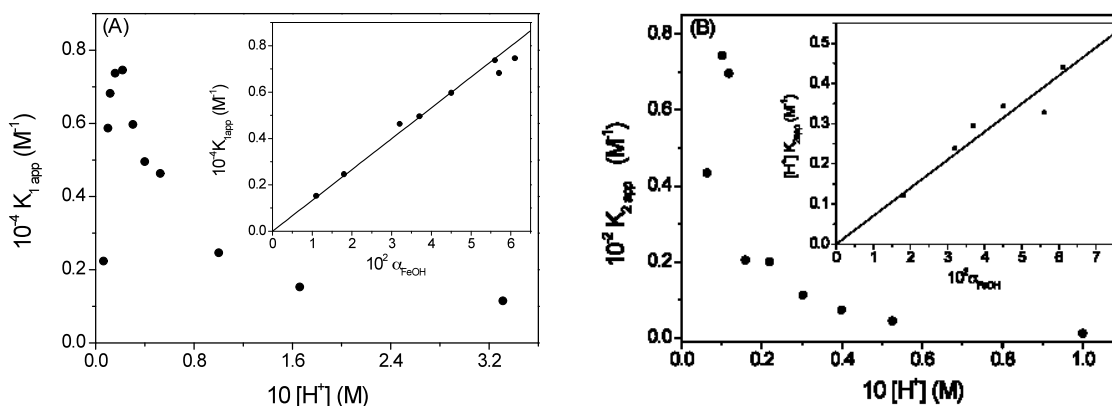
Figure 4.10 Dependence of the apparent binding constants, K_{1app} and K_{2app} , for the Fe(III)/SHA system on [H^+] at I = 1 M ( HClO_4/NaClO_4 ) and T = 298 K ; (A) plot of K_{1app} vs [H^+] , inset: dependence of K_{1app} on \alpha_{FeOH} . (B) plot of K_{2app} vs [H^+] , inset: dependence of [H^+] \times K_{2app} on \alpha_{FeOH} .
