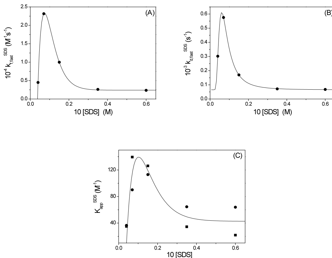
Figure 3.12 Micellar catalysis for the system Ni(II)/SHA at pH = 4.65 , I = 0.2 M, T = 298 K. (A) Dependence of the forward rate constant, k_{f,fast}^S , on the SDS concentration. (B) Dependence of the back rate constant, k_{d,fast}^S , on the SDS concentration. (C) Dependence of the equilibrium constant obtained from spectrophotometric titrations (■) and expressed as k_{f,fast}^S / k_{d,fast}^S (●) on the SDS concentration.
