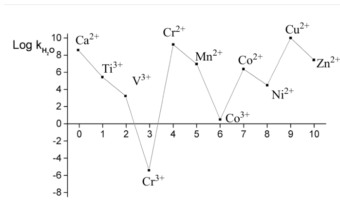
Figure 1.3 Dependence of the rate constant of the \text{H}_2\text{O} exchange process on the number of d electrons in different cations (Helm and Merbach, 1999).
