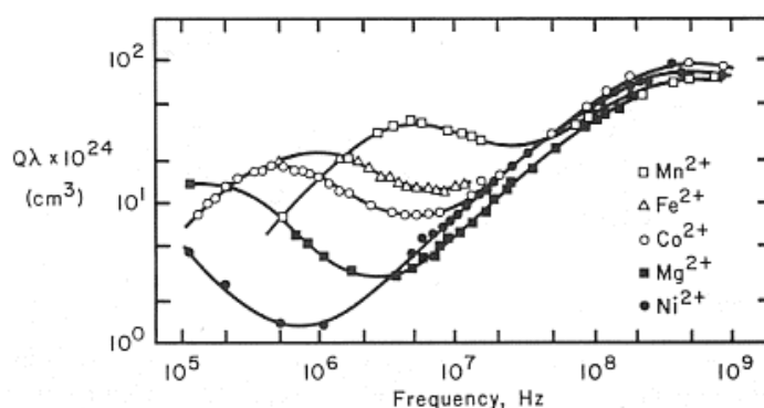
Figure 1.2 Ultrasound spectrum of some divalent metal sulphates (0.5 M) in aqueous solution.
