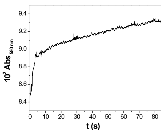
Figure 5.16 Biphasic kinetic curve for the reaction of 12-MC-4 with La(III). C_{La} = 3.9 \times 10^{-2} M; C_{Cu} = C_L = 3 \times 10^{-3} M; I = 0.1 M; pH = 4.75 ; \lambda = 580 nm; T = 298 K.
