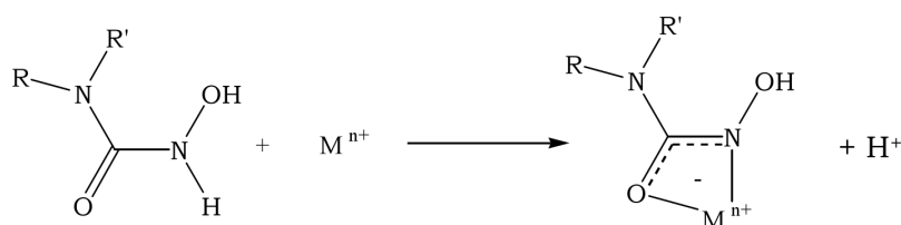
Scheme 1.12 Metal ion ( \text{M}^{n+} ) {N,O} coordination by a generic aminohydroxamic acid.
