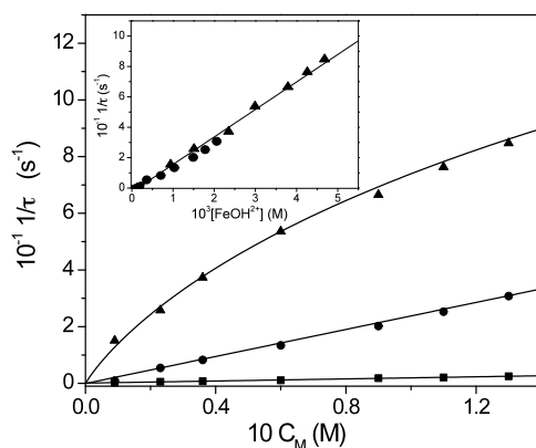
Figure 4.12 Dependence of 1/\tau on C_M at different [H^+] values for the Fe(III)/BHA system at I = 1 M ( HClO_4/NaClO_4 ) and T = 298 K; [BHA] = 2.5 \times 10^{-4} M, [H^+] = 1 M ■, 0.1 M ●, 0.01 M ▲. The inset represents the dependence of 1/\tau on [FeOH^{2+}] , calculated at all acidities by the relationship [FeOH^{2+}] = \alpha_{FeOH} C_M .
