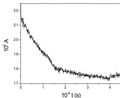
Figure 4.6 Kinetic trace recorded by spectrophotometric measurements for Fe(III). C_M = 2 \times 10^{-4} \text{ M} , \lambda = 532 \text{ nm} , [H^+] = 0.1 \text{ M} , I = 1 \text{ M} ( \text{HClO}_4/\text{NaClO}_4 ) and T = 298 \text{ K} .
