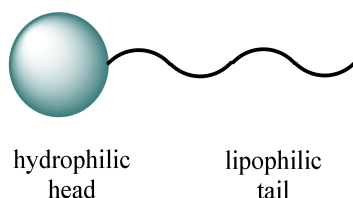
Figure 3.1 Structure of a generic surfactant
