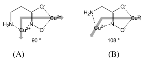
Scheme 5.4 Structures of the conceptual building blocks of metallacrowns: 12-MC-4 (A) and 15-MC-5 (B).
