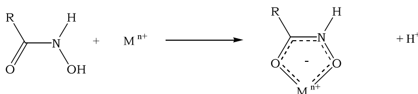
Scheme 1.11 Metal ion ( \text{M}^{n+} ) {O,O} coordination by a generic hydroxamic acid.
