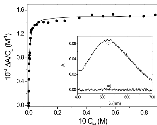
Figure 4.7 Binding isotherm for the interaction of Fe(III) with BHA at I = 1\text{ M} ( \text{HClO}_4/\text{NaClO}_4 ) and T = 298\text{ K} . Inset shows the spectral change induced by complex formation; [\text{BHA}] = 2.5 \times 10^{-4}\text{ M} , [\text{H}^+] = 0.1\text{ M} , inset: (a) C_M = 0\text{ M} , (b) C_M = 1.7 \times 10^{-1}\text{ M} .
