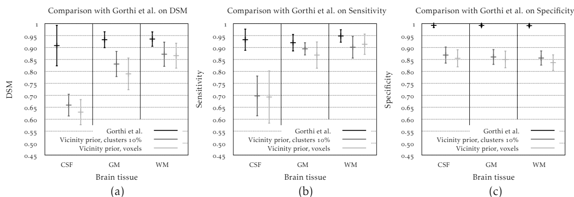
Figure 5.9: Quantitative comparison of brain tissue segmentation with [GTC 11 ] on the original BrainWeb simulated MRI dataset.
