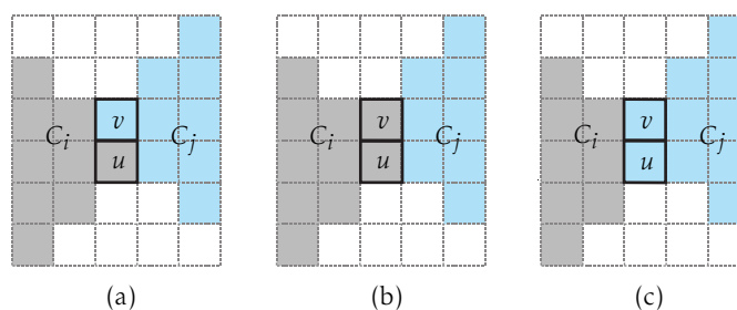
Figure 4.2: The three voxel assignment possibilities to a pair of clusters, in gray and blue, during energy minimization. (a) Initial configuration, (b) C_i grows; C_i \leftarrow u, v , and (c) C_j grows; C_j \leftarrow u, v .
