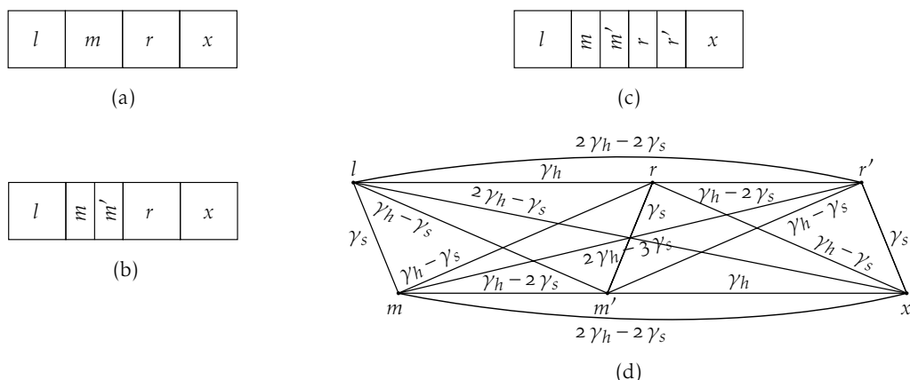
Figure 3.3: (a) 4-label structure adjacency model, (b) the model after shadowing the label m and (c) after shadowing the label r' , (d) geometrical representation of the extended adjacency prior on the new model. Note that line segment lengths are set for illustration clarity and do not precisely correspond to indicated quantities. Segments \bar{lr}' and \bar{m}\bar{x} are drawn curved for the same purpose.
