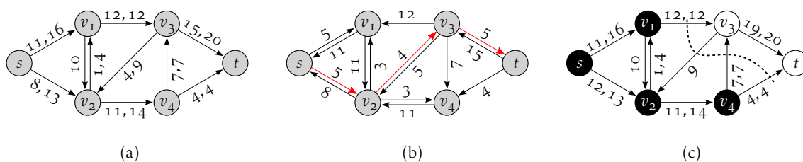
Figure 2.1: Illustration of concepts of flow networks after [CLRS09]. (a) A flow network with |f| = 19 indicating the flow and the capacity of each edge, negative flows are not shown, (b) the residual network induced by the previous flow with an augmenting path of capacity c_f(p) = 4 highlighted, (c) the flow network after augmentation through the highlighted path producing the indicated minimum cut with capacity c(S, T) = 23 .
